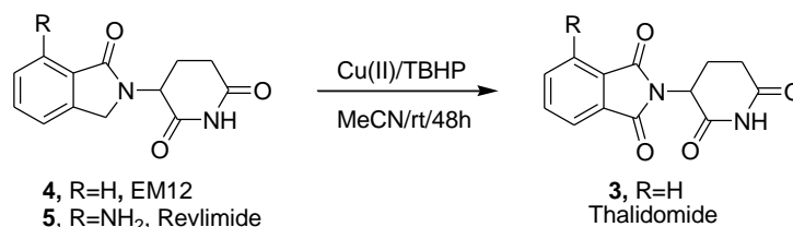
Scheme 2. Oxidation of EM12 4 to thalidomide 3 .
