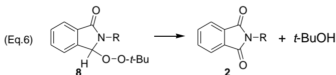
Scheme 3. Plausible mechanistic steps for the Cu(II)/TBHP-mediated isoindolinone to phthalimide oxidation
