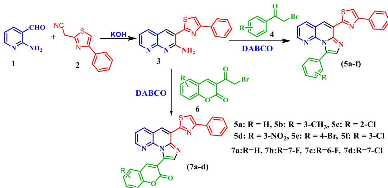
Scheme 1 Synthesis of novel fused naphthyridine ( 5a-f/7a-d ) scaffolds.
