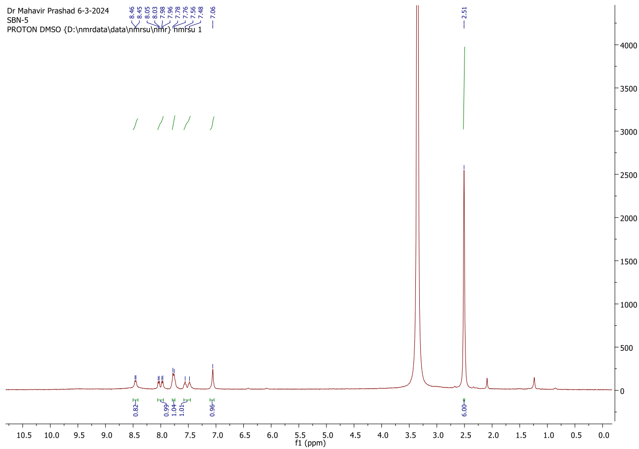
1 H NMR of 5g
