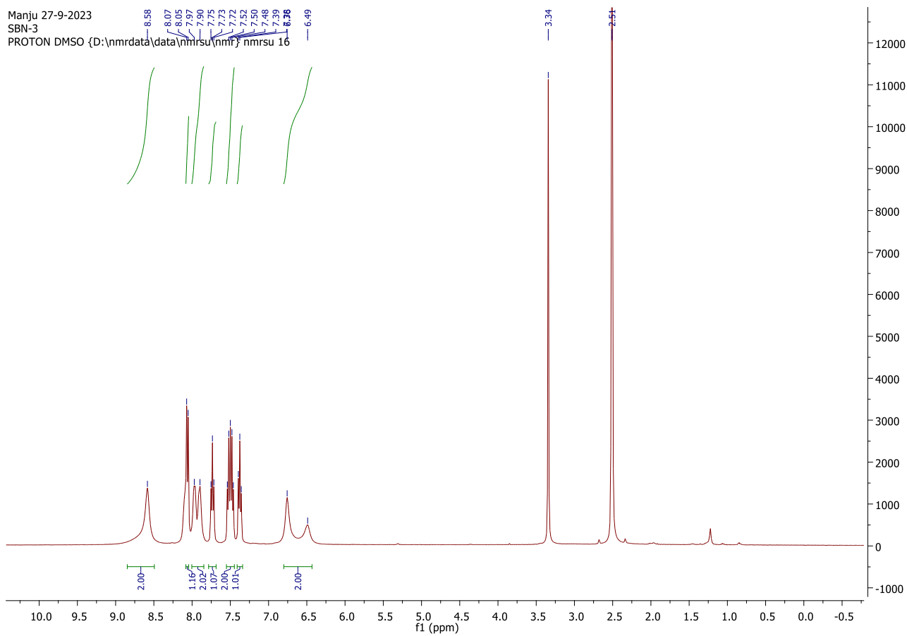
^1\text{H} NMR of 5c
