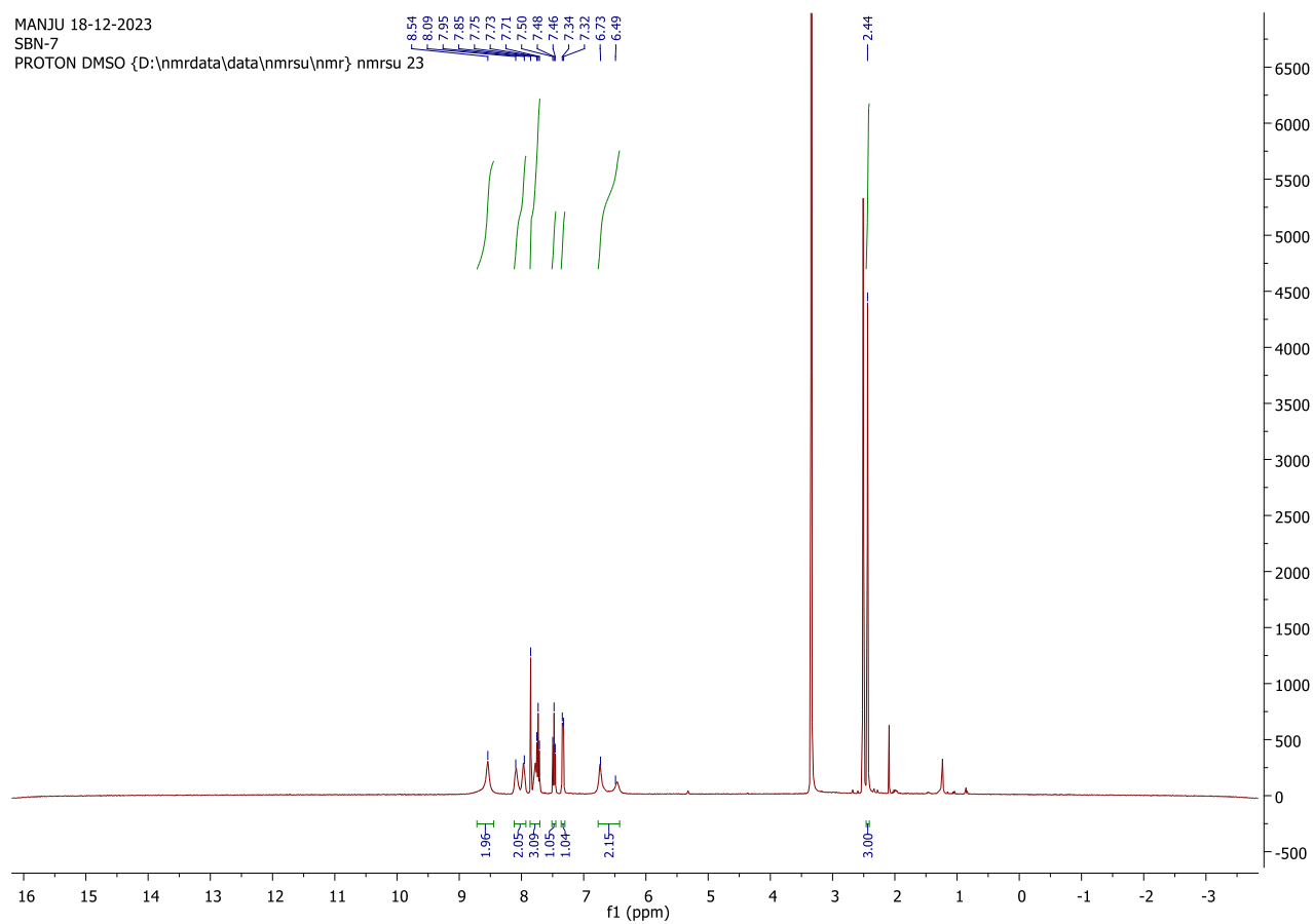
^1\text{H} NMR of 5d
