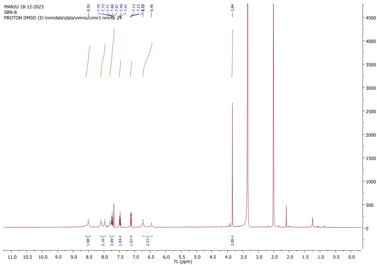
^1\text{H} NMR of 5f
