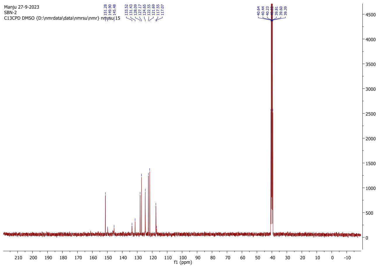
13 C NMR of 5b
