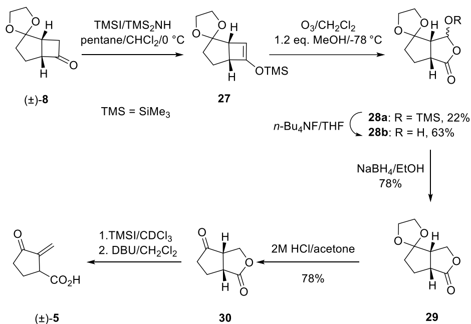
Scheme 4. The synthesis of ( \pm )-sarkomycin ( 5 ) from the fused cyclobutanone ( \pm )- 8 .
