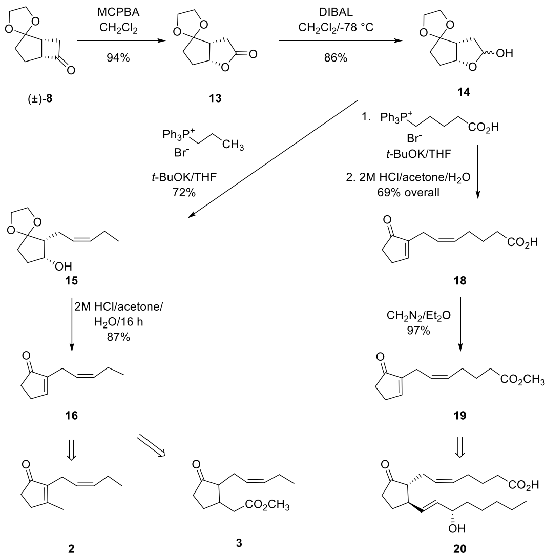
Scheme 2. Elaboration of (±)-8 to 16 , a known synthetic precursor to cis -jasmonone ( 2 ) and (±) -methyl jasmonate ( 3 ), and 19 , an established precursor to racemic 11-deoxy-PGE 2 ( 20 ). 4,16
