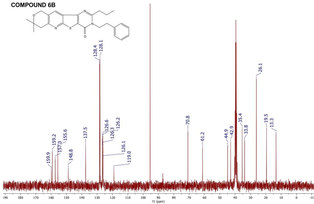
COMPOUND 6B
