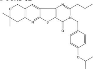
COMPOUND 6L
