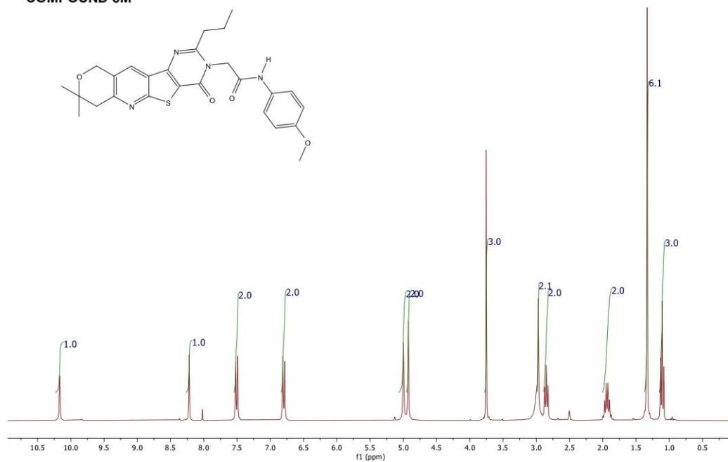
COMPOUND 6M
