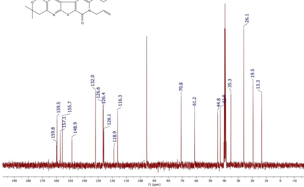
COMPOUND 6C
