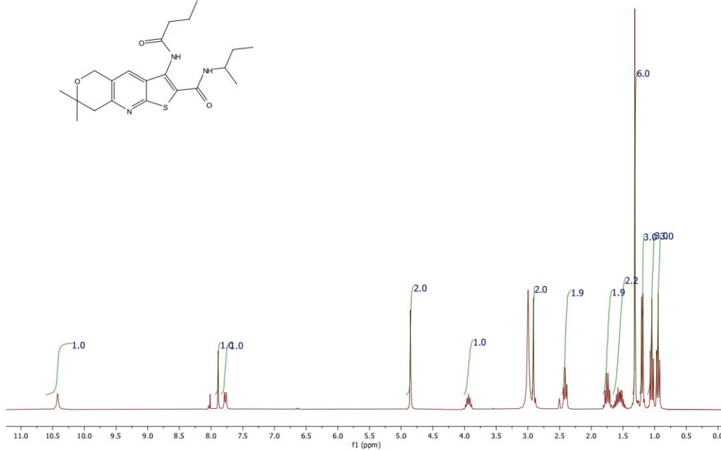
COMPOUND 3C
