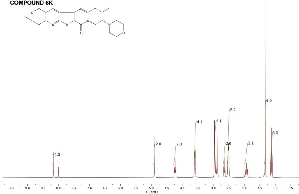
COMPOUND 6K
