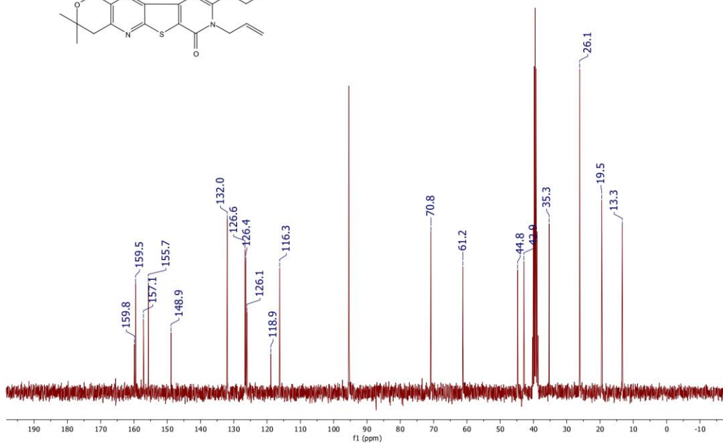
COMPOUND 4C
