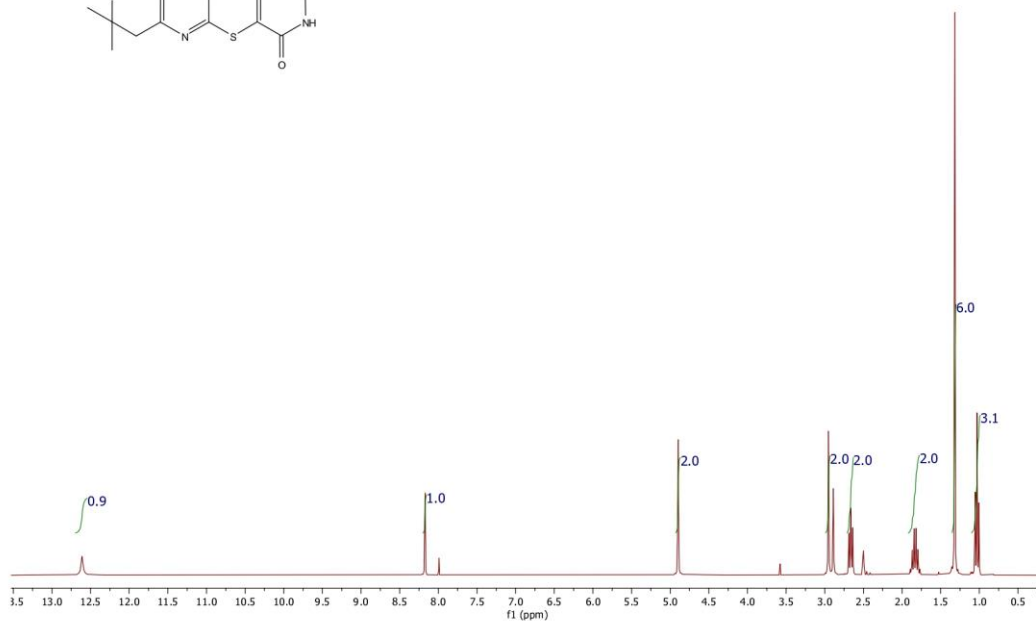
COMPOUND 5
