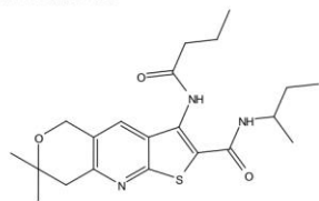
COMPOUND 3C
