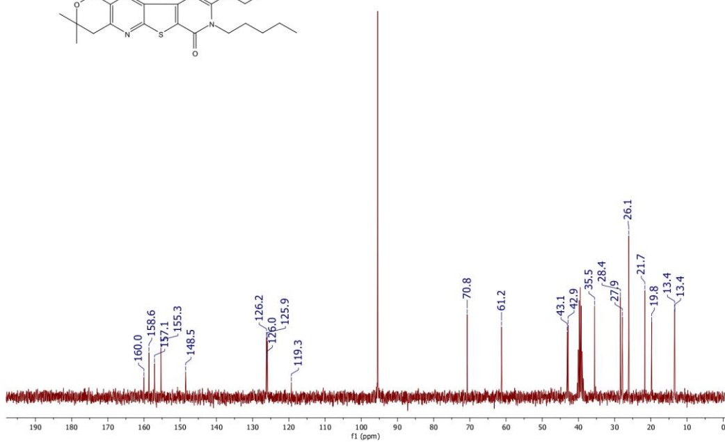
COMPOUND 6E
