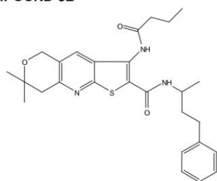
COMPOUND 3B
