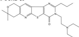
COMPOUND 6J
