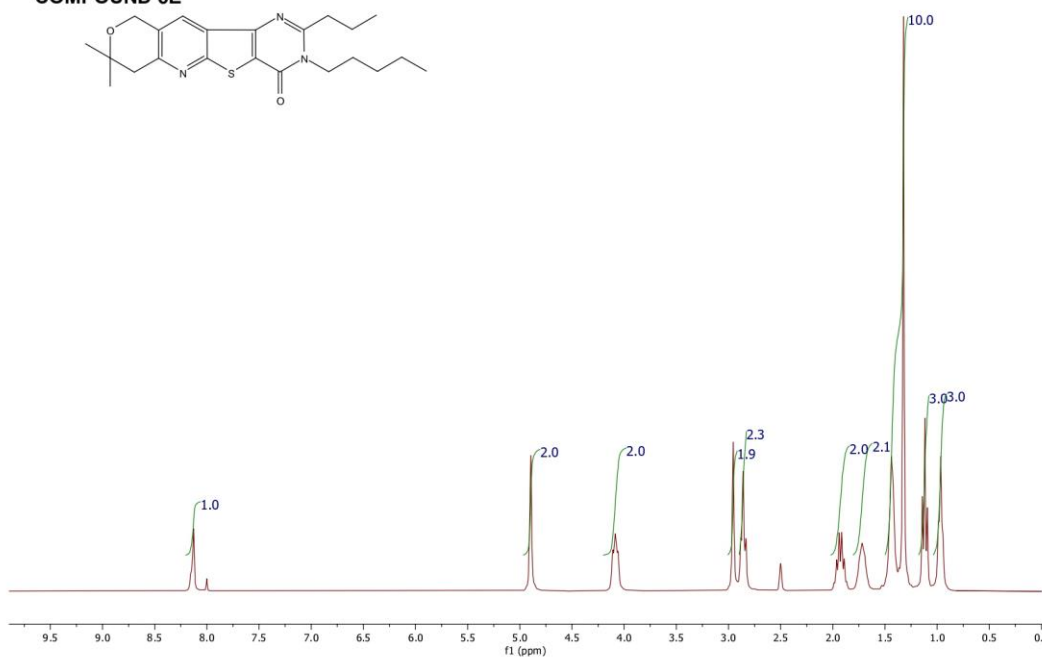
COMPOUND 6E
