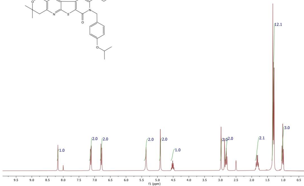
COMPOUND 6L
