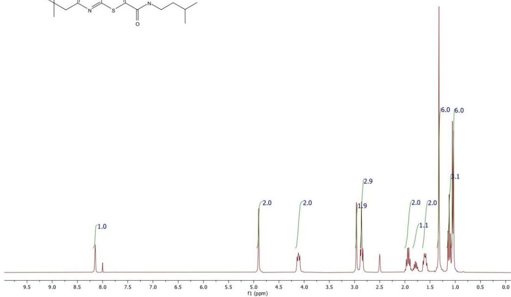
COMPOUND 6F
