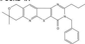
COMPOUND 4A
