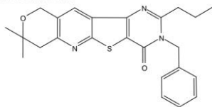
COMPOUND 6A
