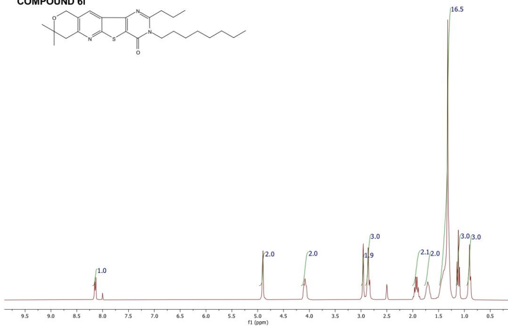
COMPOUND 6i
