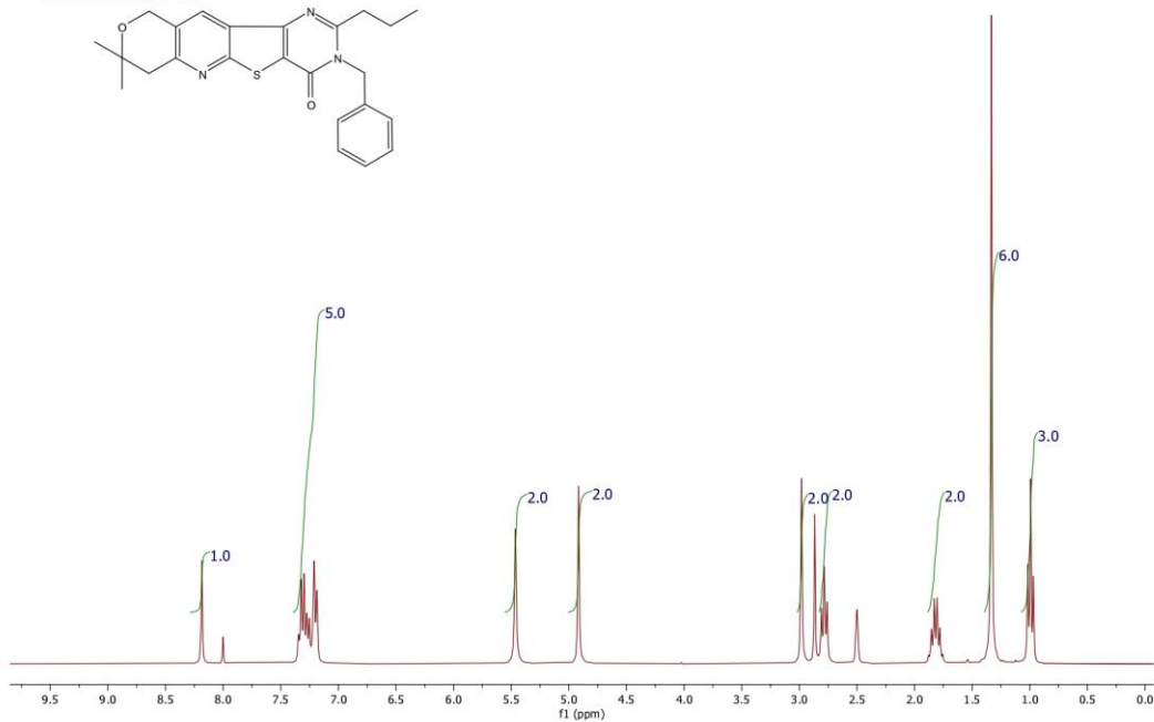
COMPOUND 4A
