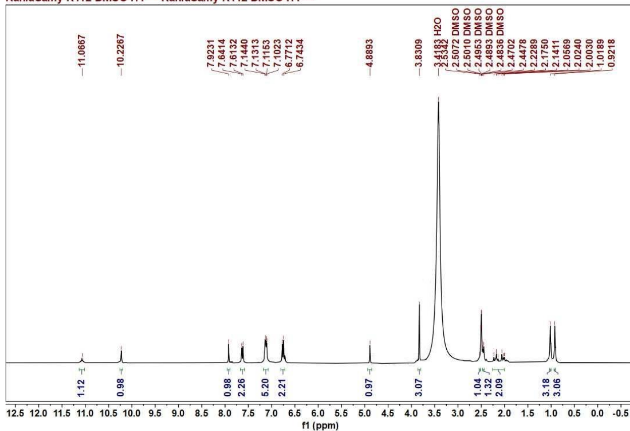
Figure 8. The 1 H NMR spectrum of compound 13b
