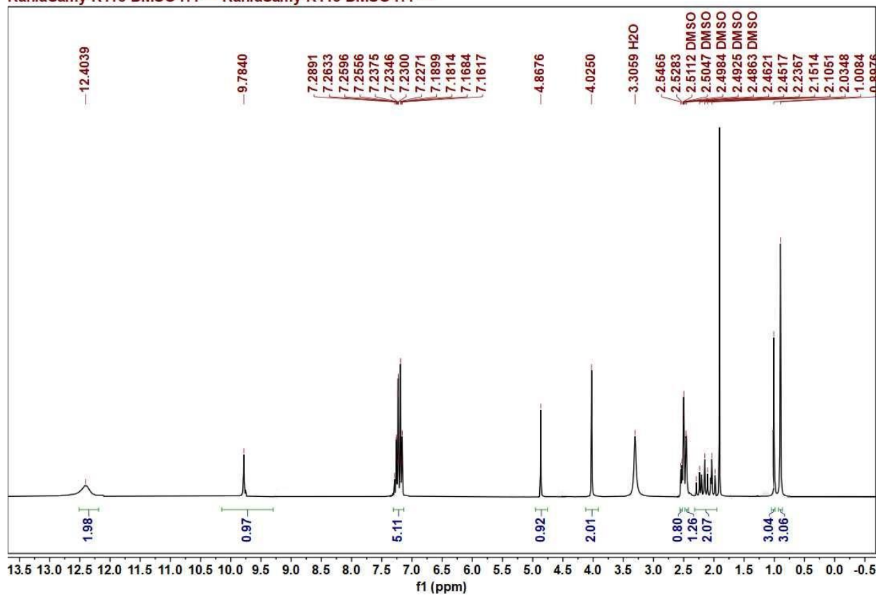
Figure 14. The 1 H NMR spectrum of compound 15b
