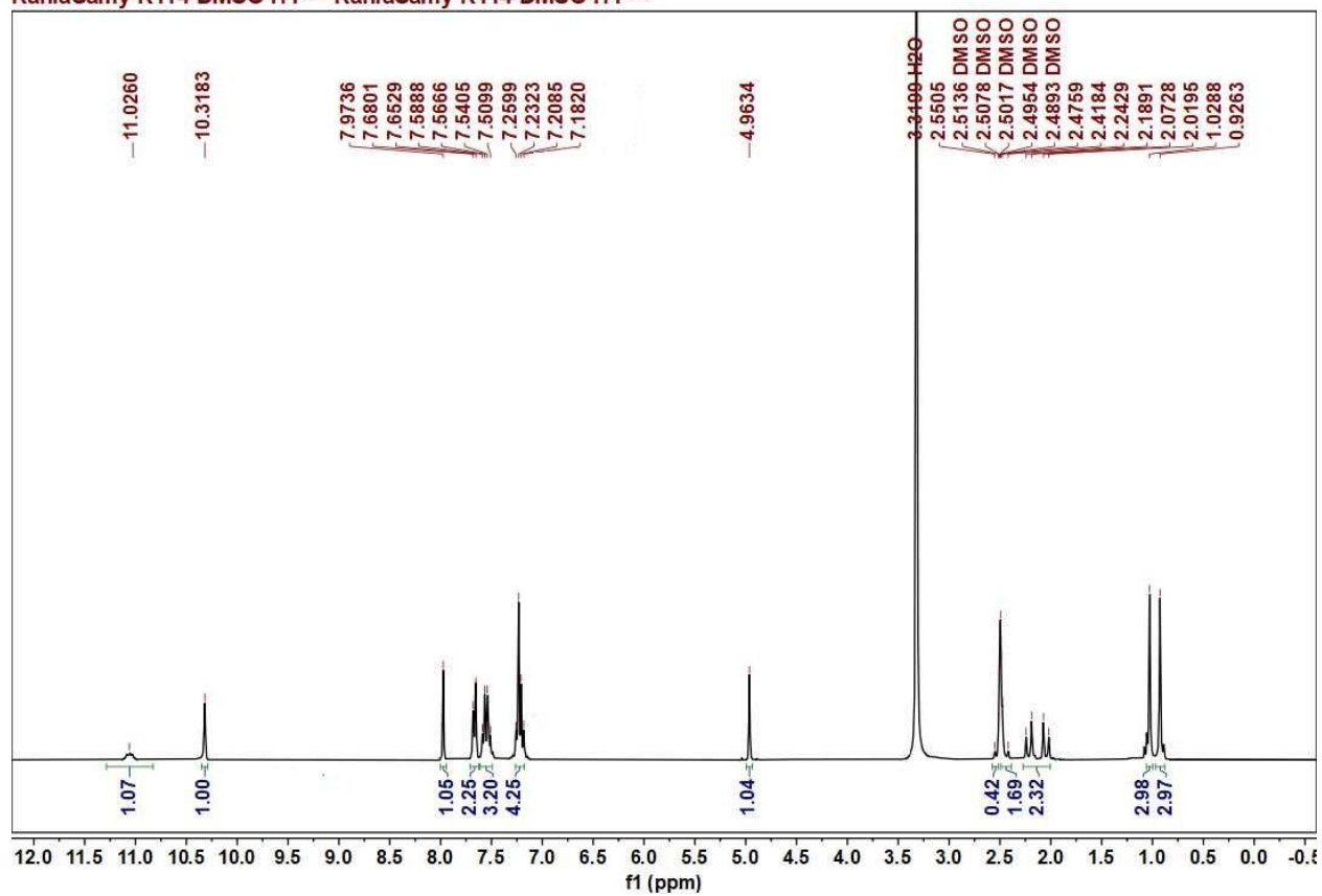
Figure 12. The 1 H NMR spectrum of compound 13e
