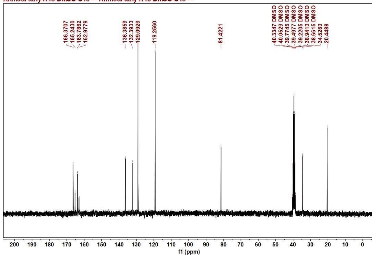
Figure 3. The 13 C NMR spectrum of compound 9b
