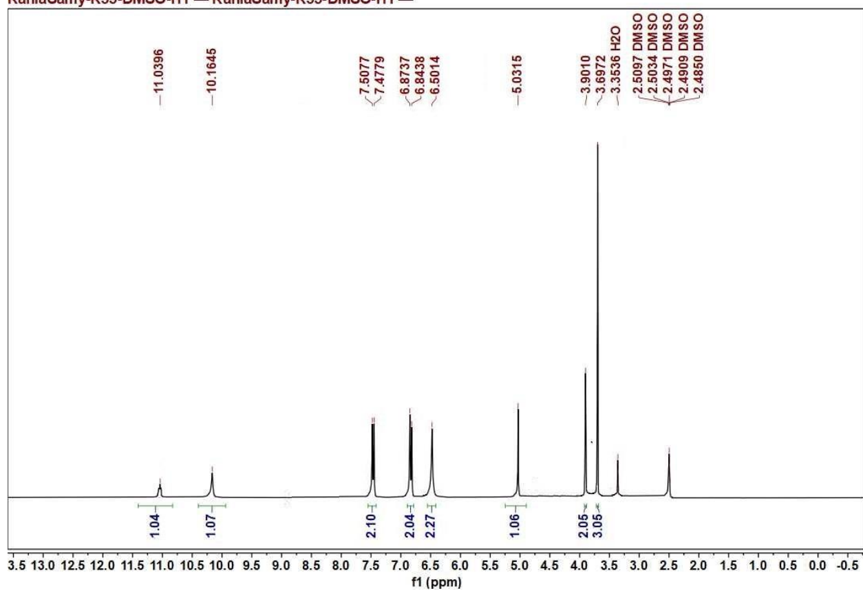
Figure 4. The 1 H NMR spectrum of compound 9c
