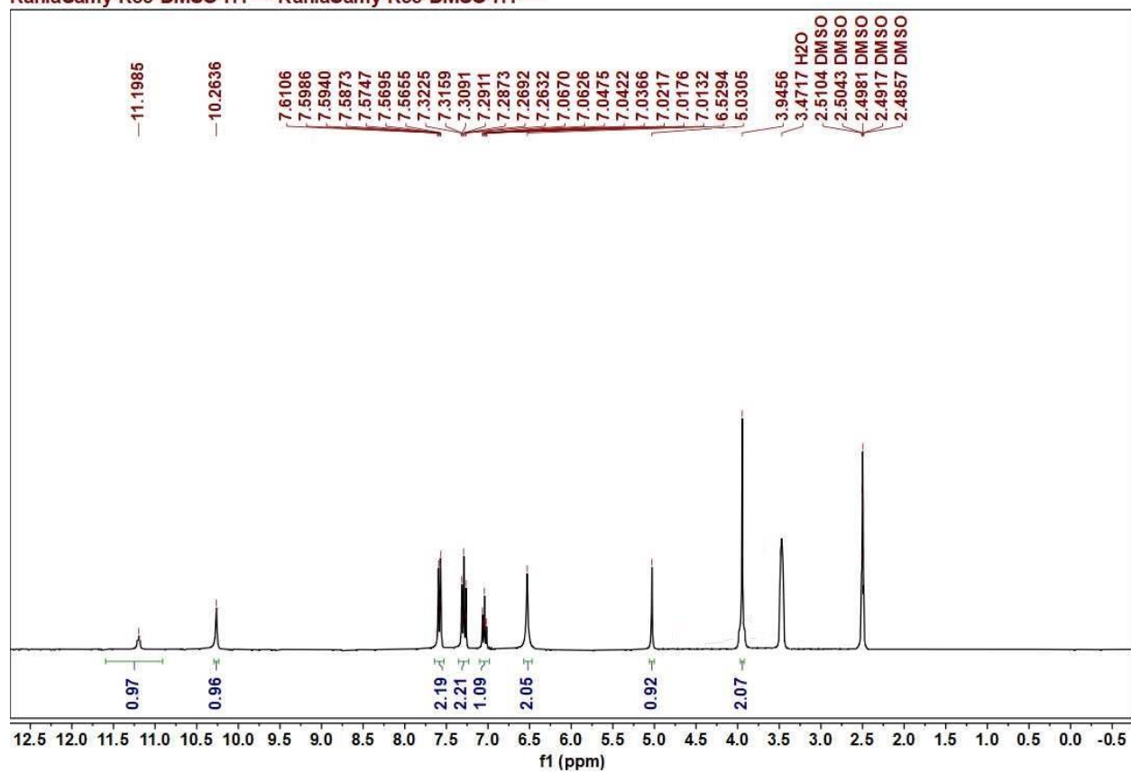
Figure 1. The 1 H NMR spectrum of compound 9a
