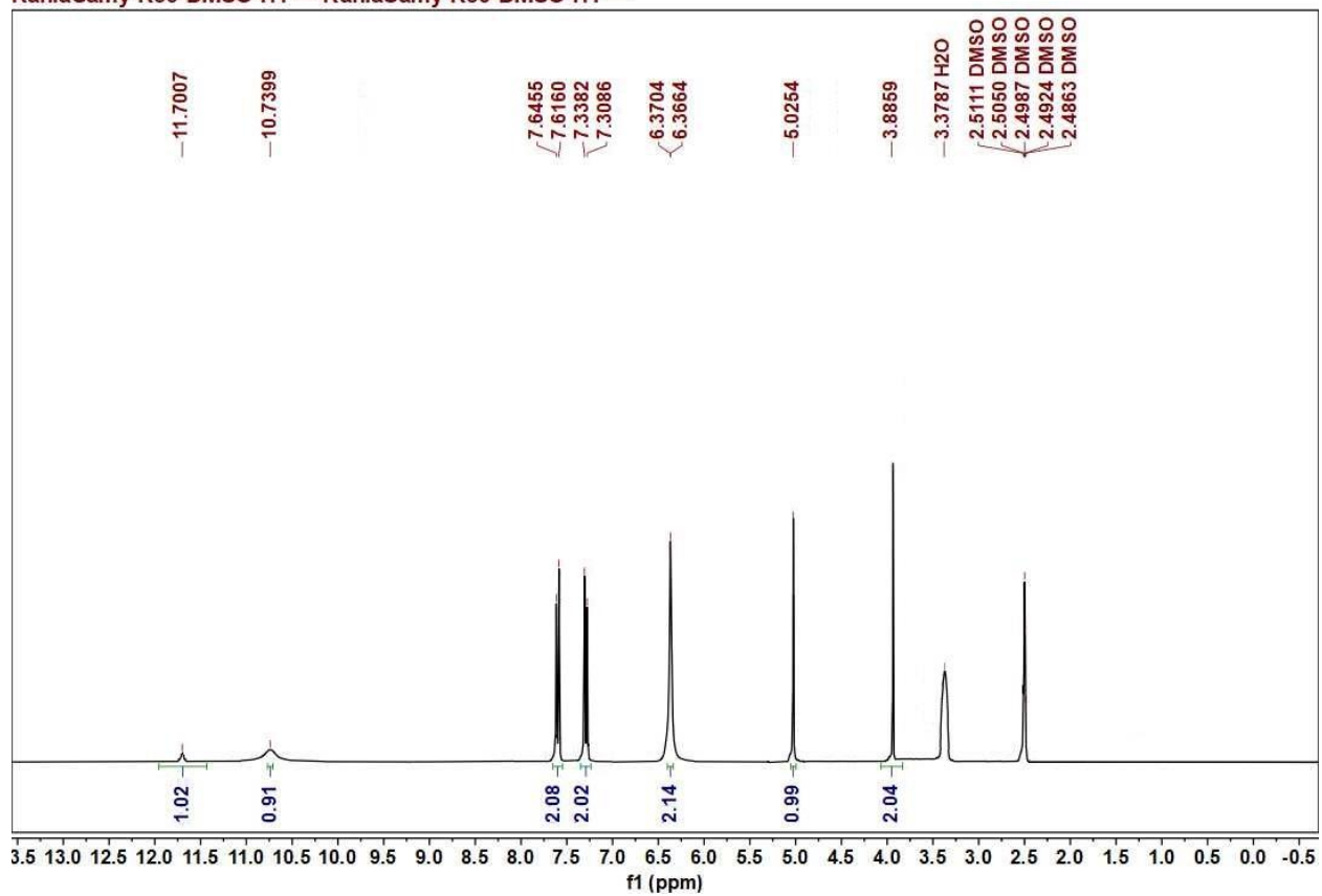
Figure 5. The 1 H NMR spectrum of compound 9d
