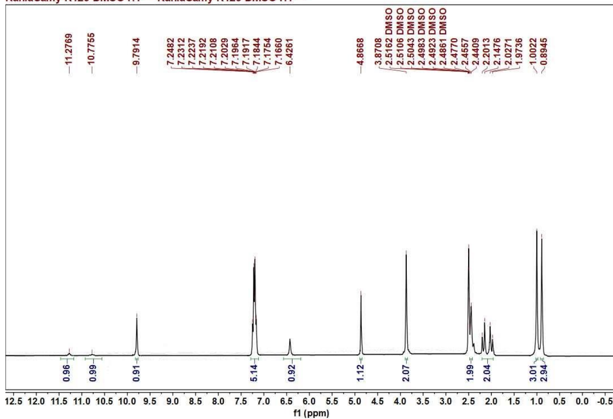
Figure 13. The 1 H NMR spectrum of compound 15a
