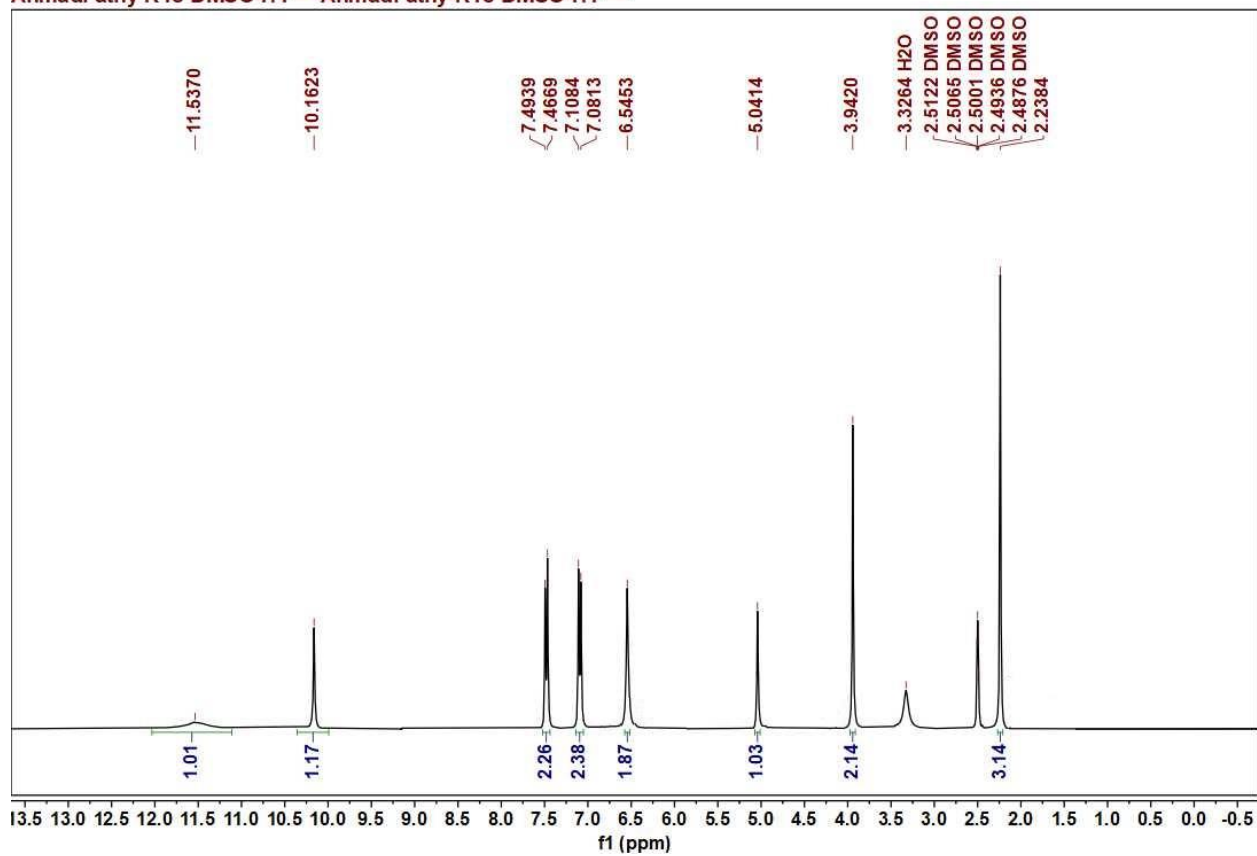
Figure 2. The 1 H NMR spectrum of compound 9b
