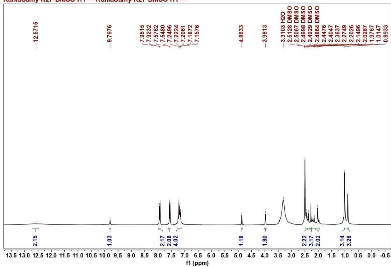
Figure 6. The 1 H NMR spectrum of compound 12b
