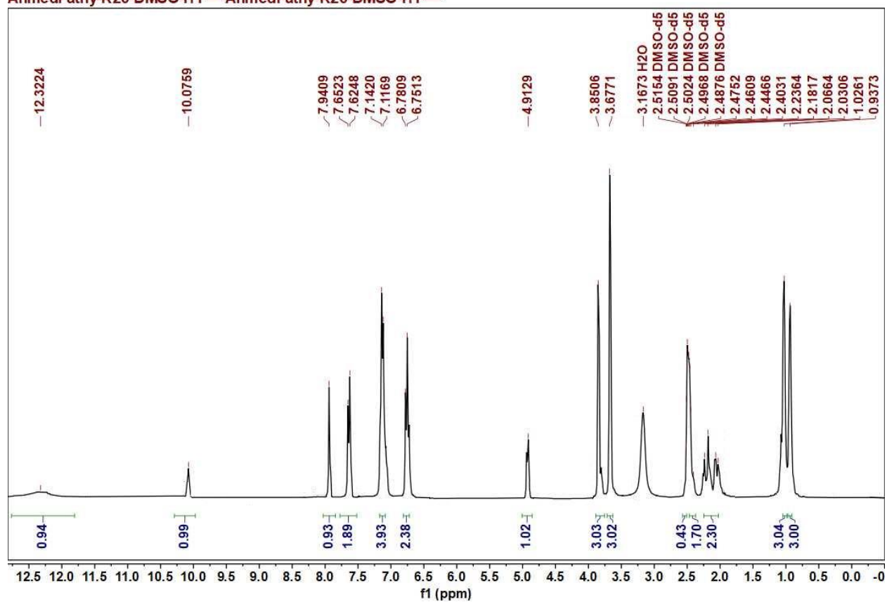
Figure 11. The 1 H NMR spectrum of compound 13d
