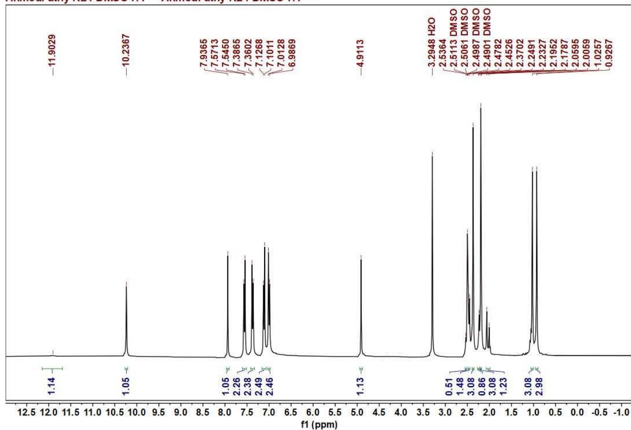
Figure 9. The 1 H NMR spectrum of compound 13c
