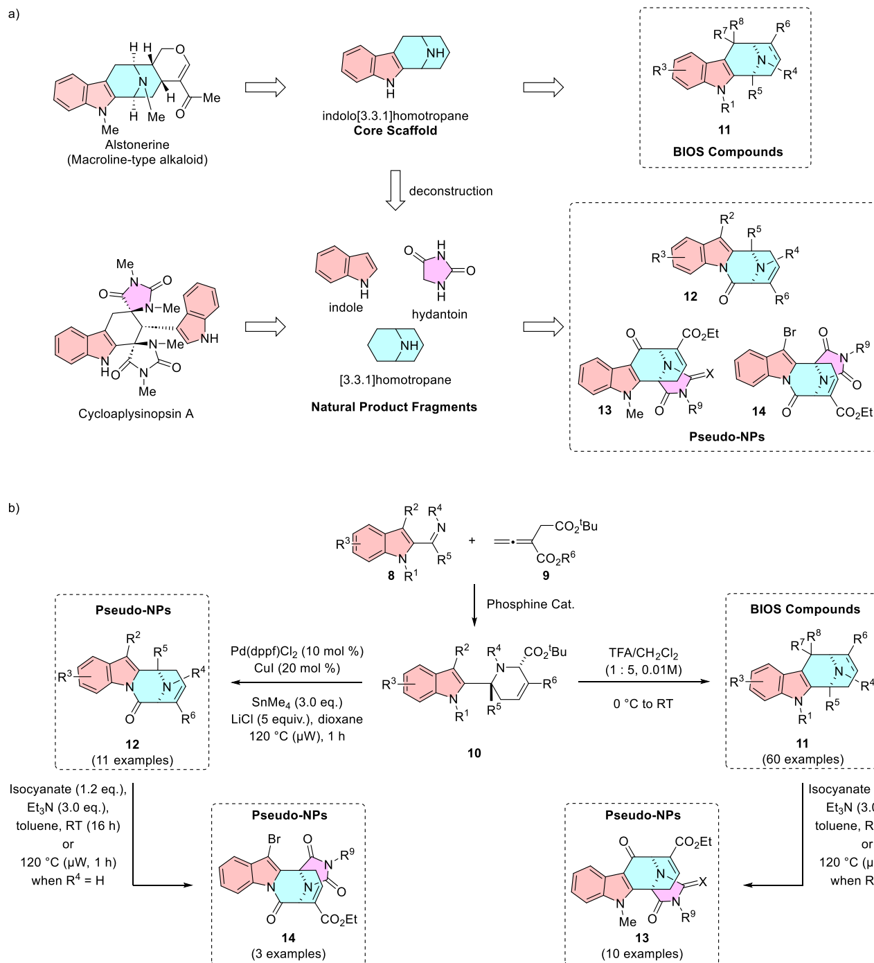
Figure 6. Design and synthesis of a biology-oriented synthesis- and PNP-inspired compound collection.
