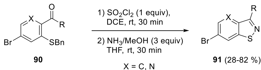
Scheme 31. Formation of benzo[ d ]isothiazoles from 5-(2-acetyl-5-bromophenyl) benzothioates, using sulfuryl chloride and ammonia. 8
