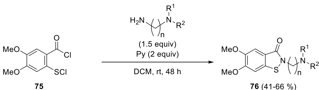
Scheme 26. Formation of benzo[ d ]isothiazolones from -(chlorocarbonyl)phenyl hypochlorothioites. 73
