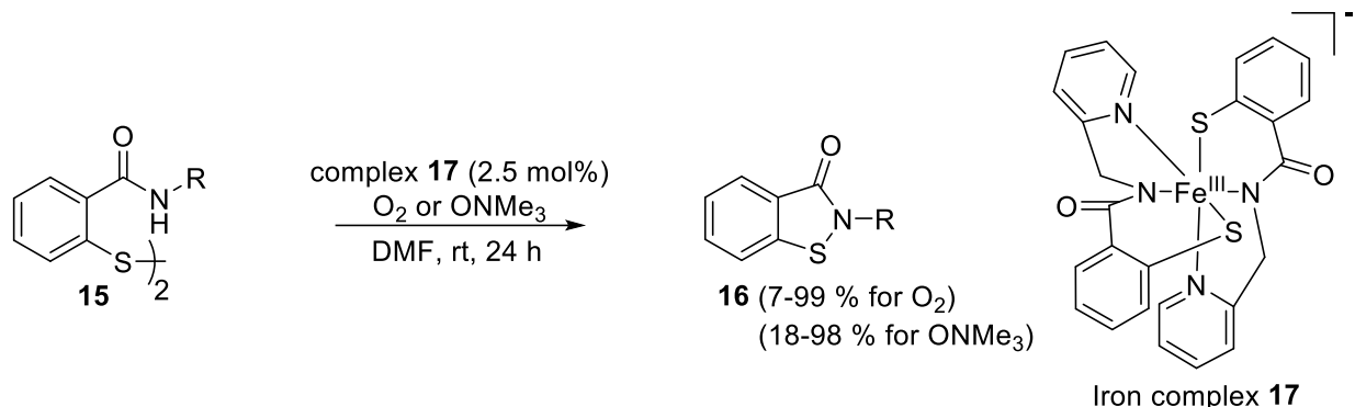
Scheme 4. Formation of benzo[ d ]isothiazolones from 2,2'-disulfaneyldibenzamides, catalyzed by mononuclear iron (III) complex 17 . 39
