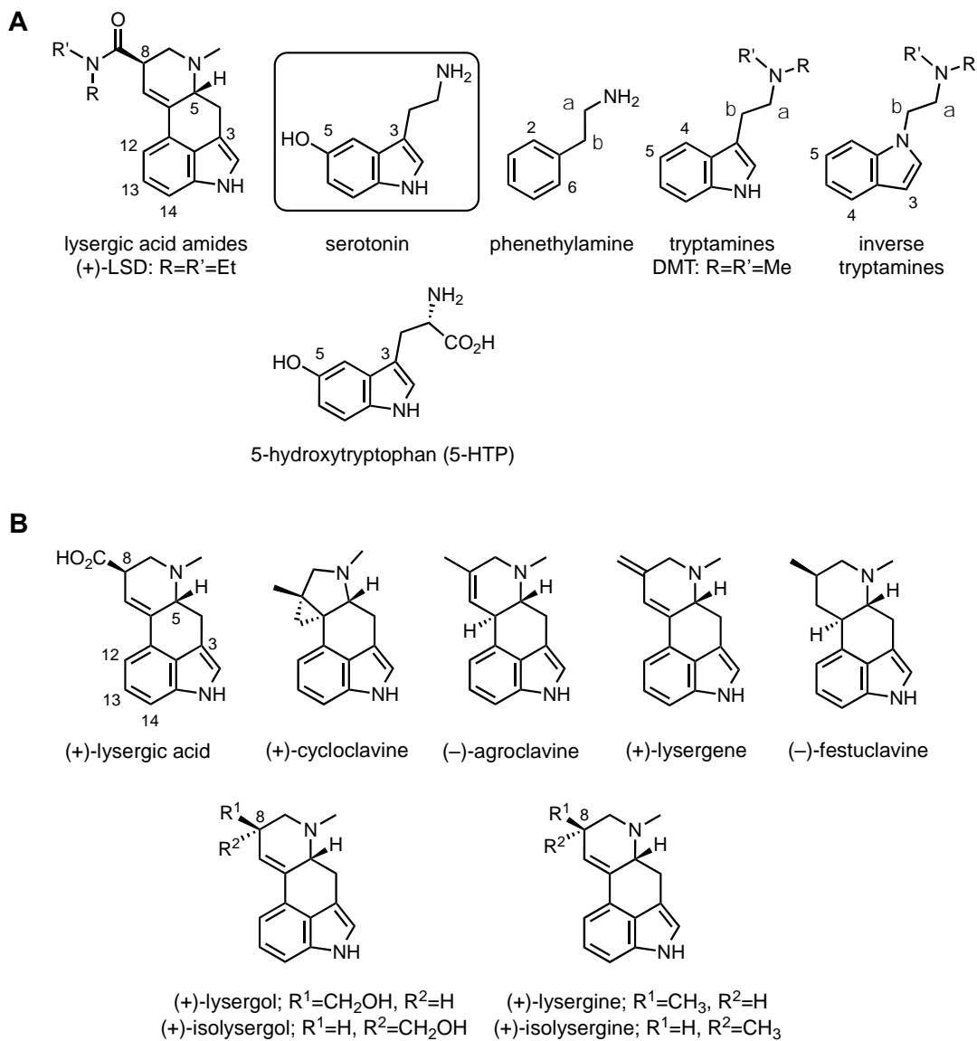
Figure 1. Panel A: Serotonin (5-HT), 5-hydroxytryptophan (5-HTP) and synthetic 5-HT 2A ligands. Panel B: Lysergic acid and representative ergot (lysergic acid) and clavine (cycloclavine, agroclavine, lysergol, lysergene, festuclavine, lysergine) natural products.
