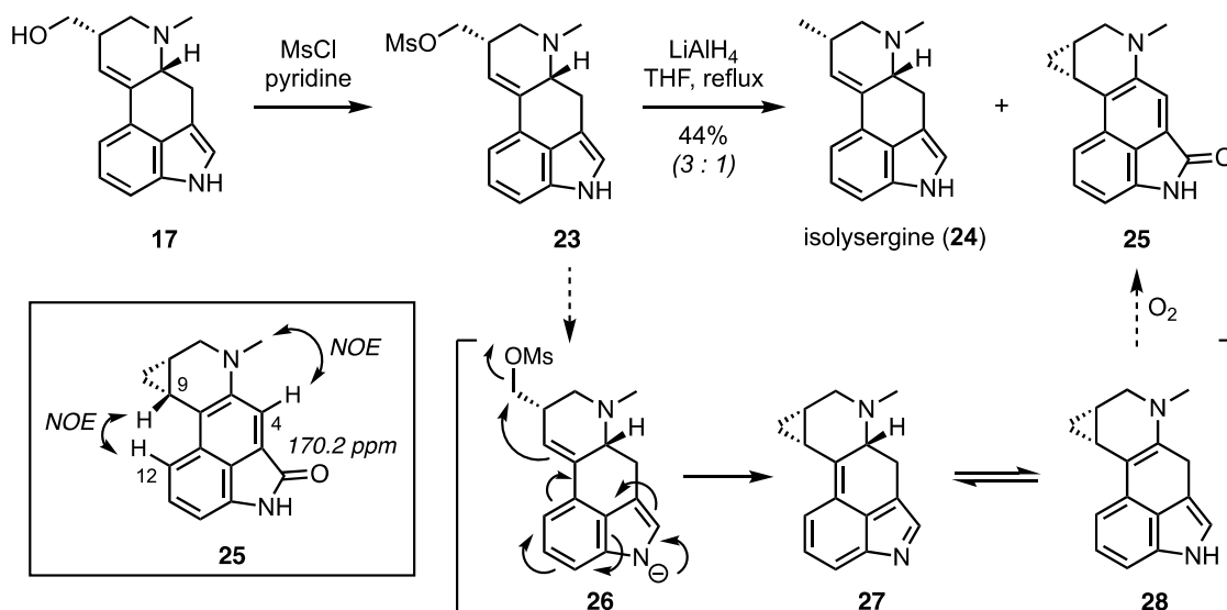
Scheme 4. Syntheses of ( \pm )-isolysergine ( 24 ) and the novel ergolin-2(3 H )-one 25 . Mechanistic hypothesis for the formation of 25 by air-oxidation of 28 , and key spectroscopic evidence for the structure of 25 .
