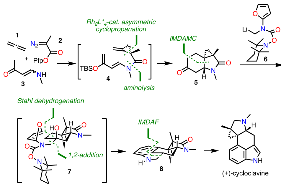
Scheme 1. Overview of an 8-step asymmetric total synthesis of (+)-cycloclavine. 16
