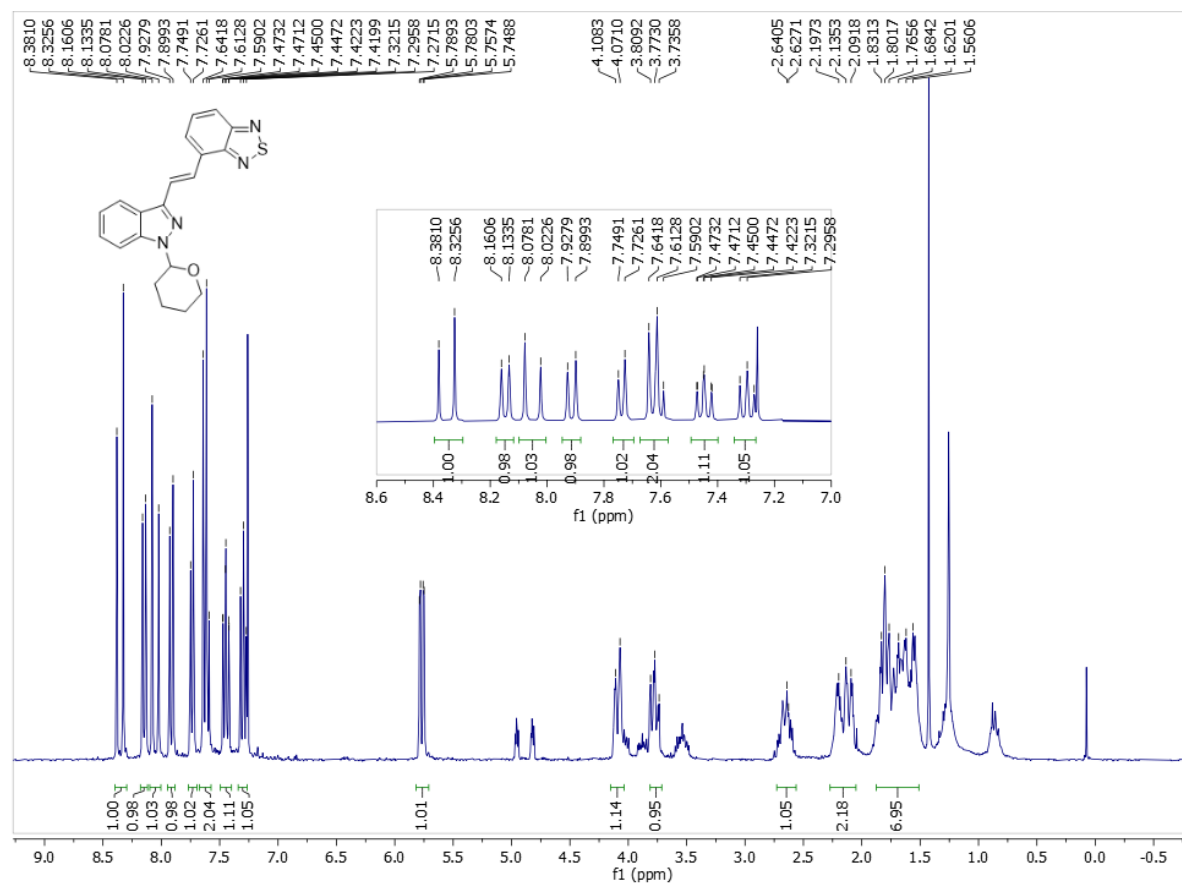
Figure S 8. 4-(2-(1-(tetrahydro-2H-pyran-2-yl)indazol-3-yl)vinyl)benzo[c][1,2,5]thiadiazole (13)
