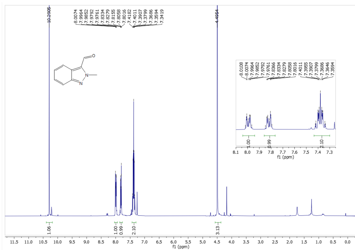
Figure S 10. 2-methyl-2H-indazole-3-carbaldehyde ( 15 )
