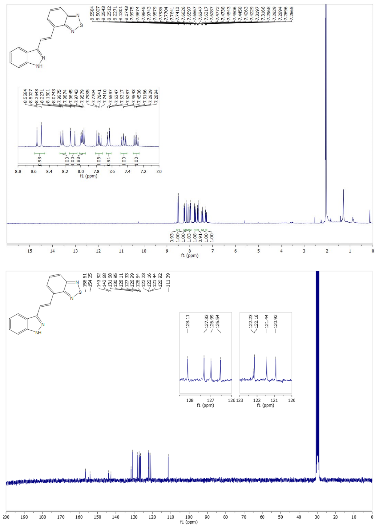
Figure S 1. NMR spectra of 4-(2-(1H-indazol-3-yl)vinyl)benzo[c][1,2,5]thiadiazole ( 2 )
