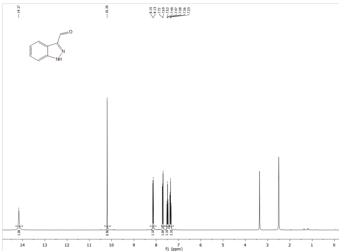
Figure S 6. 1H-indazole-3-carbaldehyde ( 11 )
