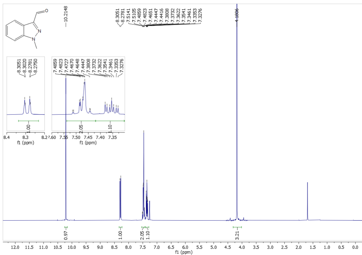
Figure S 9. 1-methyl-1H-indazole-3-carbaldehyde ( 14 )
