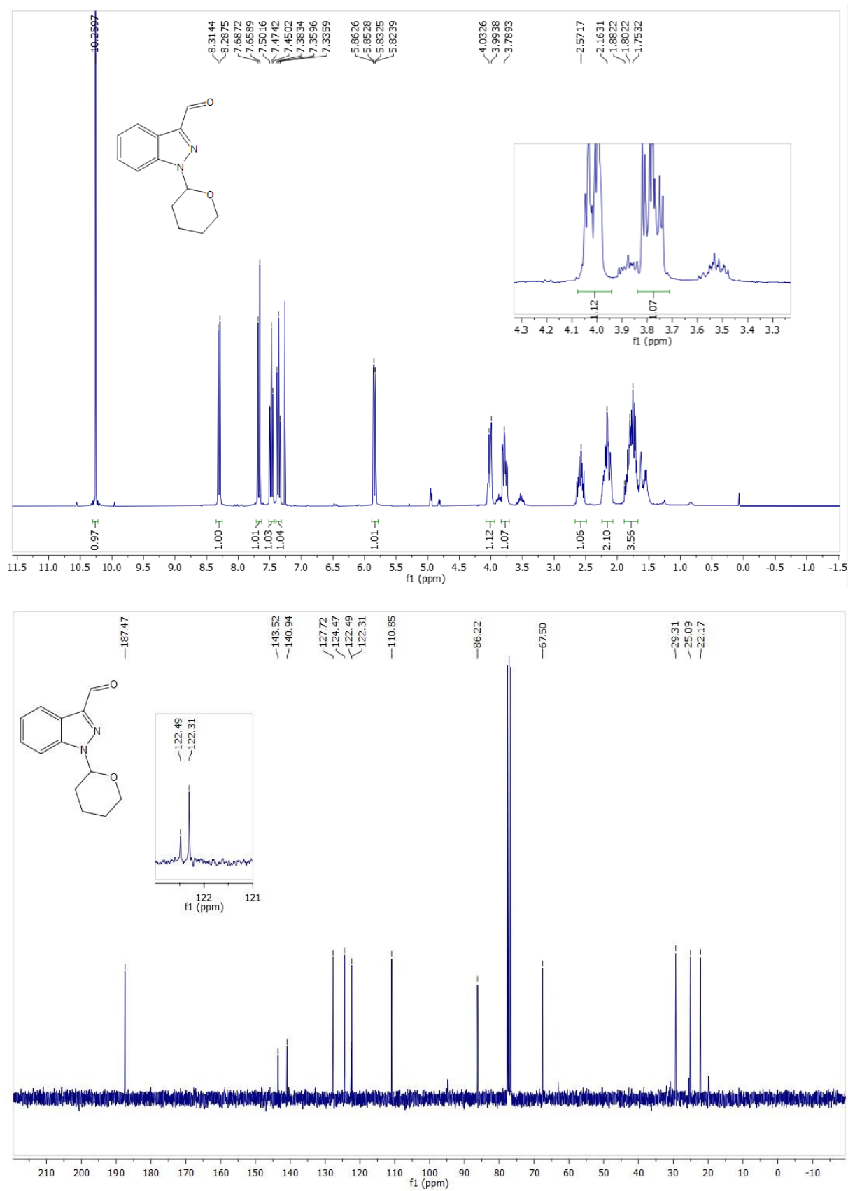
Figure S 7. 1-(tetrahydro-2H-pyran-2-yl)indazole-3-carbaldehyde ( 12 )
