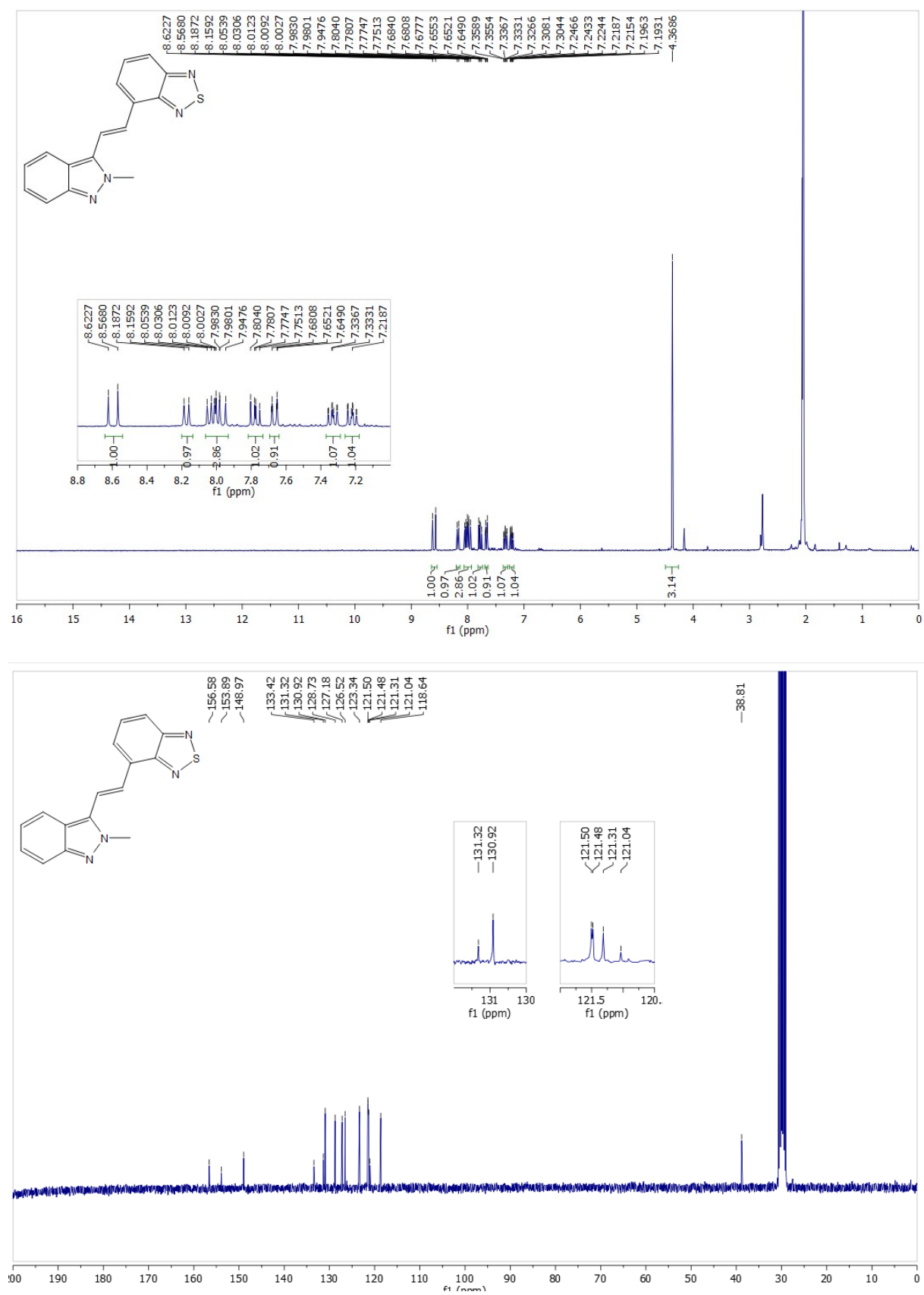
Figure S 3. NMR spectra of 4-(2-(2-methyl-2H-indazol-3-yl)vinyl)benzo[c][1,2,5]thiadiazole ( 4 )
