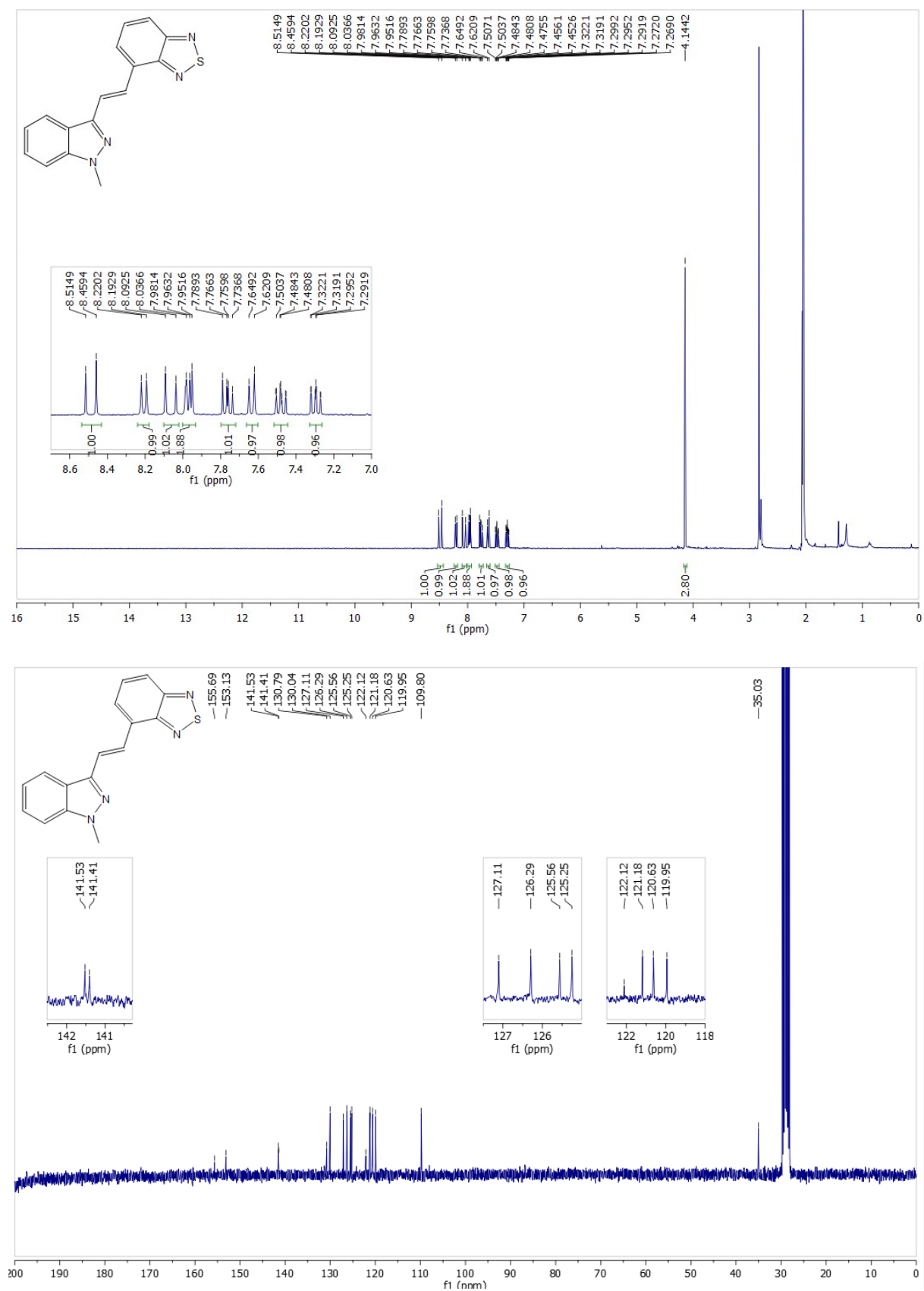
Figure S 2. NMR spectra of 4-(2-(1-methyl-1H-indazol-3-yl)vinyl)benzo[c][1,2,5]thiadiazole (3)
