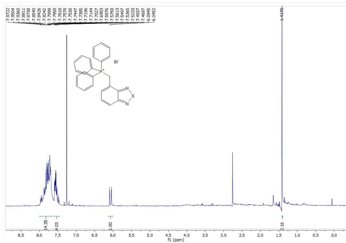
Figure S 5. (Benzo[ c ][1,2,5]thiadiazol-4-ylmethyl)triphenylphosphonium bromide ( 9 )
