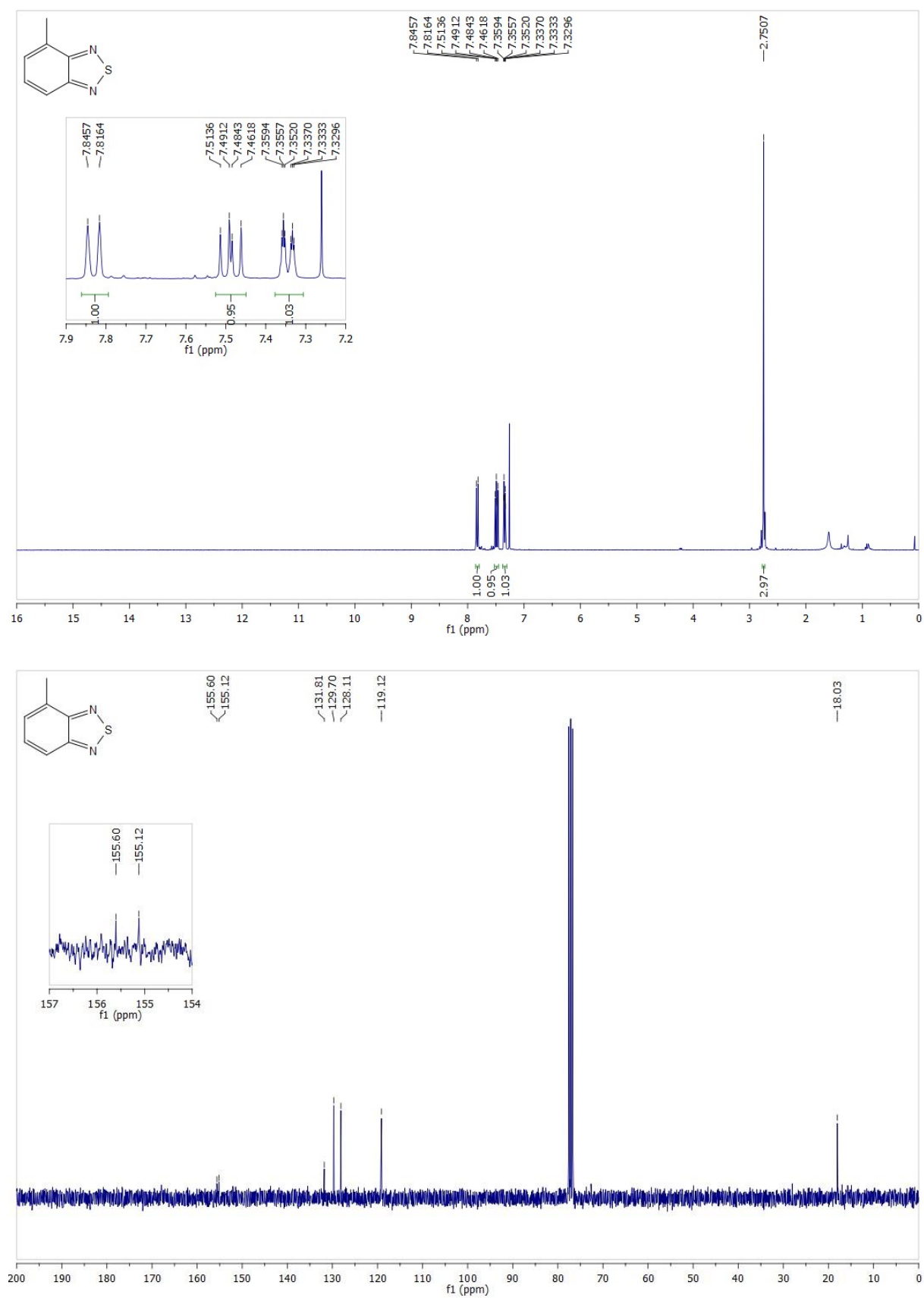
Figure S 4. 4-methylbenzo[c][1,2,5]thiadiazole ( 7 )
