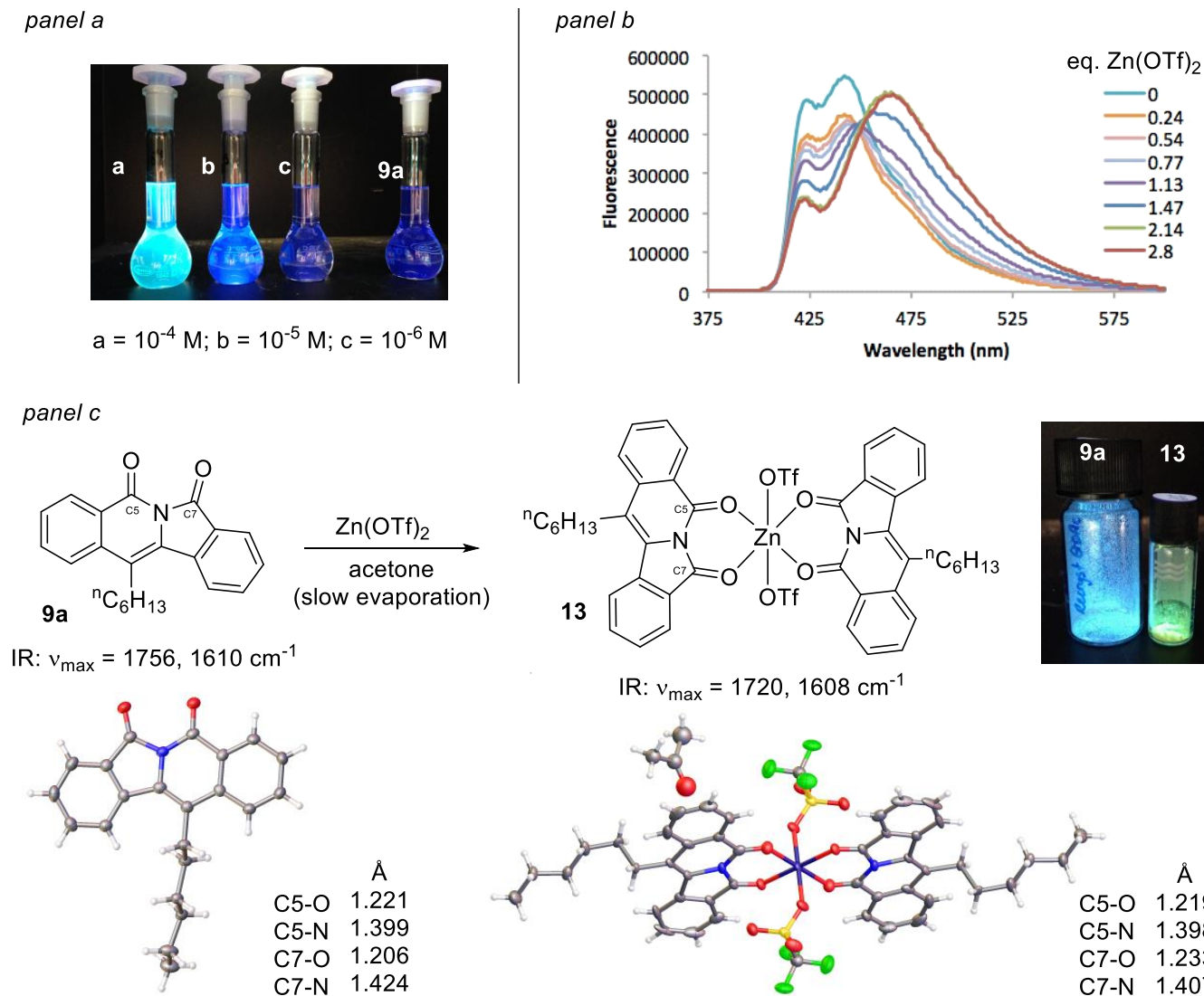
Figure 3. Panel a: fluorescence of 2:1 mixtures of 9a and \text{Zn}(\text{OTf})_2 at varying concentrations in EtOAc; panel b: fluorescence titration of 9a ( 2 \times 10^{-4} M in dichloromethane) and \text{Zn}(\text{OTf})_2 in dichloromethane; panel c: crystallographic and IR data for 9a and zinc complex 13 , plus solid-state fluorescence.
