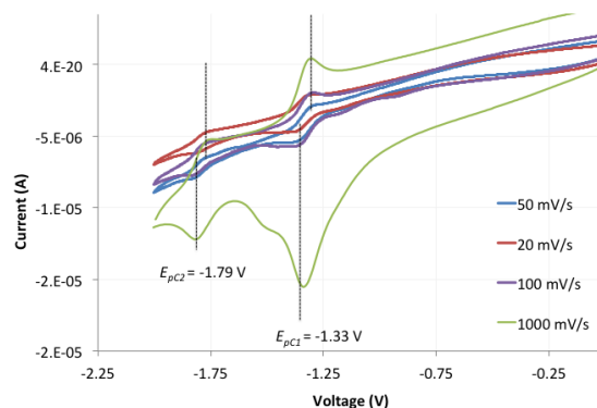
Figure 2. Cyclic voltammograms of 9a (1.0 mM) in non-aqueous media (CH 3 CN/[ n Bu 4 N]BF 4 0.10 M).
