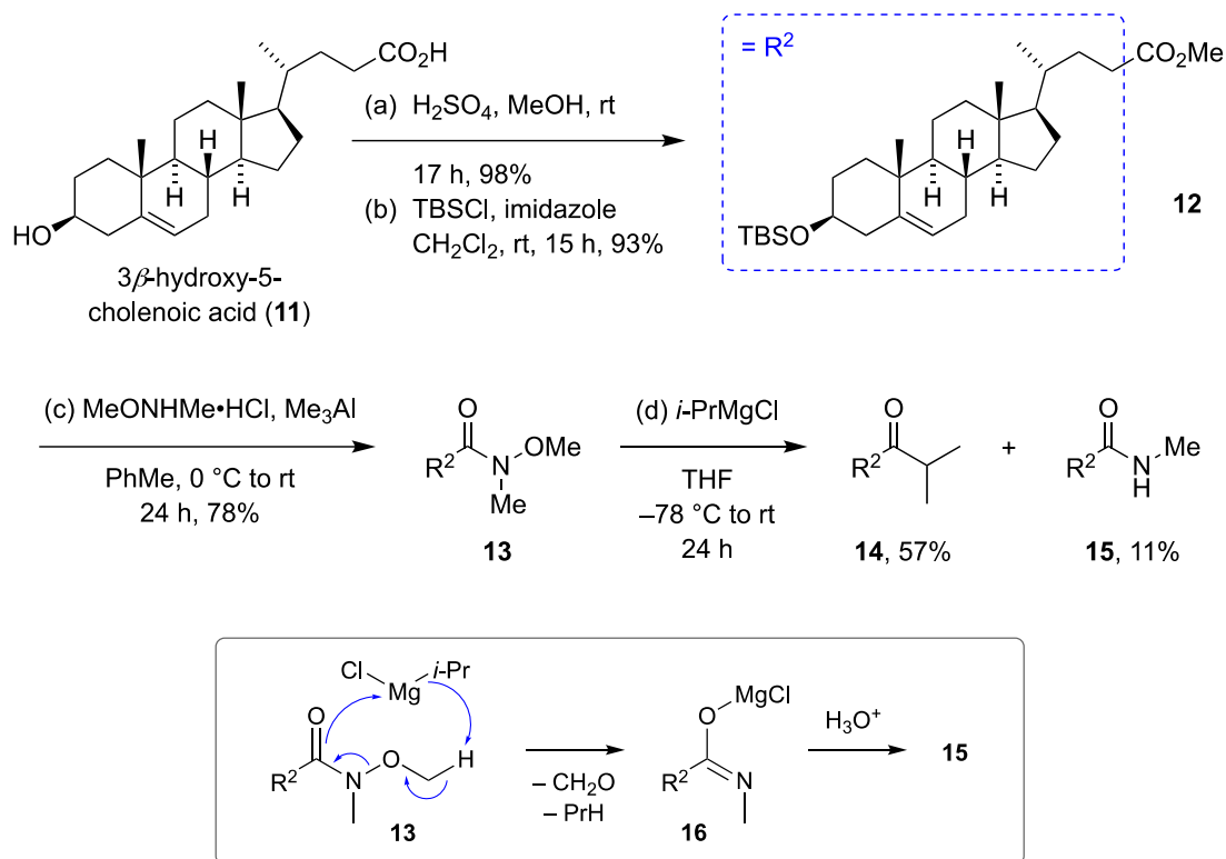
Scheme 3. Conversion of 3β-hydroxy-5-cholenoic acid (11) to a 24-ketocholesterol derivative (14) via Weinreb amide 13 and observation of demethoxylation side-product (15) formation during addition of isopropylmagnesium chloride. Insert = putative mechanism for demethoxylation.
