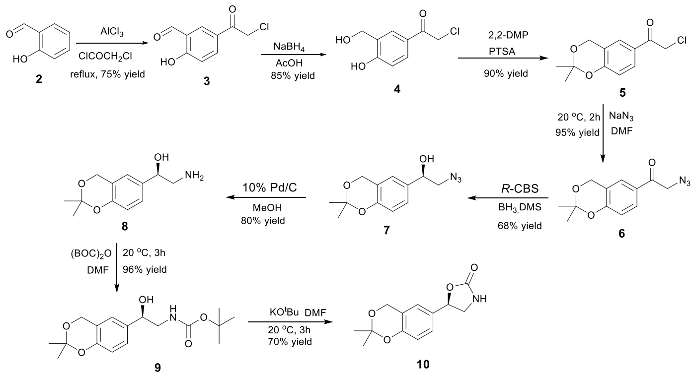
Scheme 3. Synthesis of oxazolidinone compound ( 10 ).
