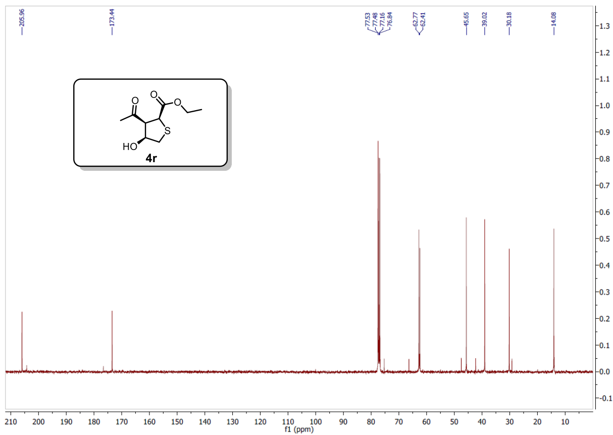
400 MHz ^1\text{H} NMR and 100 MHz ^{13}\text{C} NMR Spectra of 4r
