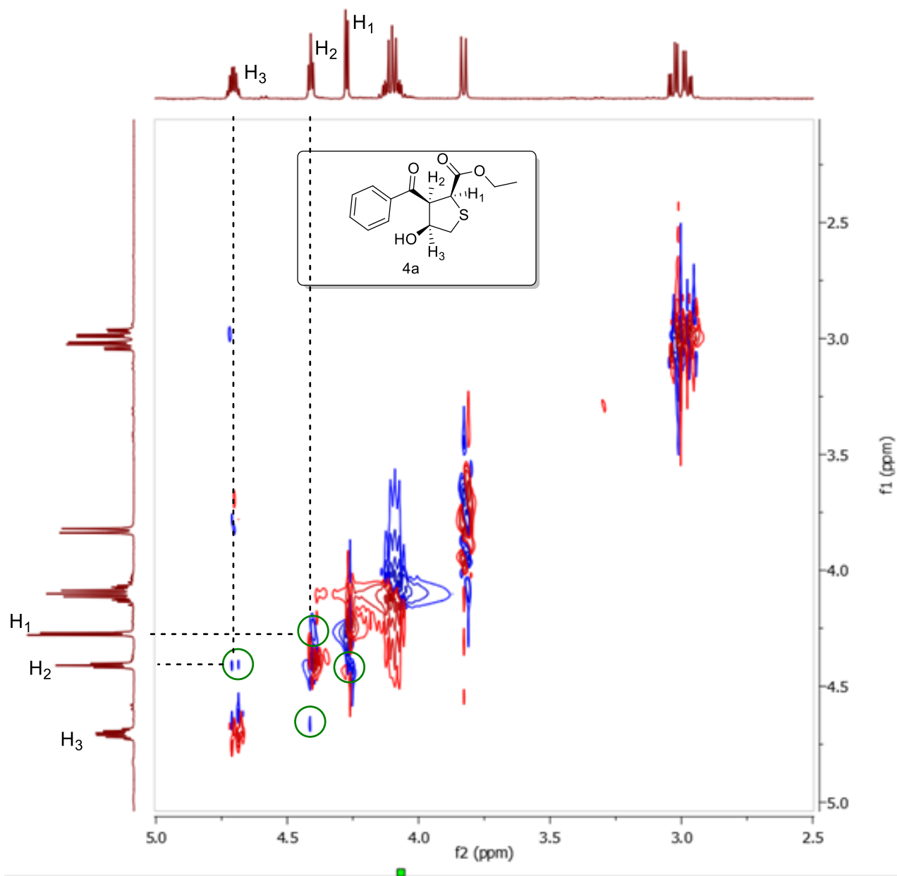
500 MHz NOESY Spectra of 4a
