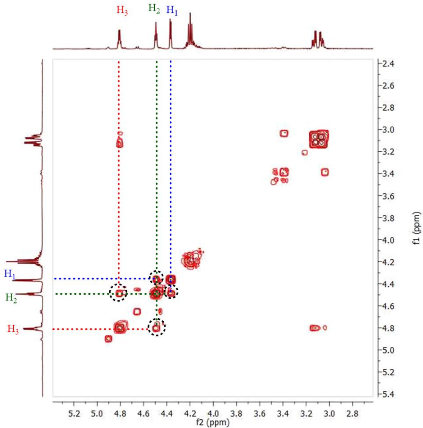
500 MHz ^1\text{H} - ^1\text{H} COSY Spectra of 6a
