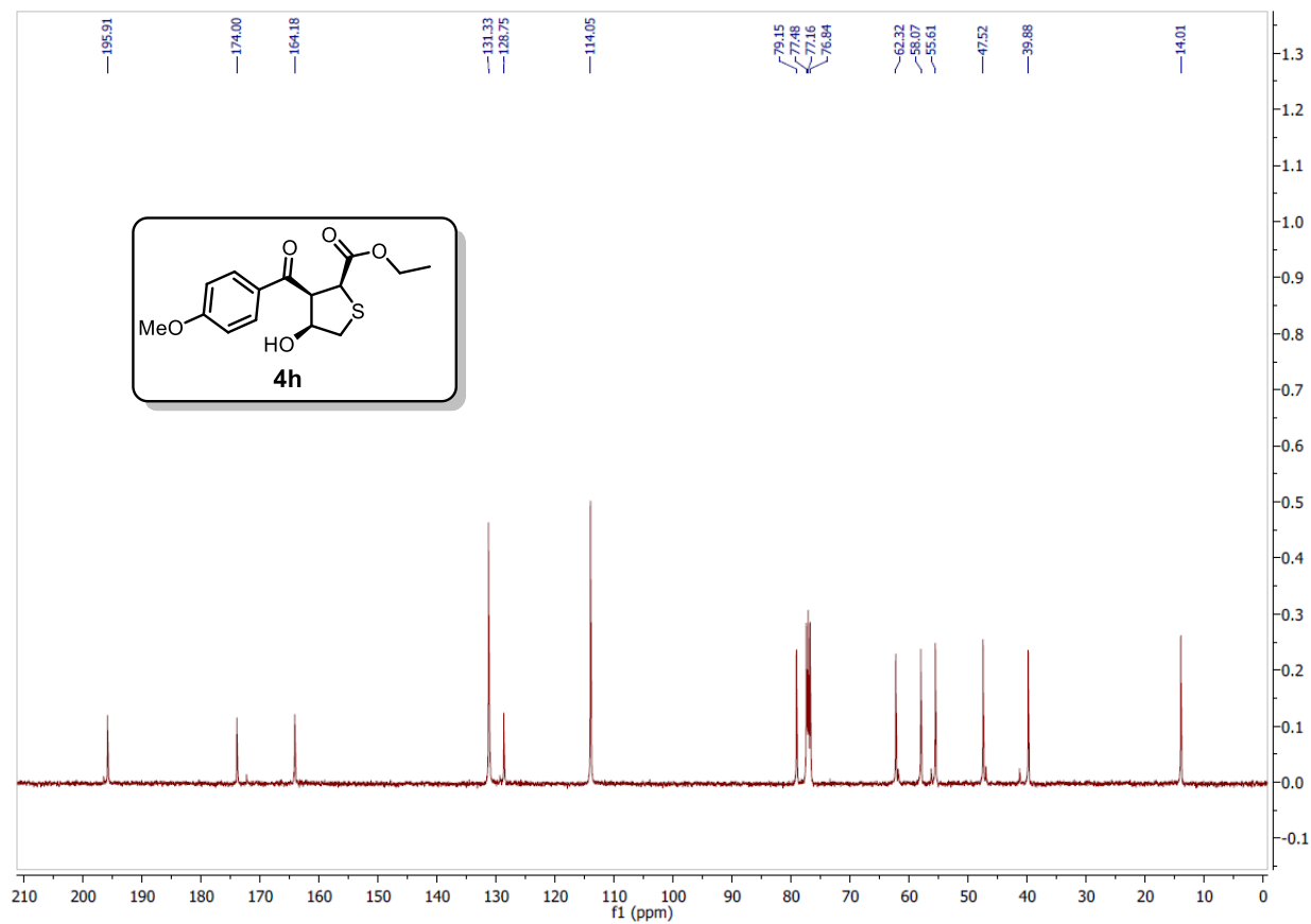
400 MHz 1 H NMR and 100 MHz 13 C NMR Spectra of 4h
