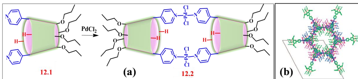
Scheme 12. (a) Synthetic scheme for the upper rim pyridyl calix[4] derivative to form a metallocyclic calix[4]arene tube, 12.2 . (b) Formation of calix-wheel in the crystal structure of 12.2 .
