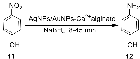
Scheme 5 The Catalytic reduction of 4-nitrophenol in the presence of AgNPs/AuNPs-Ca 2+ -alginate.
