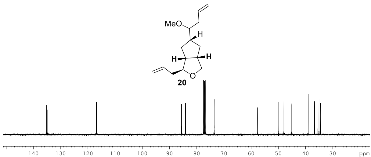
Figure 28. ^{13}\text{C} NMR spectrum of 20 .
