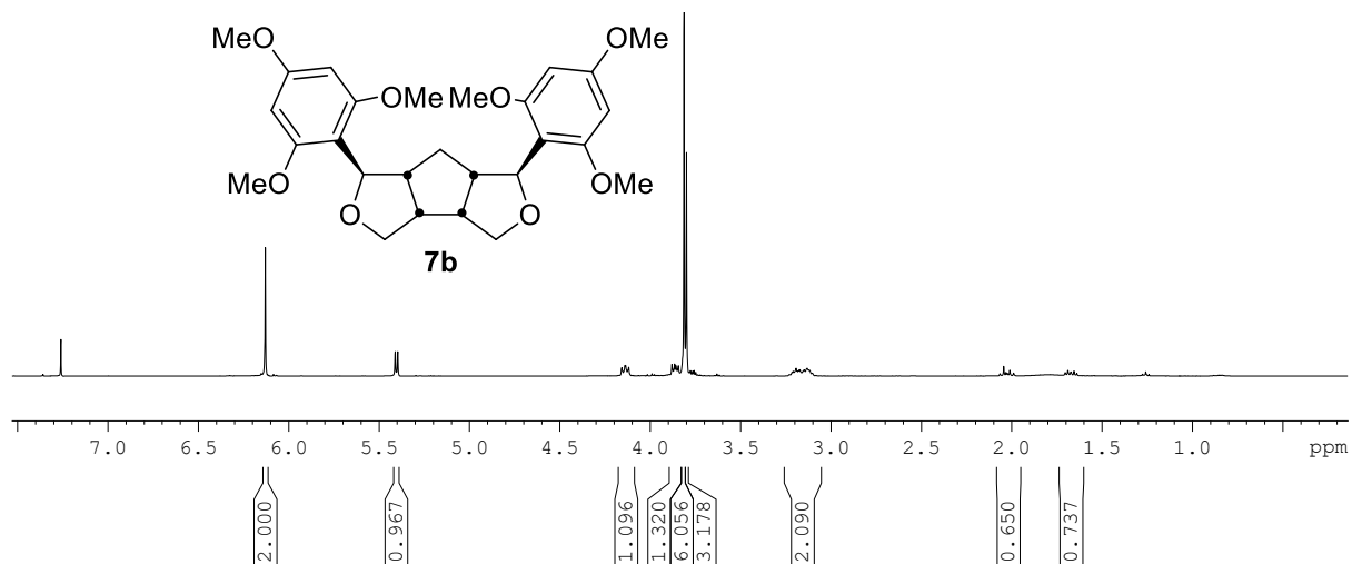
Figure 5. 1 H NMR spectrum of 7b .
