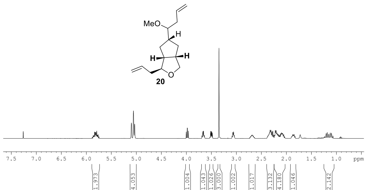
Figure 27. ^1\text{H} NMR spectrum of 20 .
