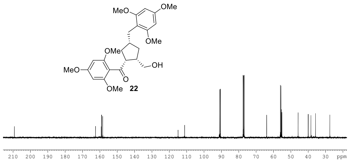
Figure 30. ^{13}\text{C} NMR spectrum of 22 .
