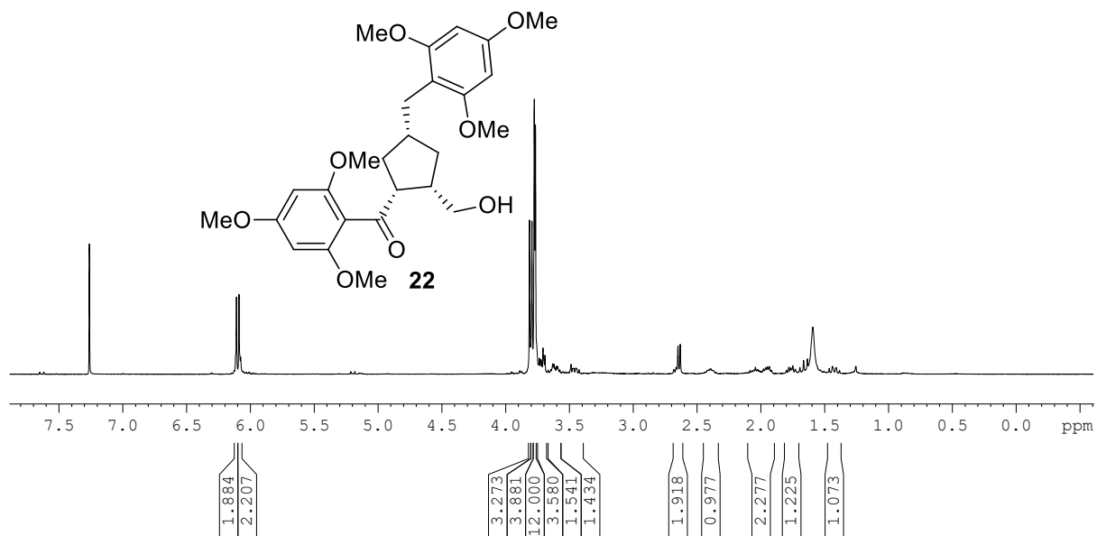
Figure 29. ^1\text{H} NMR spectrum of 22 .
