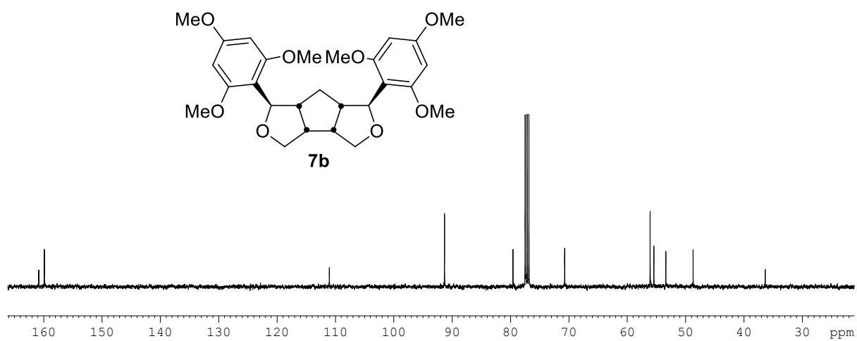
Figure 6. 13 C NMR spectrum of 7b .
