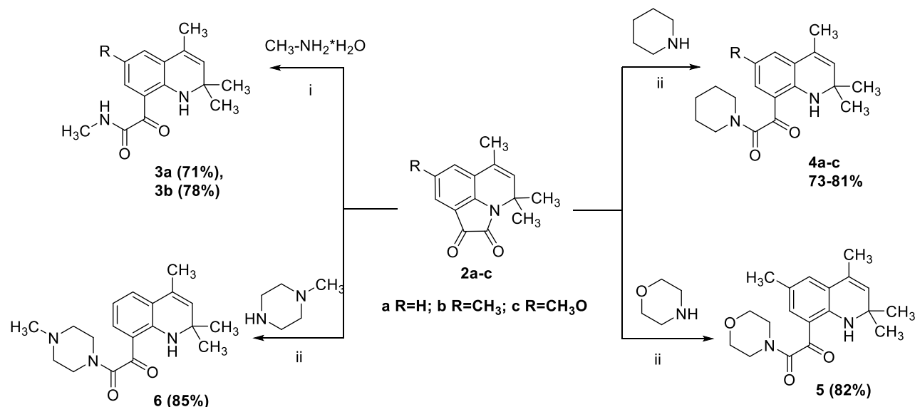
Scheme 3. Synthesis of 1,2-dihydroquinoline-8-glyoxylamides 3a-b , 4a-c , 5-6 . Reagents and conditions: (i) \text{CH}_3\text{NH}_2 (40% solution), EtOH, 60^\circ\text{C} , 30 min, 71–78%; (ii) secondary amines (5 eq), EtOH, 60^\circ\text{C} , 4–10 h, 73–85%.
