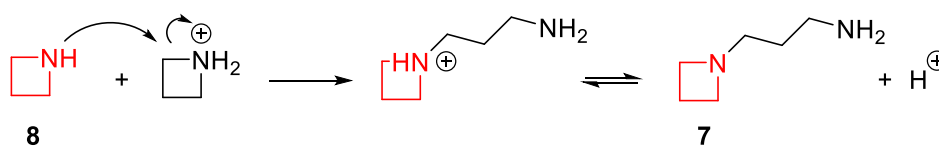
Scheme 4. Formation of 3-(azetidin-1-yl)propan-1-amine ( 7 ) via acid-catalyzed dimerization according to Schacht and Goethals (adapted from Sarazen and Jones). 33,34
