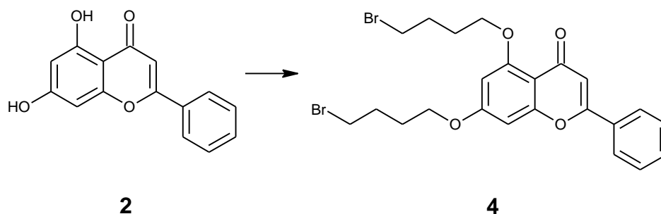
Scheme 1. The intended synthesis of compound 4 . Reagents and conditions: 1,4-dibromobutane, K_2CO_3 , CH_3CN .
