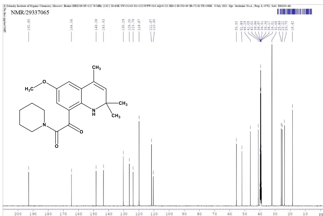
Figure 17 ^{13}\text{C} NMR (125 MHz, DMSO-d 6 , ppm) spectrum of compound 4c.
