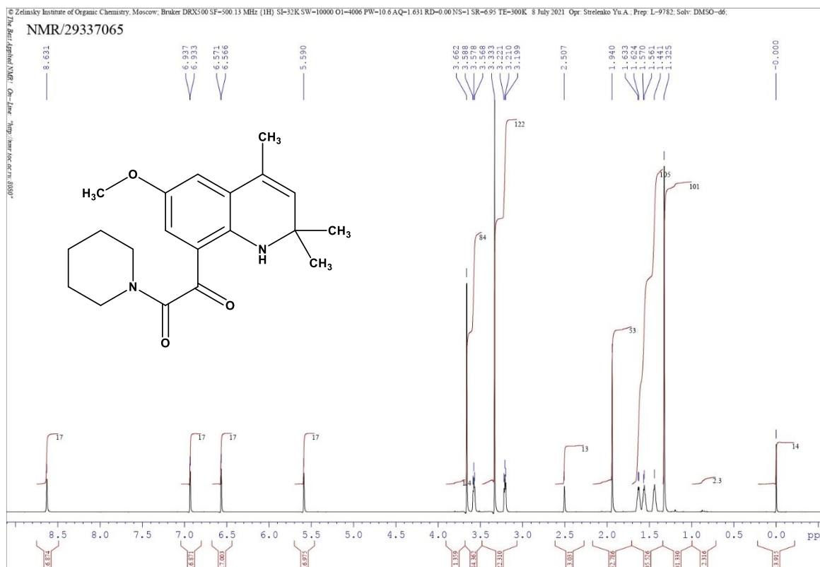
Figure 16 ^1\text{H} NMR (500 MHz, DMSO-d 6 , ppm) spectrum of compound 4c.
