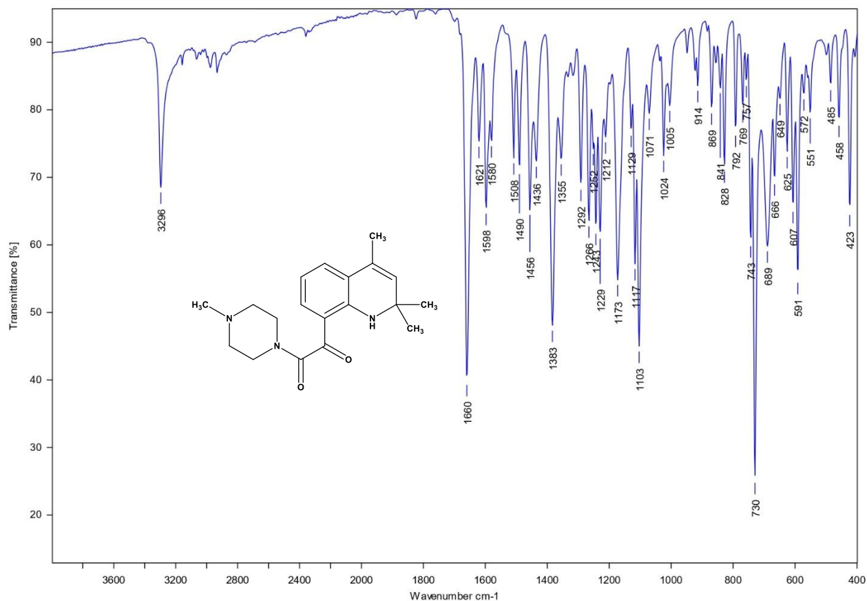
Figure 26 IR-spectrum (KBr, \text{cm}^{-1} ) of compound 6
