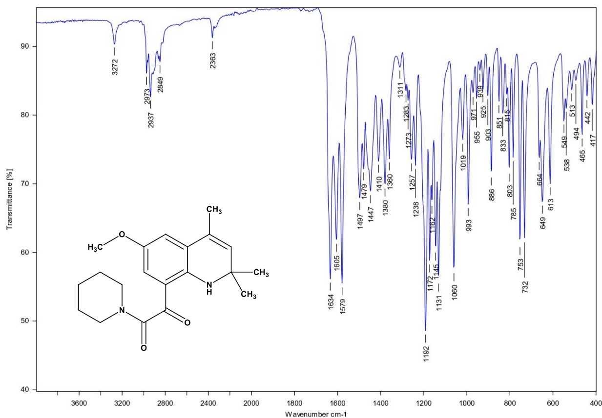
Figure 18 IR-spectrum (KBr, \text{cm}^{-1} ) of compound 4c .
