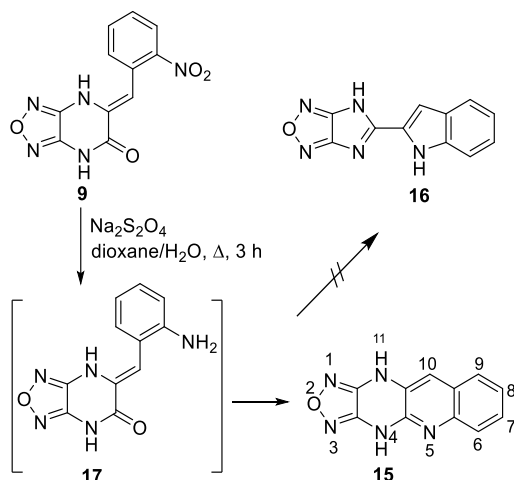
Scheme 8. Synthesis of 4,11-dihydro-[1,2,5]oxadiazolo[3',4':5,6]pyrazino[2,3- b ]quinoline ( 15 ).
