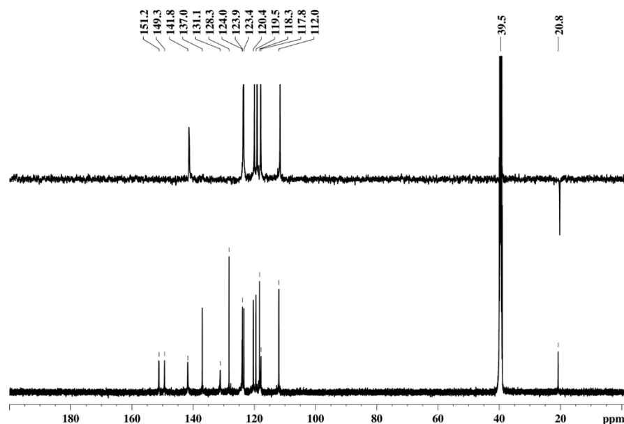
Figure 1. ^{13}\text{C}\{^1\text{H}\} (bottom) and DEPT (top) NMR spectra (126 MHz, DMSO, 303K) of 10 .
