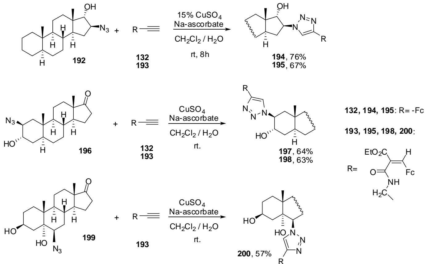
Scheme 43. Ferrocenyl triazole derivatives produced from steroidal azides 192 , 196 and 199 .
