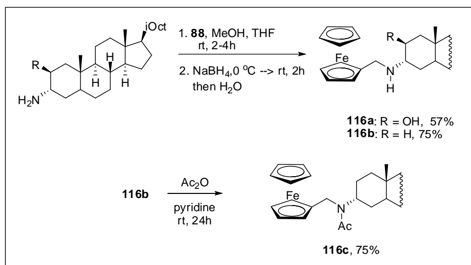
Scheme 21. Synthetic procedures towards (ferrocenylmethyl)amino-estranses 115a-f and (ferrocenylmethyl)amino-cholestanes 116a-c .
