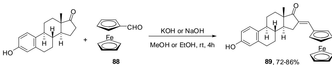
Scheme 16. Synthesis of 16-ferrocenylidene estrone ( 89 ).
