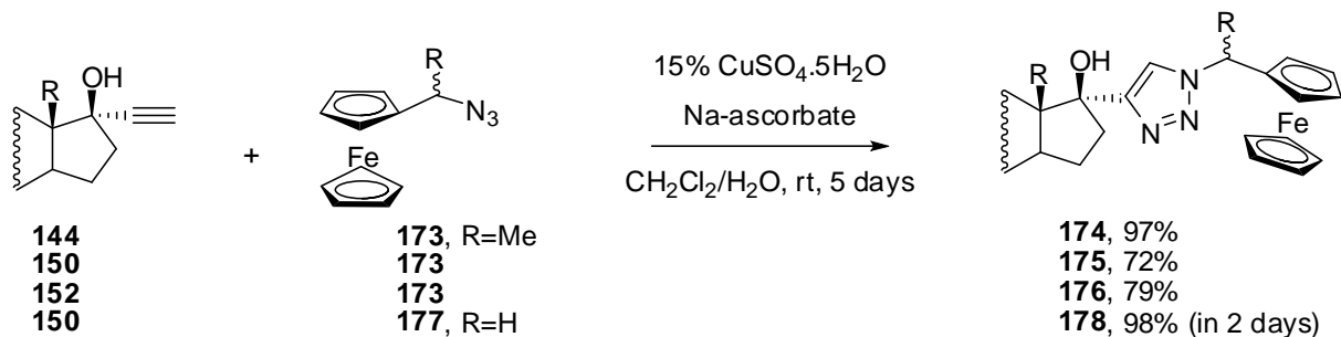
Scheme 38. Cycloaddition of 17 \alpha -ethynysteroids with ferrocenyl azides.
