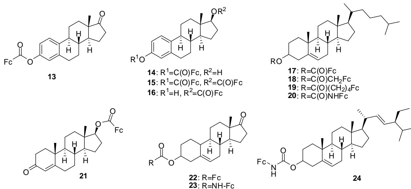
Figure 2. Products of acylation of steroid alcohols.
