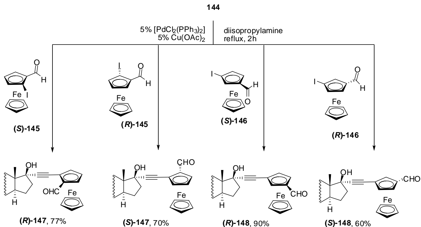
Scheme 32. Sonogashira coupling of 17 \alpha -ethynylestradiol ( 144 ) with formyl-iodoferrocenes.
