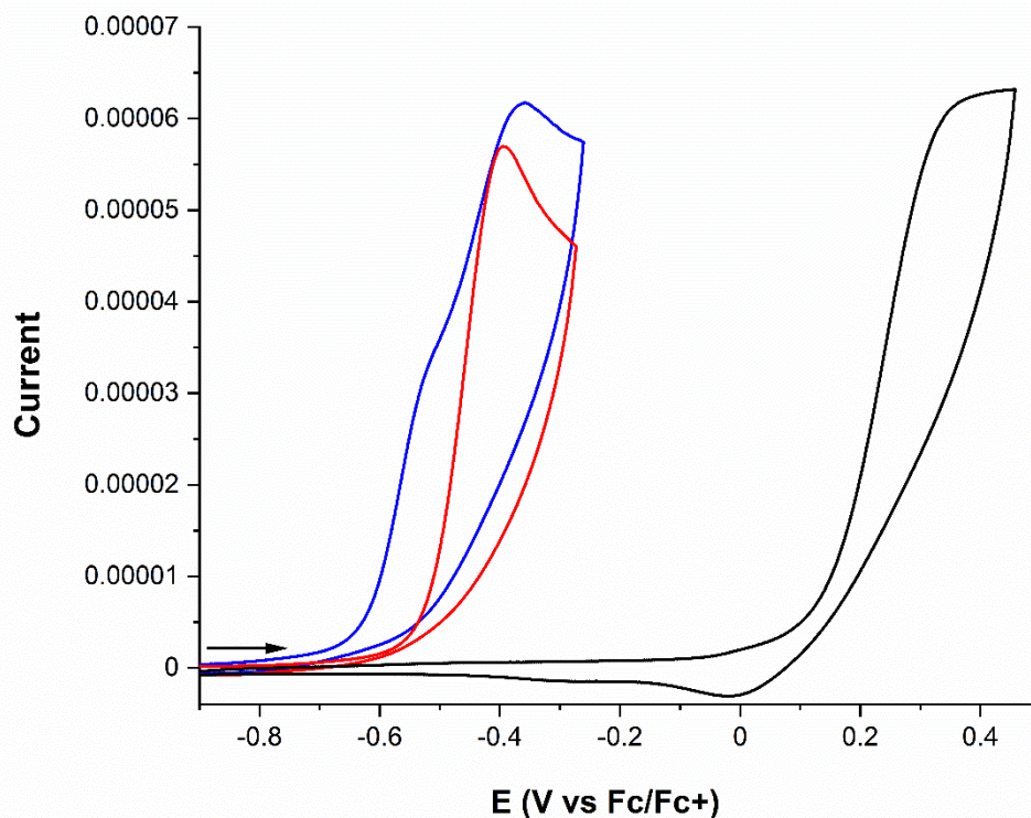
Figure 3. Cyclic voltammogram of [NMe 4 ] 2 [(PhO)Ni(CF 3 ) 3 ] ( 2 , blue), [NMe 4 ][PhO] (red), and [NMe 4 ][(MeCN)Ni(CF 3 ) 3 ] ( 1 , black) in MeCN. Complex, 10 mM; electrolyte, 100 mM [NBu 4 ][PF 6 ]; working and counter electrode, platinum; silver pseudoreference; scan rate 100 mVs -1 .
