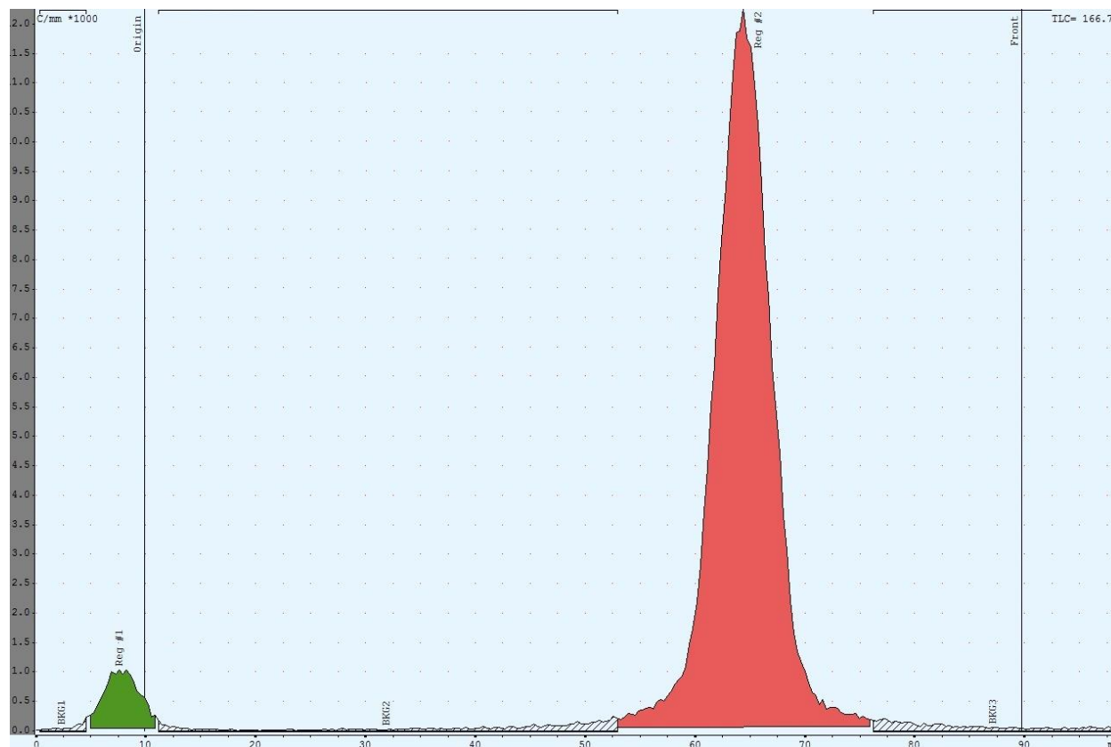
Figure 7. Radio-TLC chromatogram of the radiofluorination products of precursor 14c (CH 3 CN-H 2 O, 95:5) after purification. First peak from the left: impurity [ 18 F]KF•K 2 .2.2.2, second peak: 2-[ 18 F]-fluoro-5-nitrobenzoic acid 18 (RCP 98.0%).
