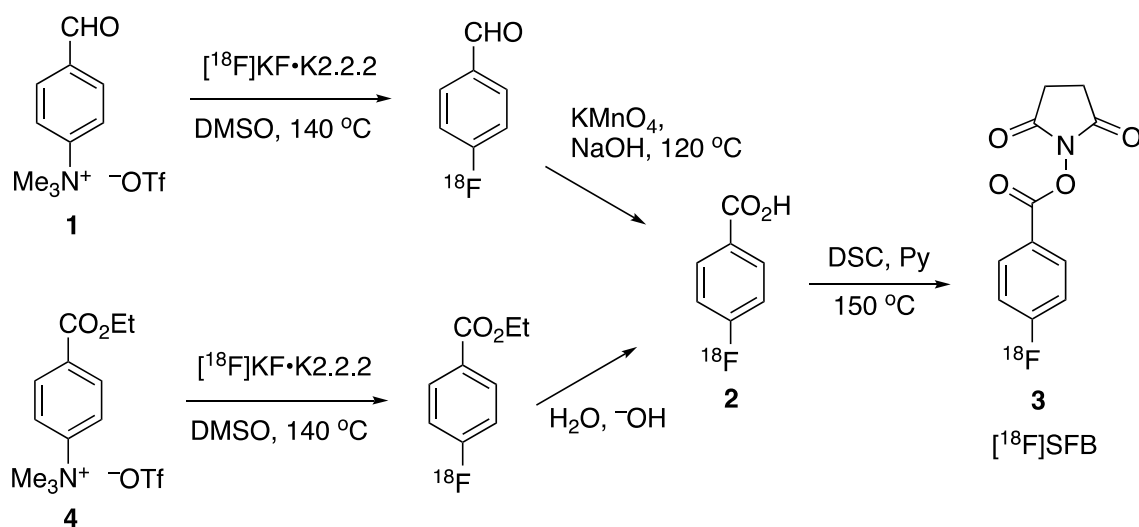
Scheme 1. Radiosynthesis of 4- [ ^{18}\text{F} ]fluorobenzoic acid 2 and [ ^{18}\text{F} ]SFB 3 .
