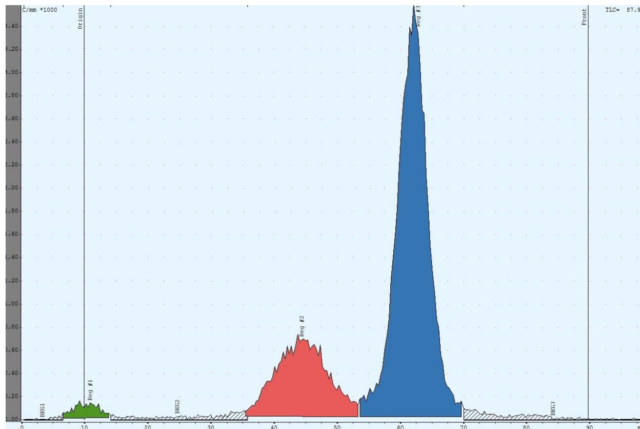
Figure 1. Radio-TLC chromatogram of the radiofluorination products of precursor 14b ( \text{CH}_3\text{CN}-\text{H}_2\text{O} , 95:5) after purification. First peak from the left: impurity [\text{}^{18}\text{F}]\text{KF}\cdot\text{K}_2.2.2 , second peak: benziodoxole [\text{}^{18}\text{F}]\text{fluoride} 17 , third peak: 2- [\text{}^{18}\text{F}] -fluoro-5-nitrobenzoic acid 18 (RCP 75%).
