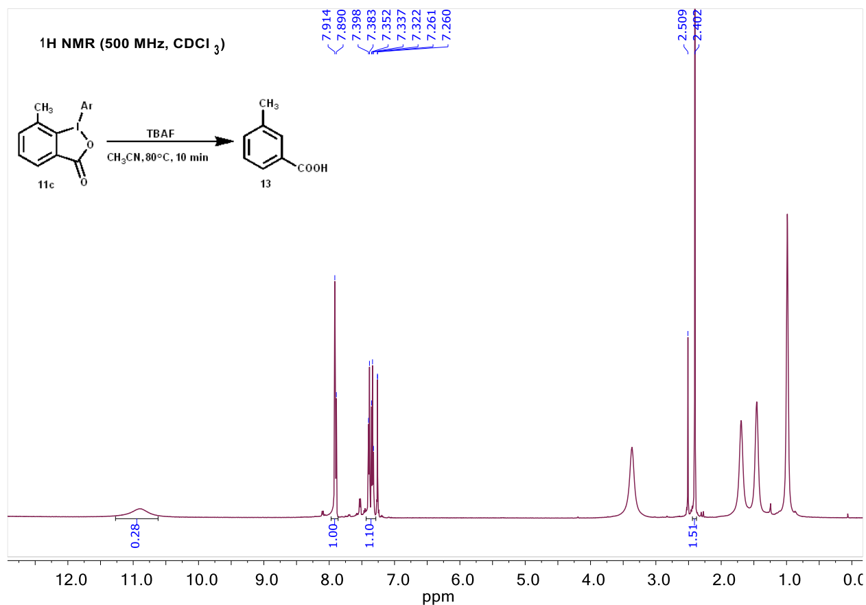
Figure 5. ^1\text{H} NMR spectrum of the reaction of 1-arylbenziodoxolone 11c with TBAF without TEMPO (Method C).
