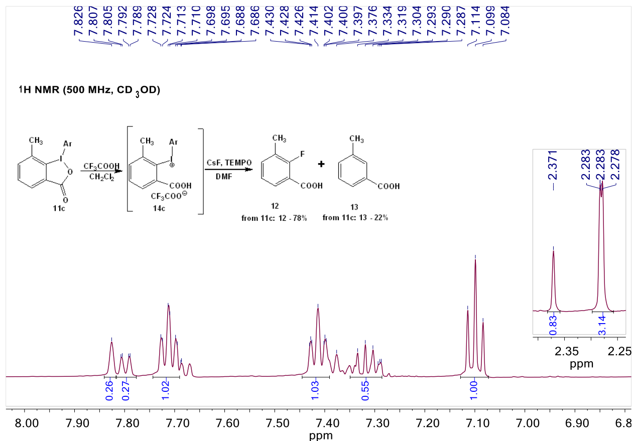
Figure 3. 1 H NMR spectrum of the reaction of 1-arylbenziodoxolone 11c with CsF (Method A).
