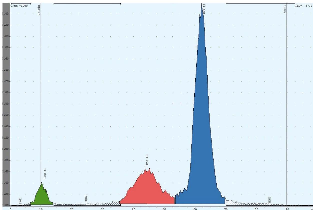
Figure 6. Radio-TLC chromatogram of the radiofluorination products of precursor 14b (CH 3 CN-H 2 O, 95:5) after purification. First peak from the left: impurity [ 18 F]KF•K2.2.2, second peak: benziodoxole [ 18 F]fluoride 17 , third peak: 2-[ 18 F]-fluoro-5-nitrobenzoic acid 18 (RCP 67%).
