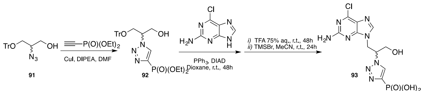
Scheme 31. Synthetic pathway to compound 93 .
