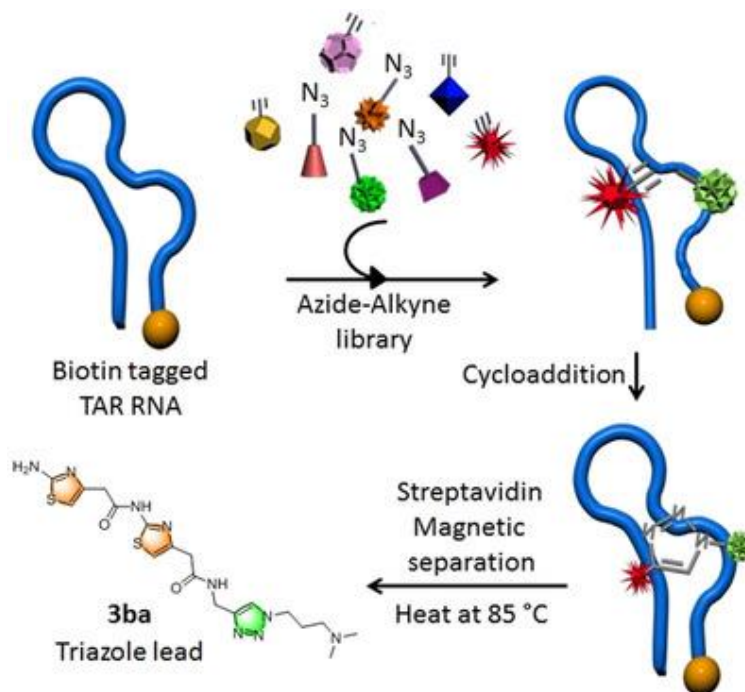
Figure 24. Identification of binding sites strategy (Reproduced with permission. 123 Copyright Year, Publisher).
