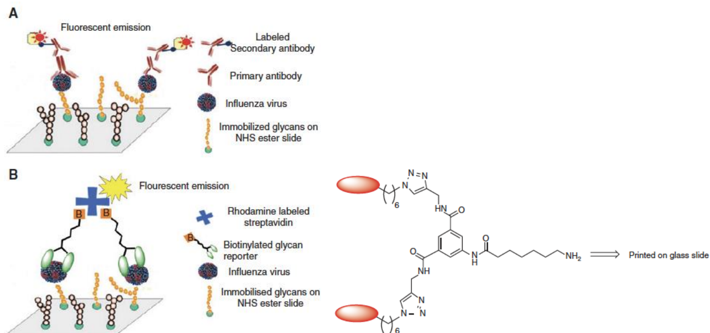
Figure 14. (A) Representation of the sandwich assay using glycans as capture and labeled antibody as reporters. (B) Representation of the sandwich assay using glycans as capture and biotinylated glycan-labeled streptavidin as reporters. Azide chemistry produces the triazole rings as the linkers between the two moieties.
