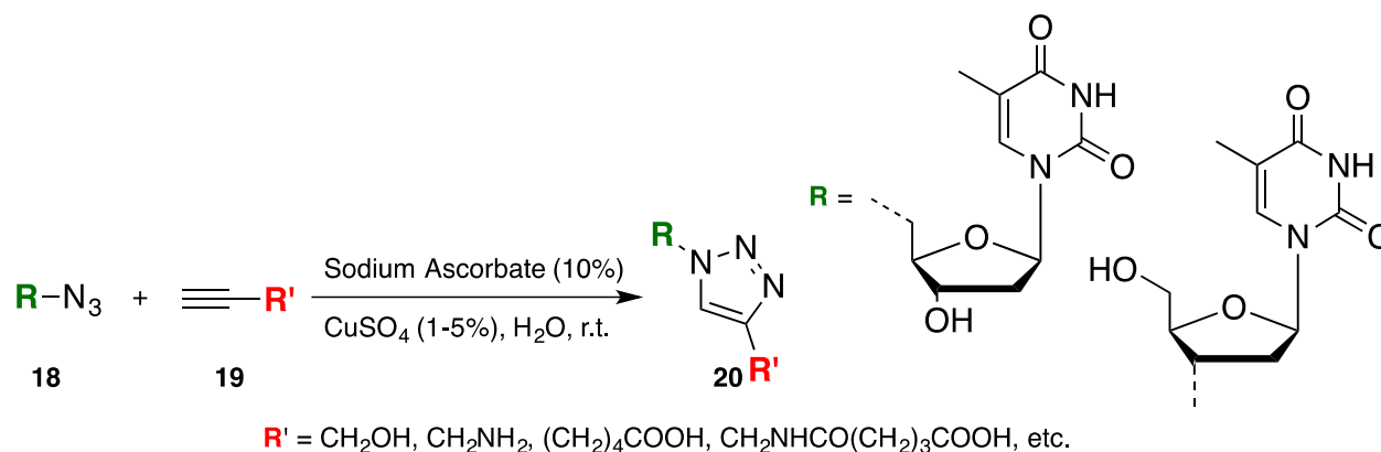
Scheme 8. Synthesis of thymidine analogues of type 20 .
