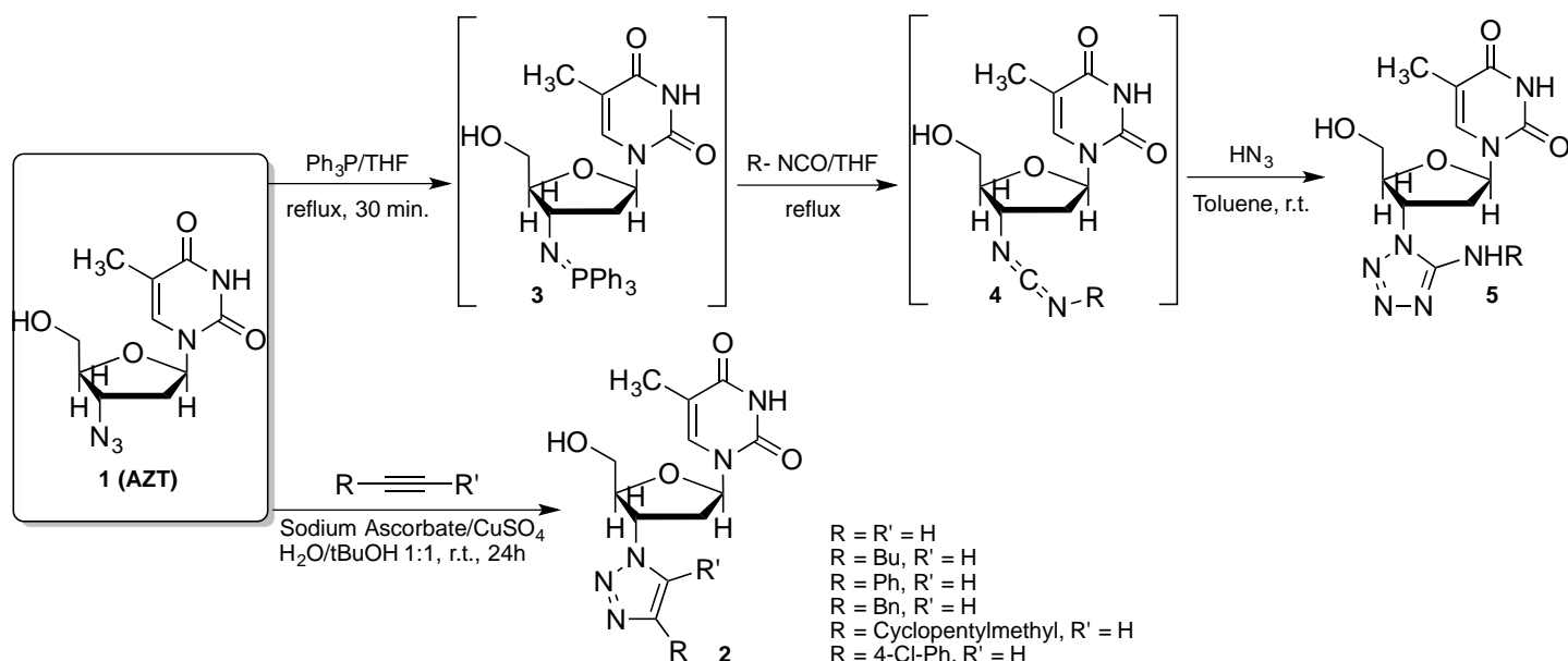
Scheme 3. Synthesis of tetrazolyl- and triazolyl-deoxythymidines.
