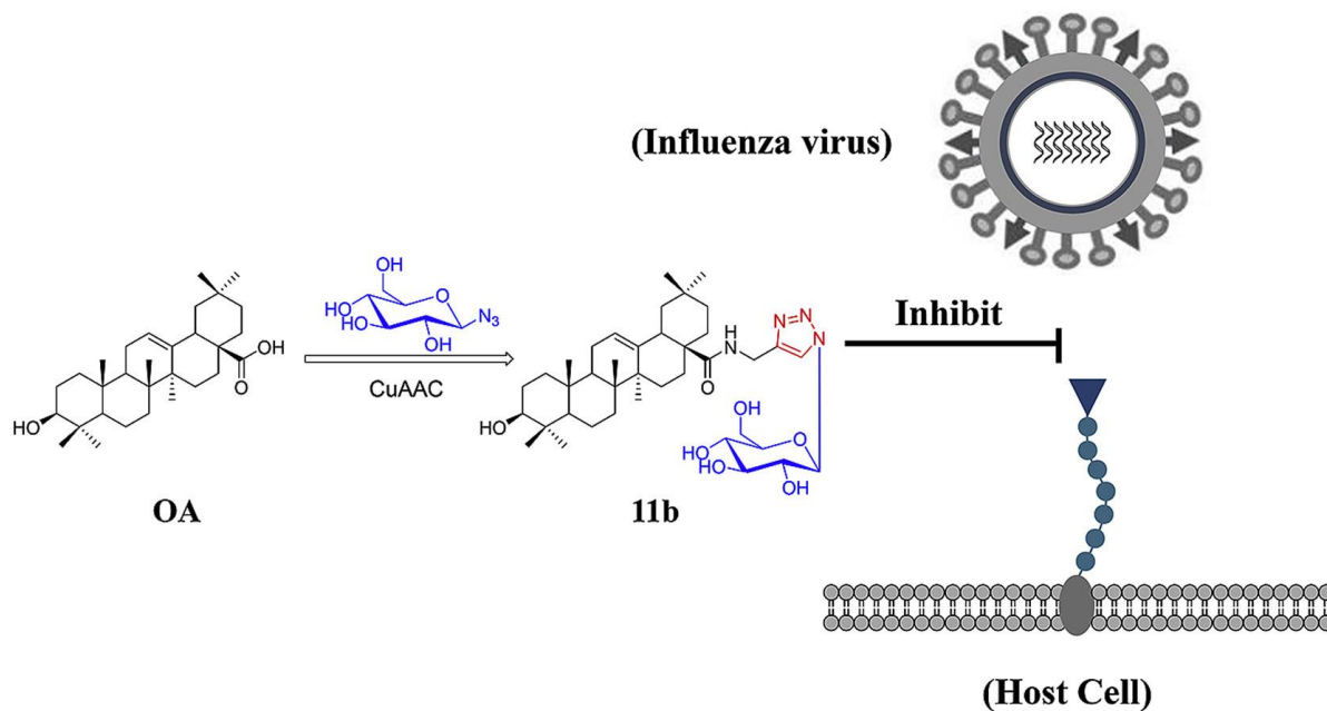
Figure 20. Synthetic strategy to oleanolic acid-saccharide conjugates (Reproduced with permission. 116 Copyright 2019, Elsevier).
