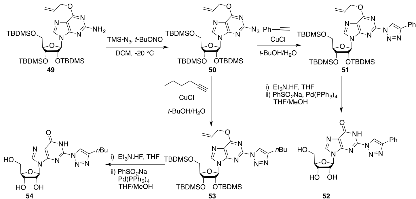
Scheme 19. Synthesis of nucleoside 54 .
