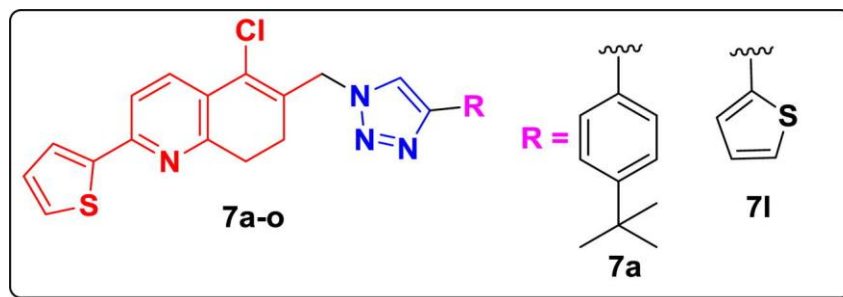
Figure 18. Structures of antitubercular agents (Reproduced with permission. 113 Copyright 2019, Elsevier).
