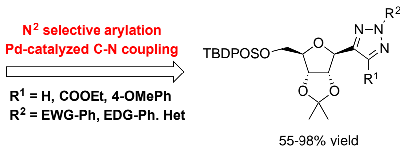
Figure 10. Functionalization strategy of the triazole ring (Reproduced with permission. 97 Copyright 2016, ACS).
