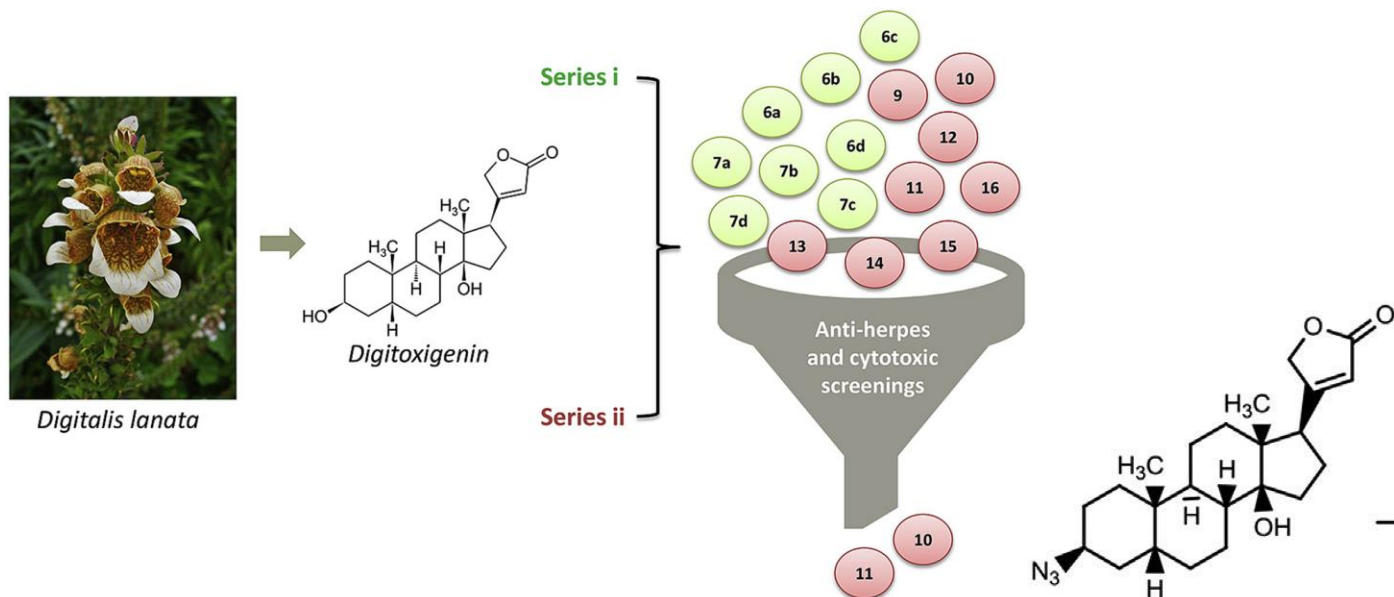
Figure 19. Source and structure of Digitoxigenin (Reproduced with permission. 115 Copyright 2019, Elsevier).
