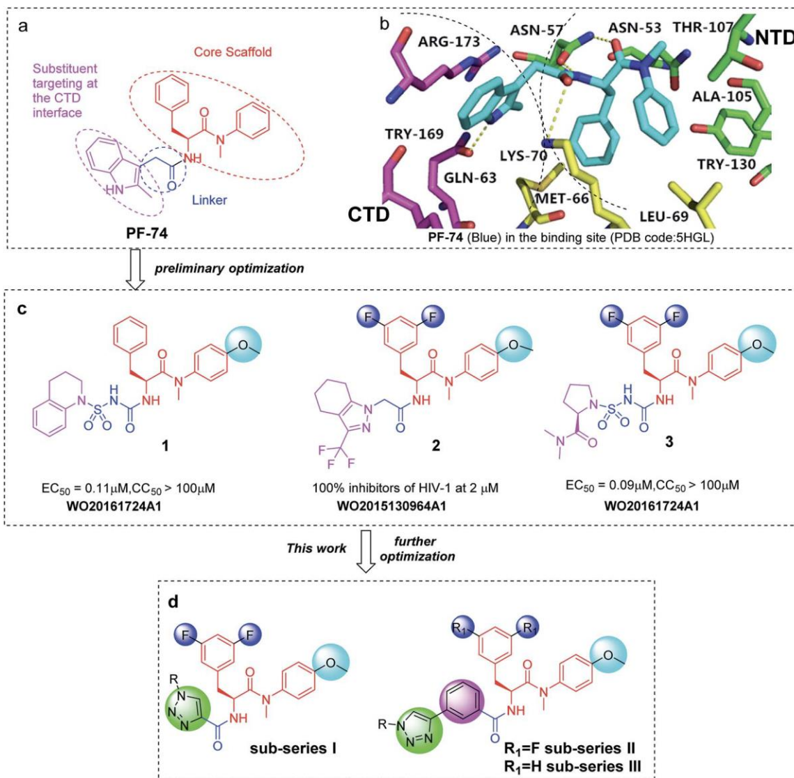
Figure 21. Design of novel phenylalanine derivatives as HIV-1 CA inhibitors: (a) Structure of PF-74; (b) the binding mode of PF-74 in the NTD-CTD interface of CA protein hexamer. Yellow dashed lines indicate H-bond interactions. (c) Phenylalanine derivatives as HIV-1 CA protein inhibitors. (d) Designed target compounds (Reproduced with permission. 119 Copyright 2019, RSC).
