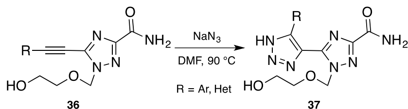
Scheme 14. Synthesis of bis-triazolyl acyclo-nucleosides 37 via Huisgen reaction using \text{NaN}_3 and various 5-alkynyltriazole acyclo-nucleosides 36 .
