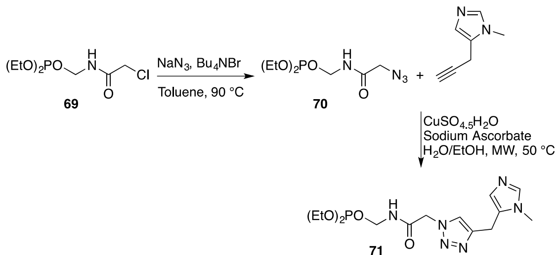
Scheme 25. Synthesis of [(1,2,3-triazol-1-yl)acetamido]-methylphosphonate 71 .
