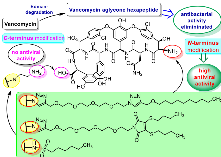
Figure 22. Synthetic strategy to the Vancomycin aglycone hexapeptide.
