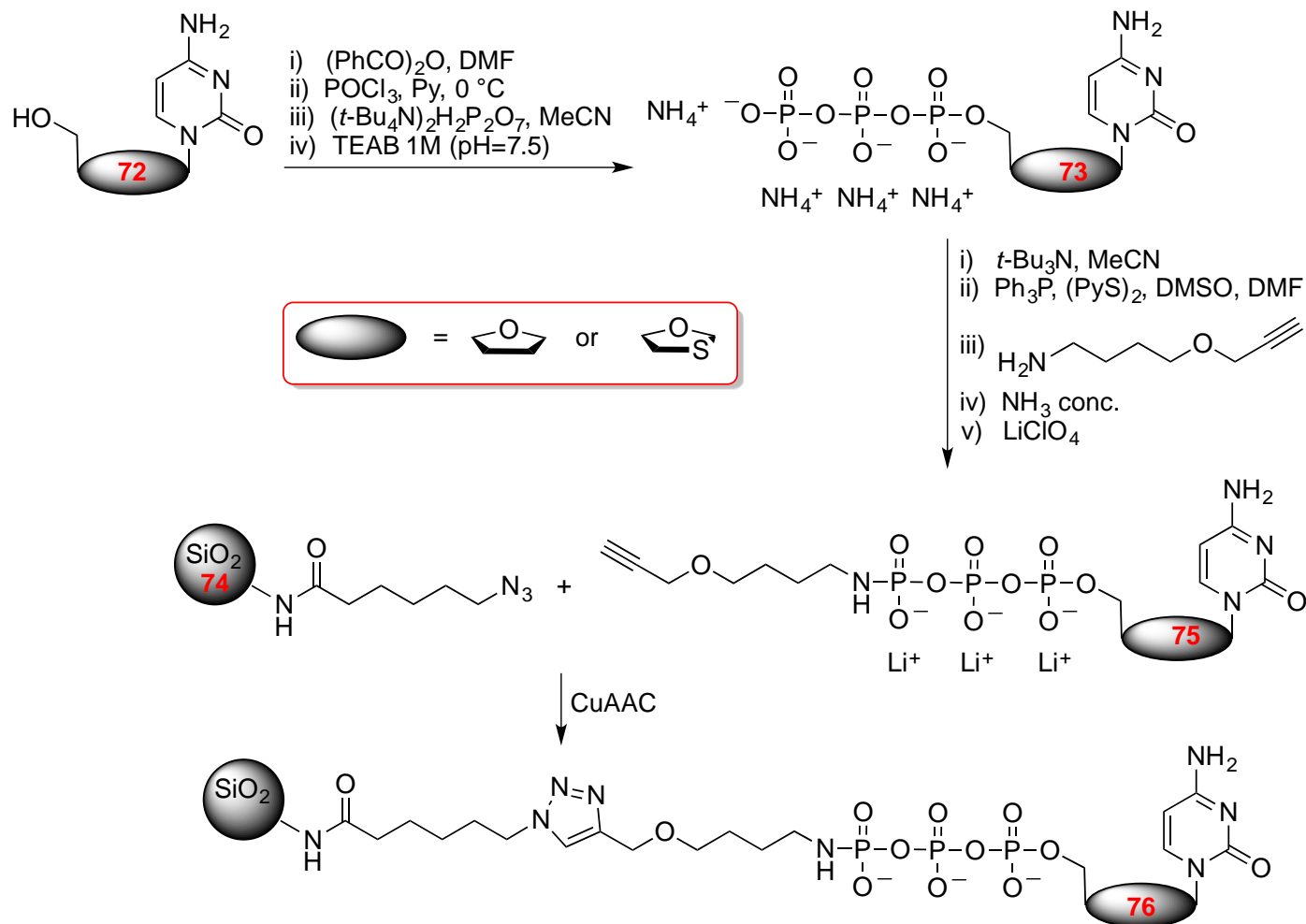
Scheme 26. \text{SiO}_2 nanoparticles synthesis.
