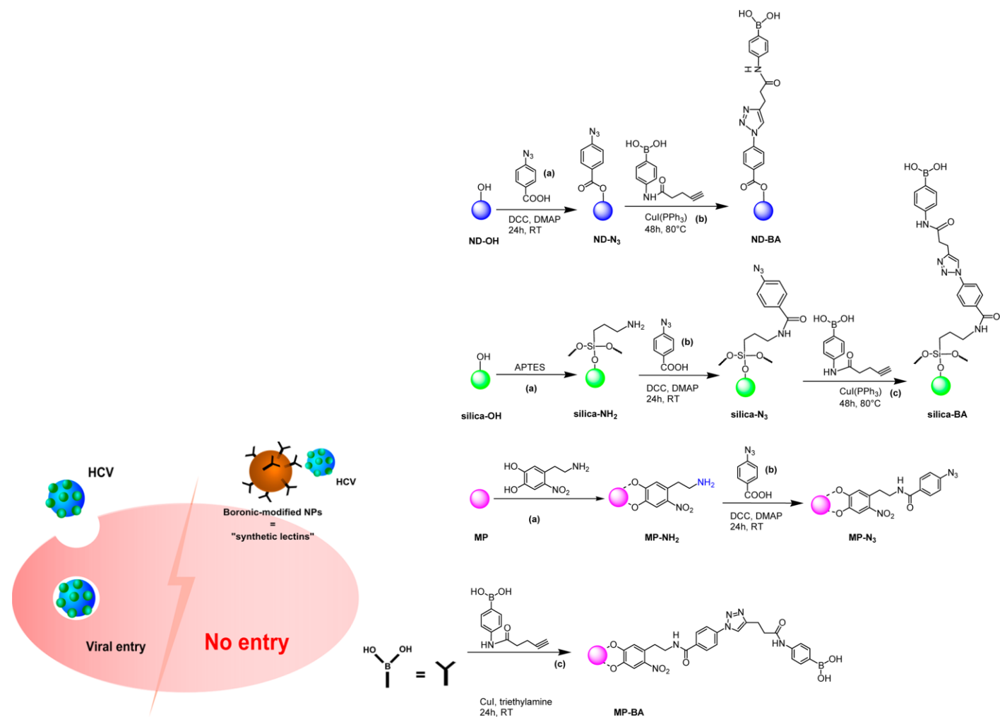
Figure 26. Mode of action of boronic-modified NPs (Reproduced with permission. 125 Copyright 2013, ACS).
