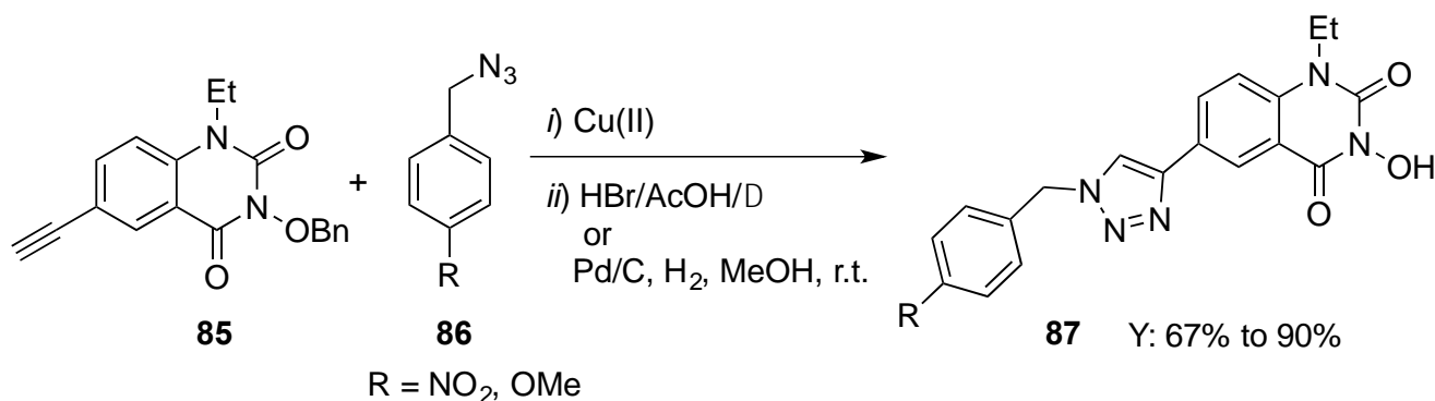
Scheme 29. Synthetic route to 3-hydroxy-quinazoline-2,4(1 H ,3 H )-diones.
