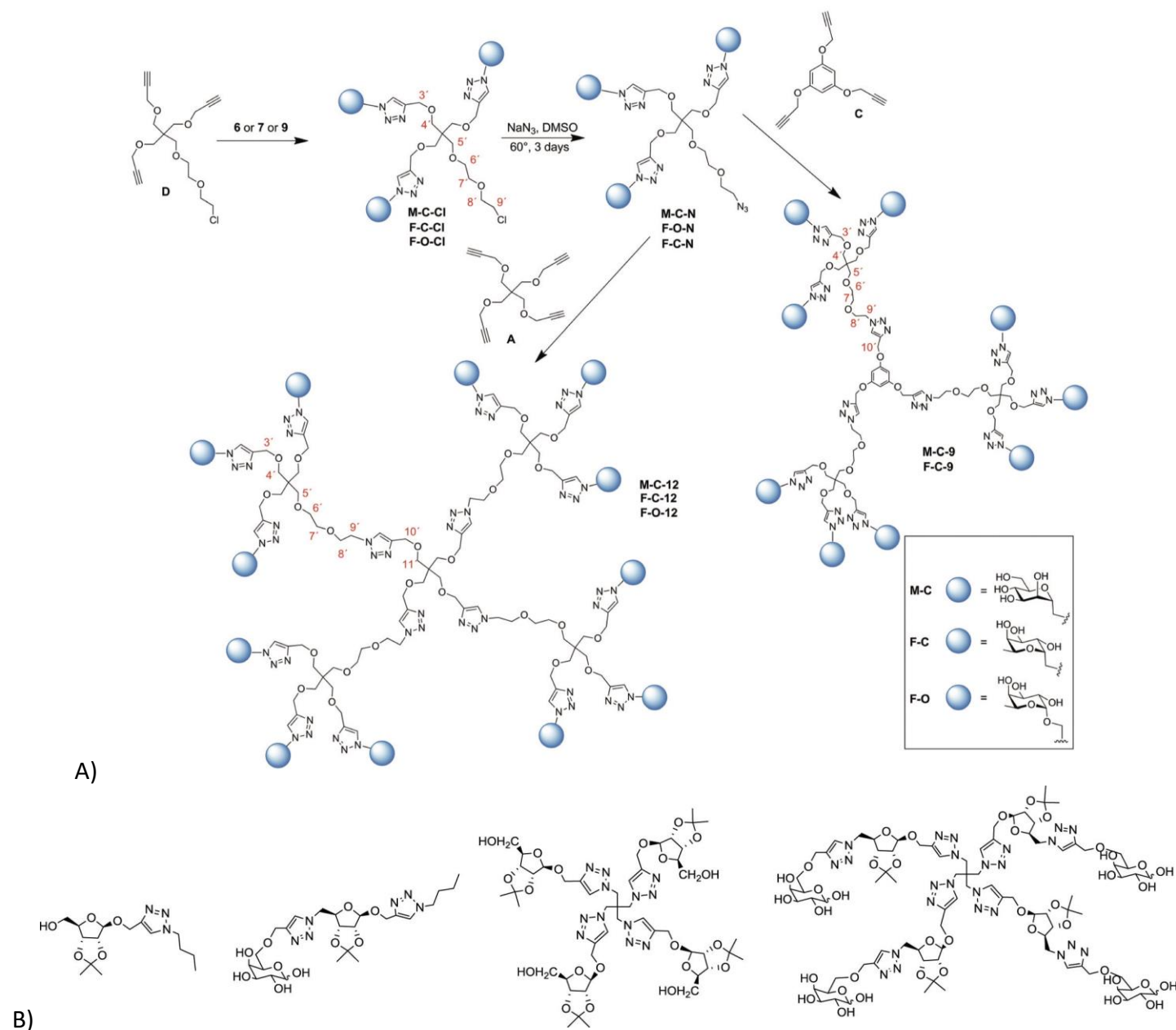
Figure 8. A) C-glycoside dendrimers decorated with 4, 6, 9, and 12 \alpha -L-fucopyranosyl units and with 9 and 12 \alpha -D-mannopyranosyl units. B) Ribavirin analogues incorporated into a multivalent arrangement.
