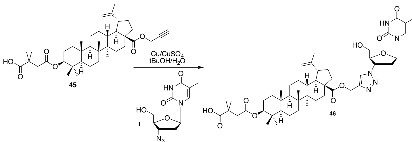
Scheme 17. Synthesis of AZT conjugates.
