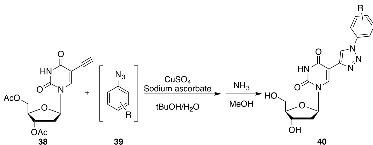
Scheme 15. Synthesis of C5-(1,4- and 1,5-disubstituted-1,2,3-triazolo)-nucleoside derivatives of type 40 .
