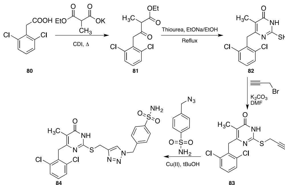
Scheme 28. Synthetic pathway to compound 84 .
