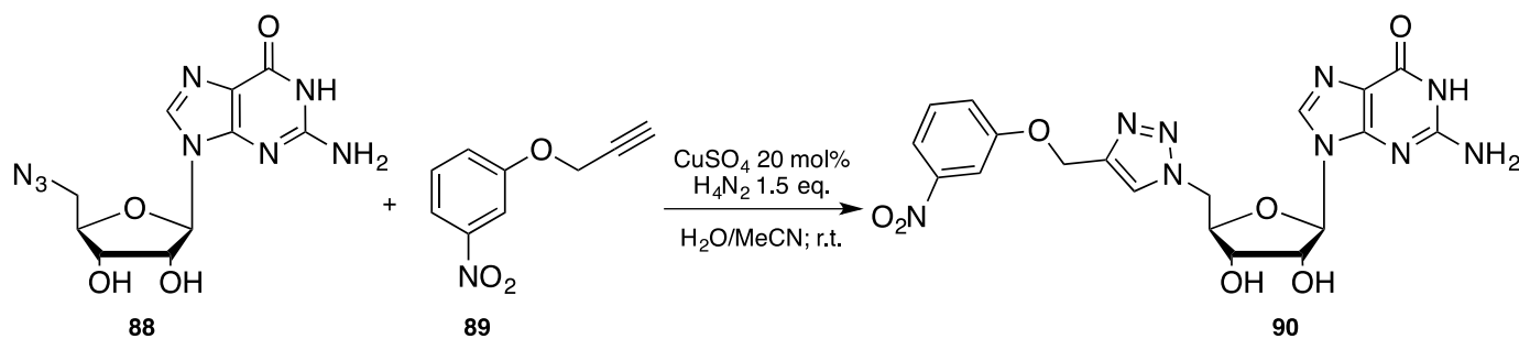
Scheme 30. Synthetic pathway to compound 90 .
