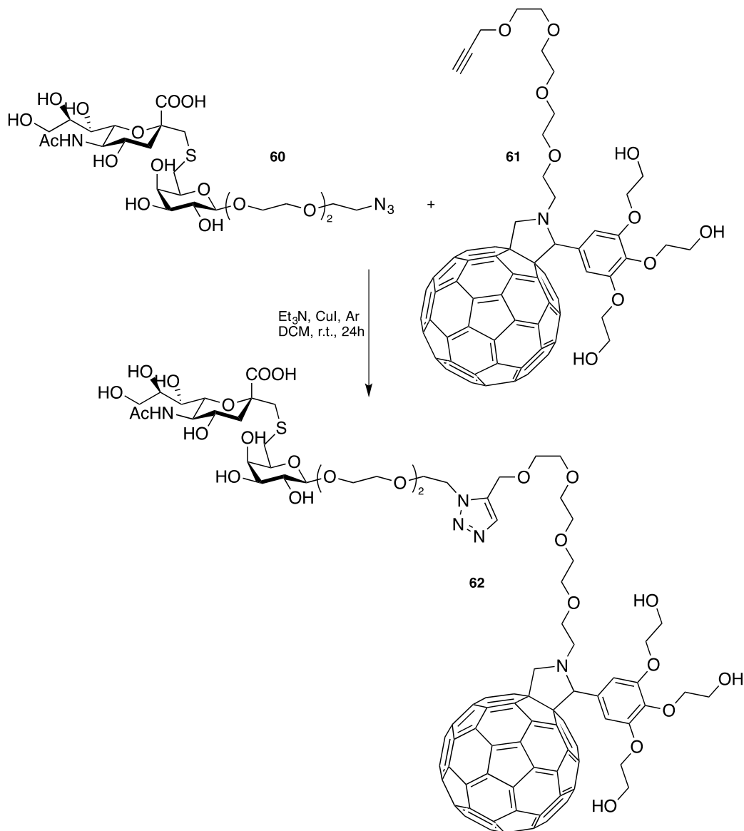
Scheme 22. Synthesis of compound 62 .
