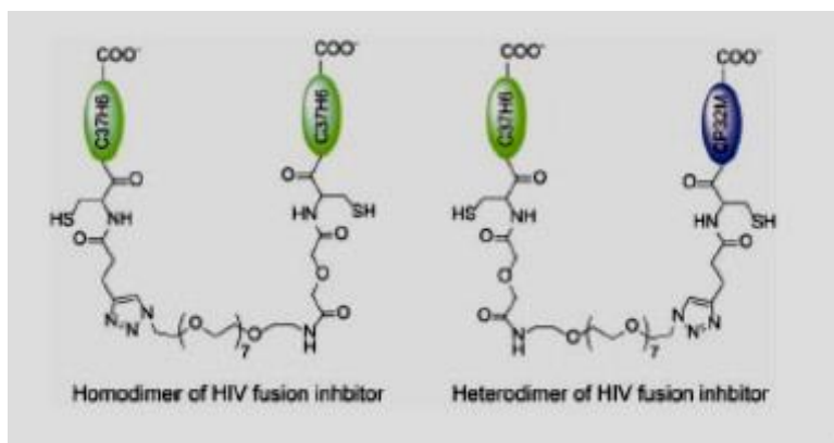
Figure 25. Structures of dimeric peptide derivatives (Reproduced with permission. 124 Copyright 2013, Elsevier).
