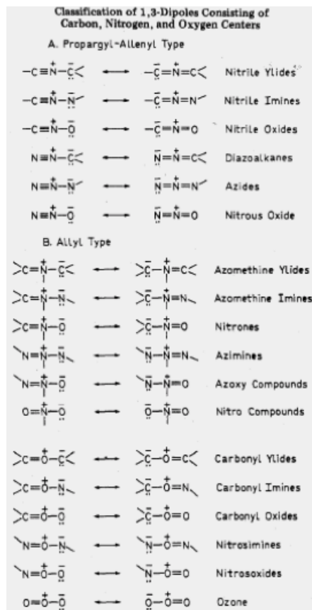
Figure 2. Classification of 1,3-dipoles (Reproduced with permission. 5 Copyright 1976, ACS).
