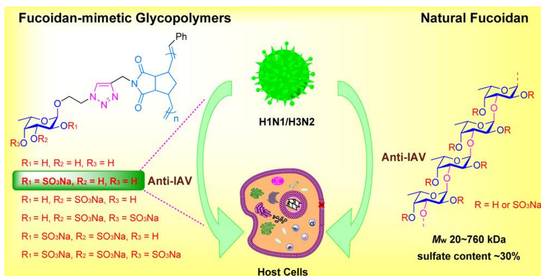
Figure 16. Fucoidan-mimetic glycopolymers structures and action mechanism (Reproduced with permission. 110 Copyright 2018, ACS).
