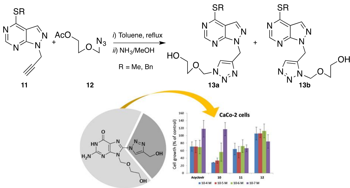
Scheme 6. Synthesis of regioisomeric 2-((4-(1 H -pyrazolo[3,4- d ]pyrimidin-1-yl)methyl)-1 H -1,2,3-triazol-1-yl)methoxy)ethan-1-ol derivatives ( 13 ).
