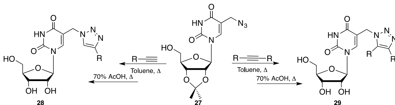
Scheme 11. Azidomethyl-uridine synthetic applications.
