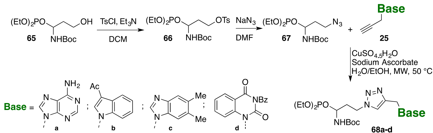
Scheme 24. Synthesis of derivatives 68 .
