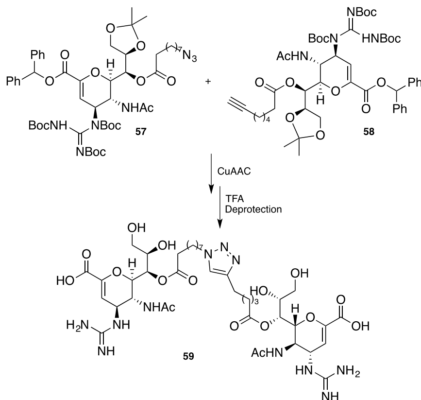
Scheme 21. Synthesis of dimer 59 .
