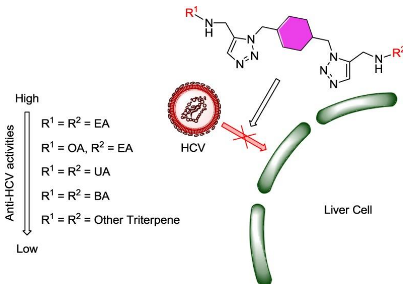
Figure 13. Inhibition scheme in HCV (Reproduced with permission. 106 Copyright 2017, Wiley).
