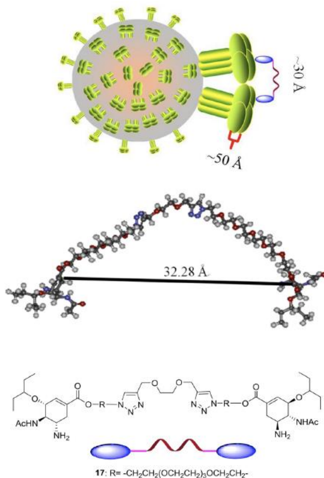
Figure 17. Schematic representation of distance between two NA monomer active sites on a same virion and the low-energy extended conformation of dimeric compound (Reproduced with permission. 112 Copyright 2019, Elsevier).
