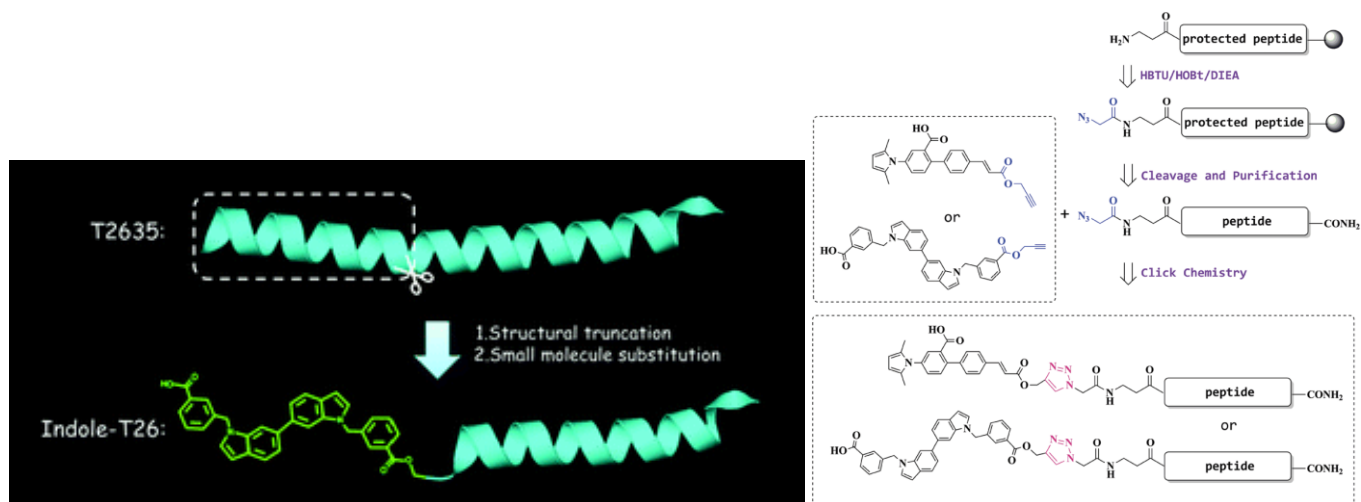
Figure 11. Truncation of peptide chain and strategy for the synthesis of small molecule–peptide conjugates (Reproduced with permission. 100 Copyright 2016, RSC).
