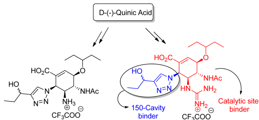
Figure 4. D-(-)-quinic acid strategy to triazole derivatives.
