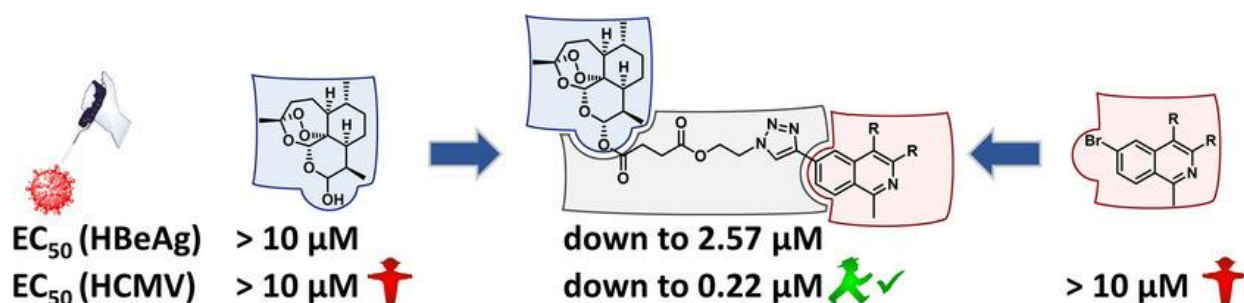
Figure 23. Isoquinoline derivatives structures and antiviral activities (Reproduced with permission. 122 Copyright 2020, Wiley).
