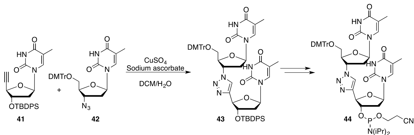
Scheme 16. Synthesis of the dinucleoside block 43 .
