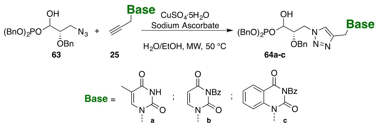
Scheme 23. Synthesis of analogues 64 .
