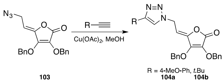
Scheme34. Synthesis of compounds 104a,b .
