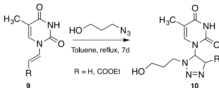
Scheme 5. Synthesis of the 1-[1-(3-hydroxypropyl)-4,5-dihydro-1 H -1,2,3-triazol-5-yl] -5-methylpyrimidine -2,4(1 H ,3 H )-dione derivatives ( 10 ).
