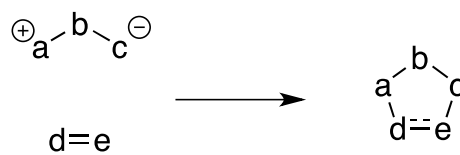
Scheme 1. Schematic representation of a 1,3-dipolar cycloaddition reaction.
