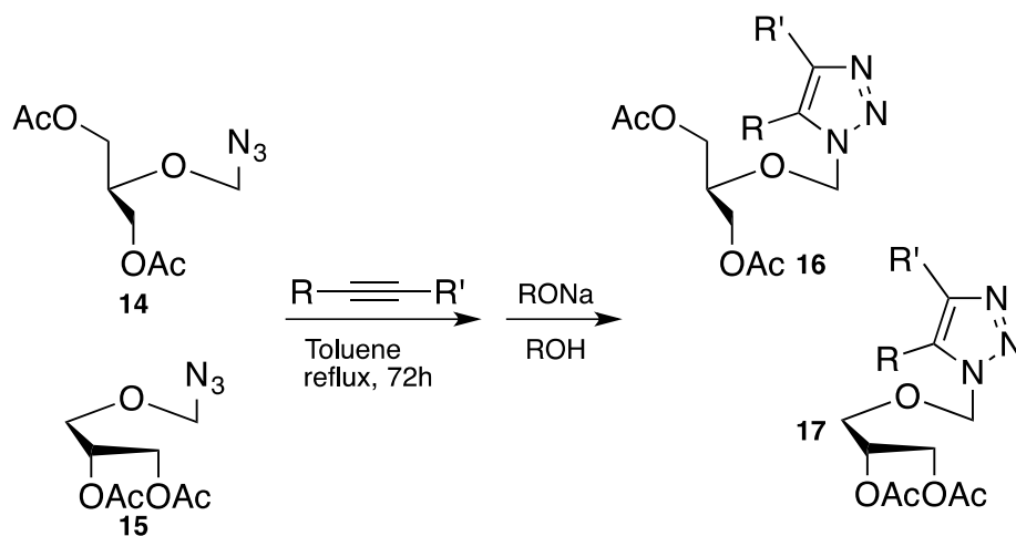
Scheme 7. Synthesis of 1,2,3-triazole acyclonucleosides.
