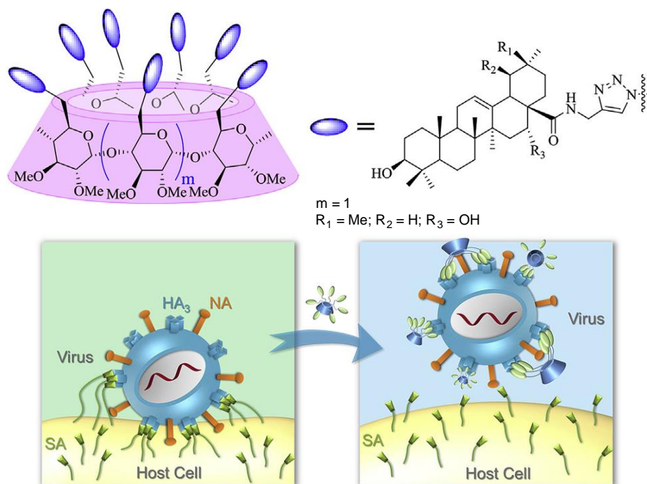
Figure 12. Cyclodextrin derivatives structures and anti-H1N1 inhibition scheme (Reproduced with permission. 101 Copyright 2017, Elsevier).
