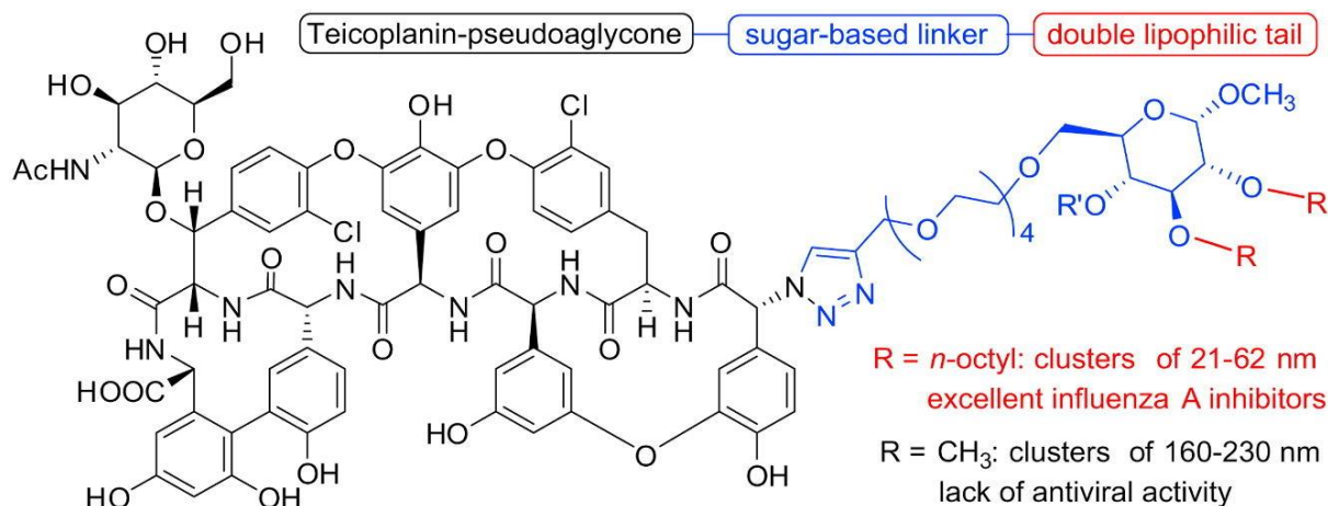
Figure 6. Teicoplanin pseudoaglycone derivatives (Reproduced with permission. 82 Copyright 2014, Elsevier).
