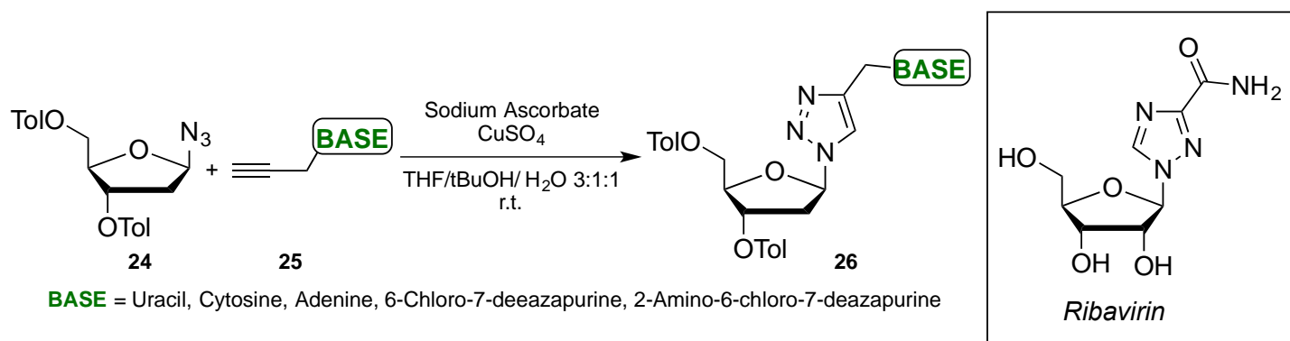
Scheme 10. Synthesis of 1,2,3-triazole nucleosides 26 .
