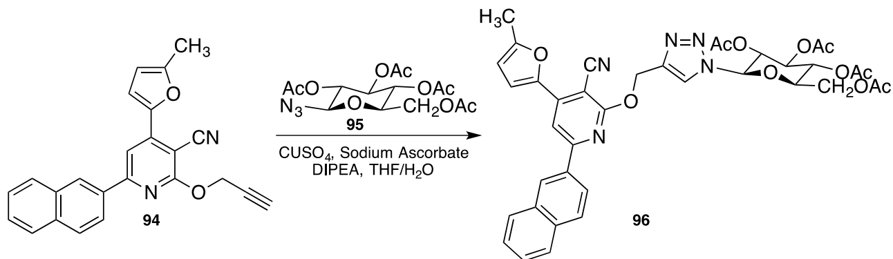
Scheme 32. Cu-catalyzed cycloaddition of azido-sugar.
