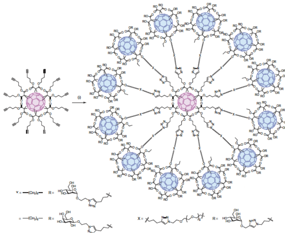
Figure 7. Syntheses of the tridecafullerenes using CuAAC click chemistry. The core fullerene (endowed with 12 alkyne groups) is joined to the peripheral fullerene-based compounds by click chemistry. Reagents and conditions: (i) CuBr·S(CH 3 ) 2 , sodium ascorbate, Cu(0), DMSO, 25 °C, 48 hours, 73-79%; (ii) CuSO 4 ·5H 2 O, sodium ascorbate, THF/H 2 O, 80 °C (MW), two hours, 76%.
