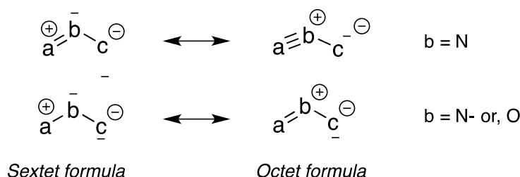
Figure 1. Sextet and octet structures of 1,3-dipoles.
