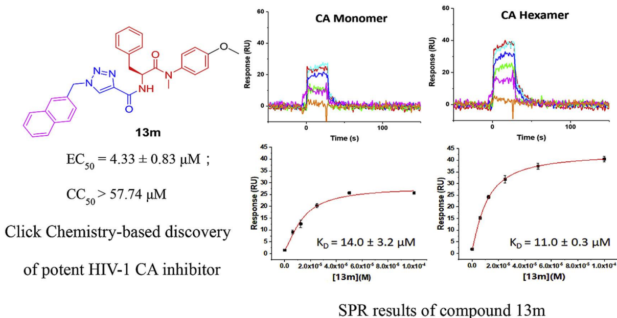
Figure 15. Structure of active compound and activity data (Reproduced with permission. 109 Copyright 2018, Elsevier).
