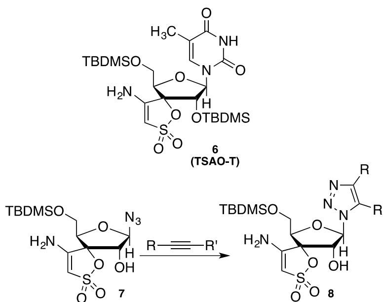
Scheme 4. Synthesis of triazole-TSAO derivatives 8 .
