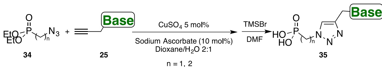
Scheme 13. Triazoloacyclic nucleoside phosphonates synthesized through the CuAAC reaction.
