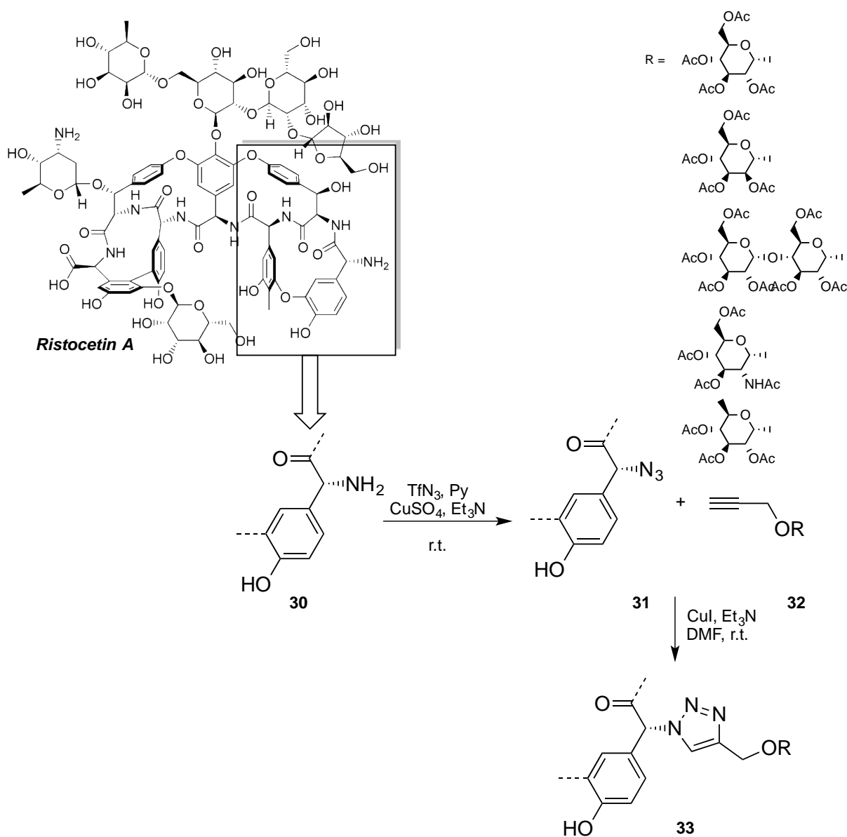
Scheme 12. Synthesis of triazole derivatives of ristocetin aglycon.
