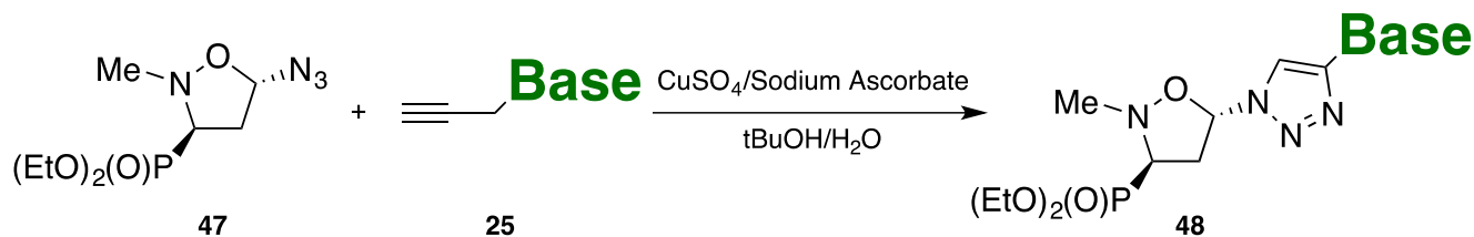
Scheme 18. 1,3-Dipolar cycloadditions of the 5-azidoisoxazolidines 47 with propargylated nucleobases 25 .
