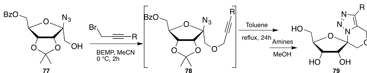
Scheme 27. Synthesis of spiro-compound 79 .
