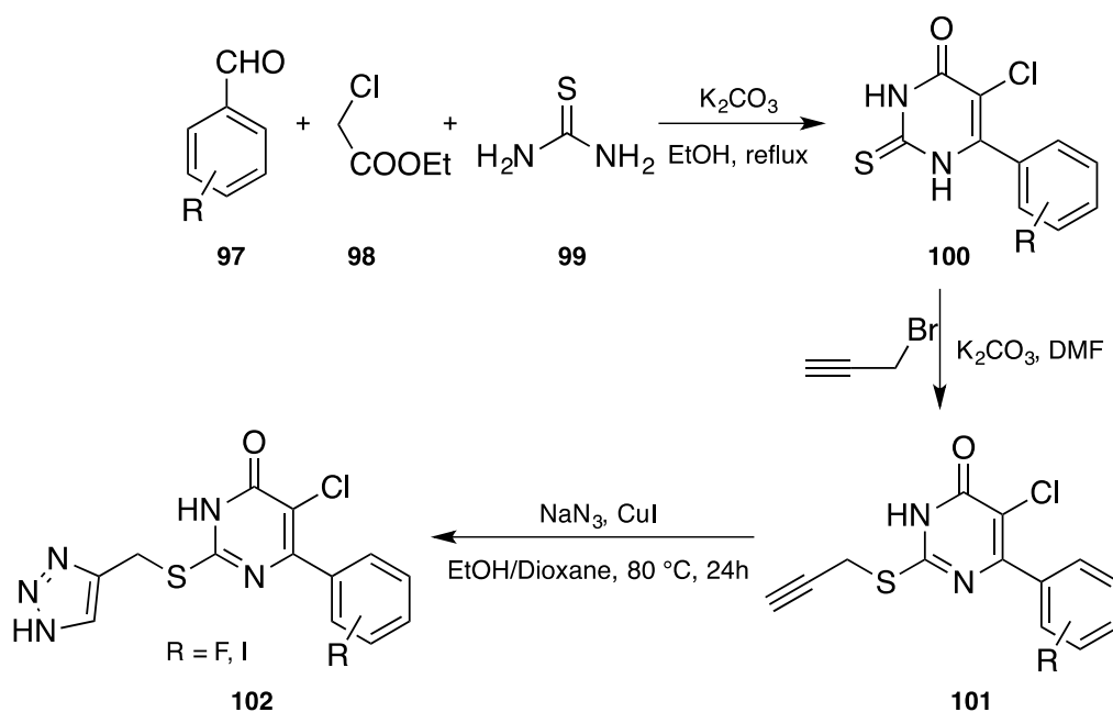
Scheme 33. Synthesis of 2-[(1H-1,2,3-triazol-4-yl)methylthio]-5-chloro-6-phenylpyrimidin-4-(3H)-one derivatives 102 .
