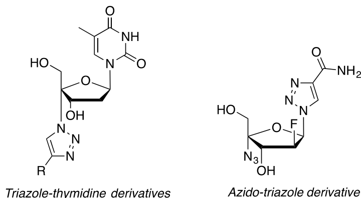
Figure 5. Structures of Triazole-thymidine and Azido-triazole derivatives.
