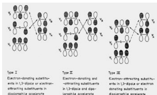
Figure 3. The HOMO-LUMO interactions between 1,3-dipoles and dipolarophiles (Reproduced with permission. 6 Copyright 1984, Wiley).
