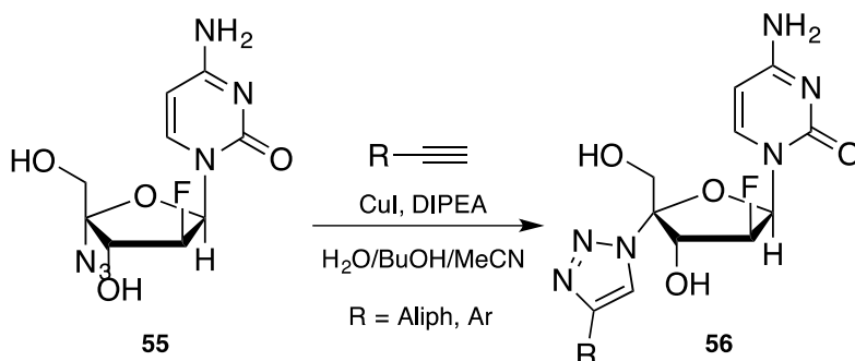
Scheme 20. Synthesis of 4'-[1,2,3]triazole-2'-deoxy-2'-fluoro- \beta -D-arabinofuranosylcytosines of type 56 .
