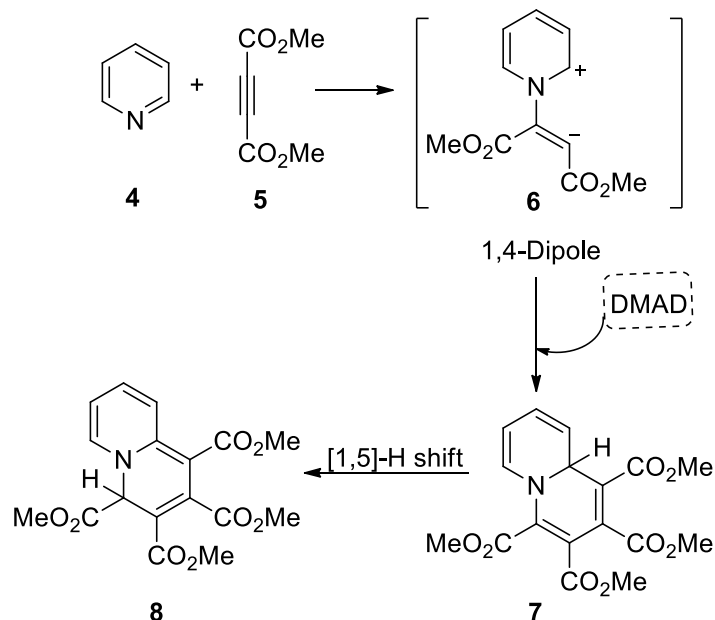
Scheme 1. Cascade reaction of pyridine with DMAD.
