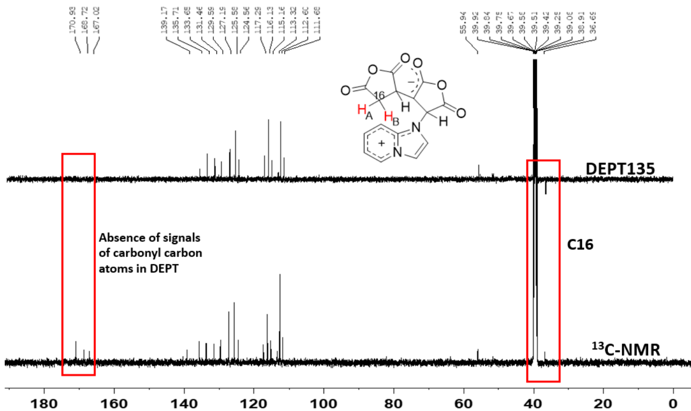
Figure 4. 13 C NMR spectrum of 16 and its DEPT 135 version.
