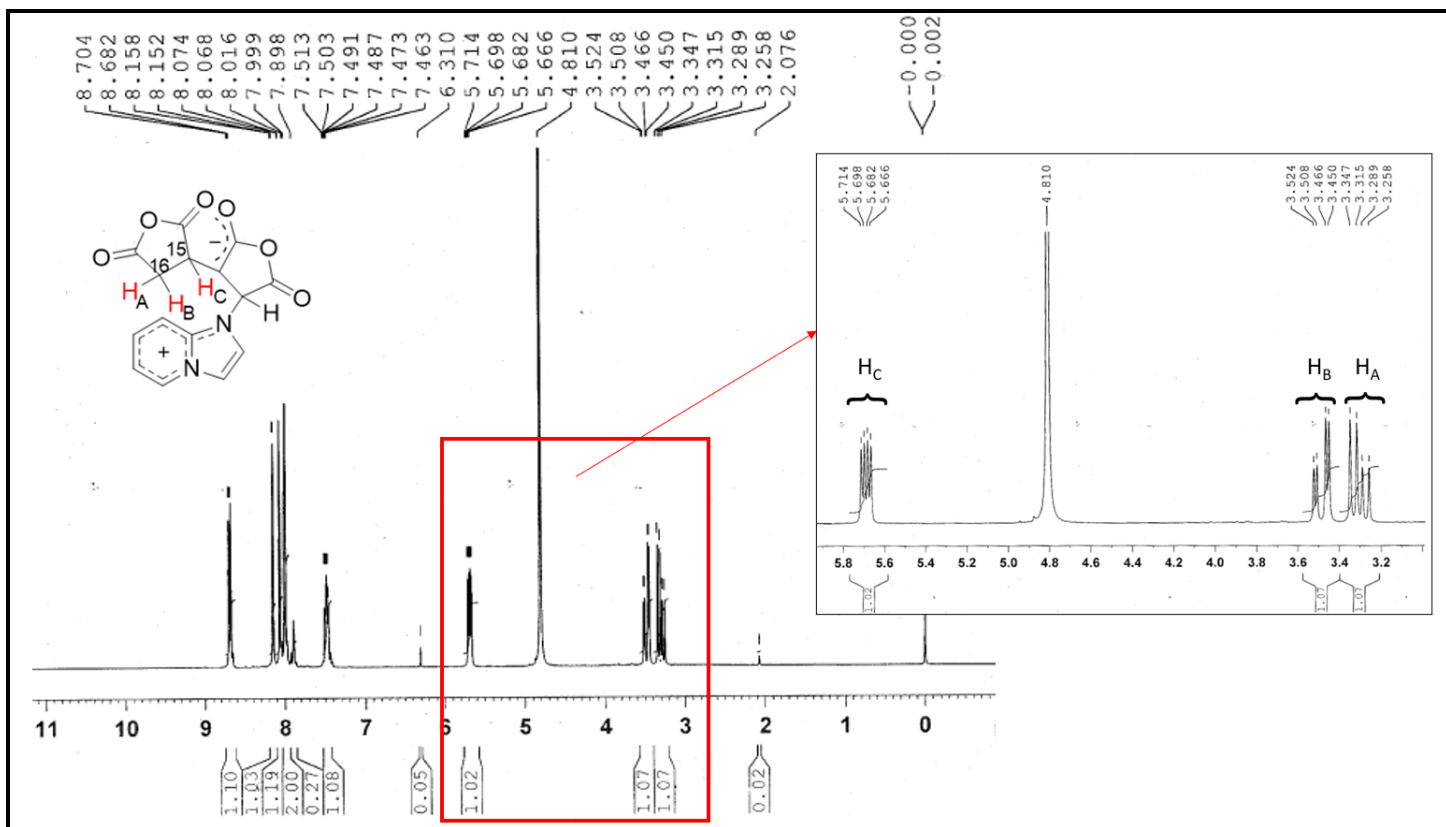
Figure 3. 1 H NMR spectrum of the product 16 depicting the ABC spin system.
