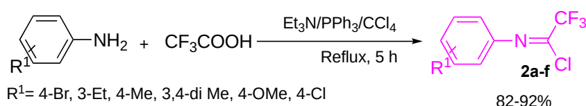
Scheme 1. Preparation of 2,2,2-trifluoroacetimidoyl chlorides 2a-f .
