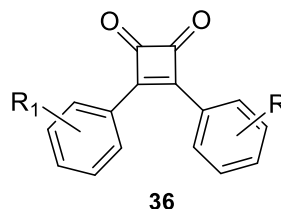
Figure 9. General formula of cyclobutenedione derivatives.
