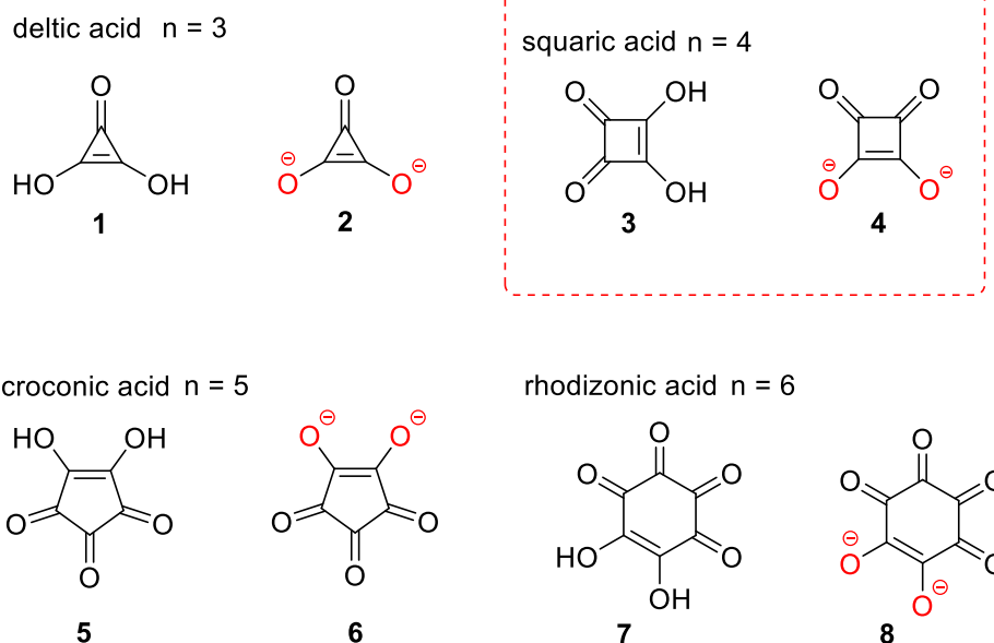
Figure 1. Chemical structures of oxocarbon acids and their dianions.
