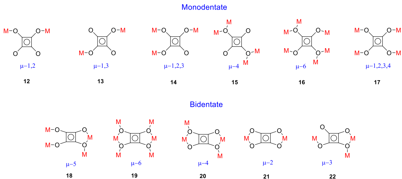
Figure 5. Schematic representations of all coordination modes of squarate dianion.
