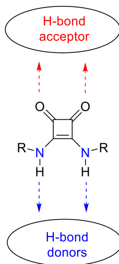
Figure 6. Representation of the possible hydrogen bonding sites in squaramides.
