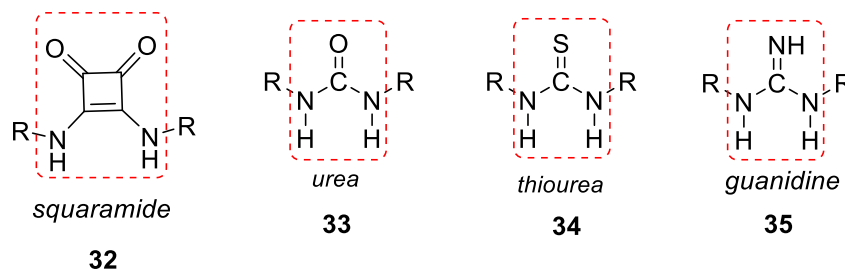
Figure 8. Squaramides as bioisosters.
