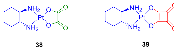
Figure 11. Chemical formulas of cis -[Pt(dach)(C 2 O 4 )] and cis -[Pt(dach)(SA)].
