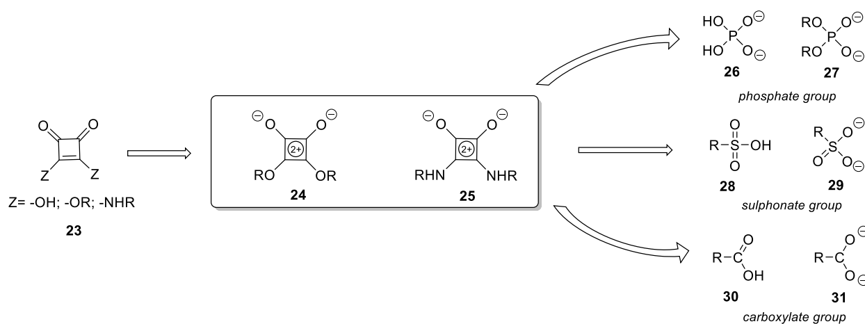
Figure 7. Squaric acid and its derivatives as bioisosteres.
