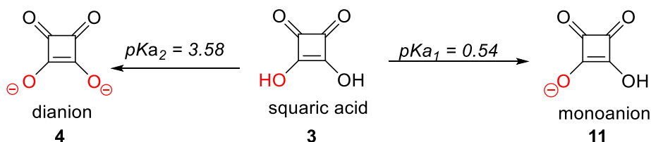
Figure 3. Squaric acid and its mono- and dianion.
