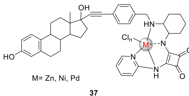
Figure 10. Estrogen-derived steroidal metal complexes.
