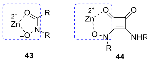
Figure 14. Structures of zinc hydroxamate and zinc hydroxamate squarate.
