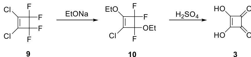
Figure 2. Synthesis of squaric acid by Cohen et al.
