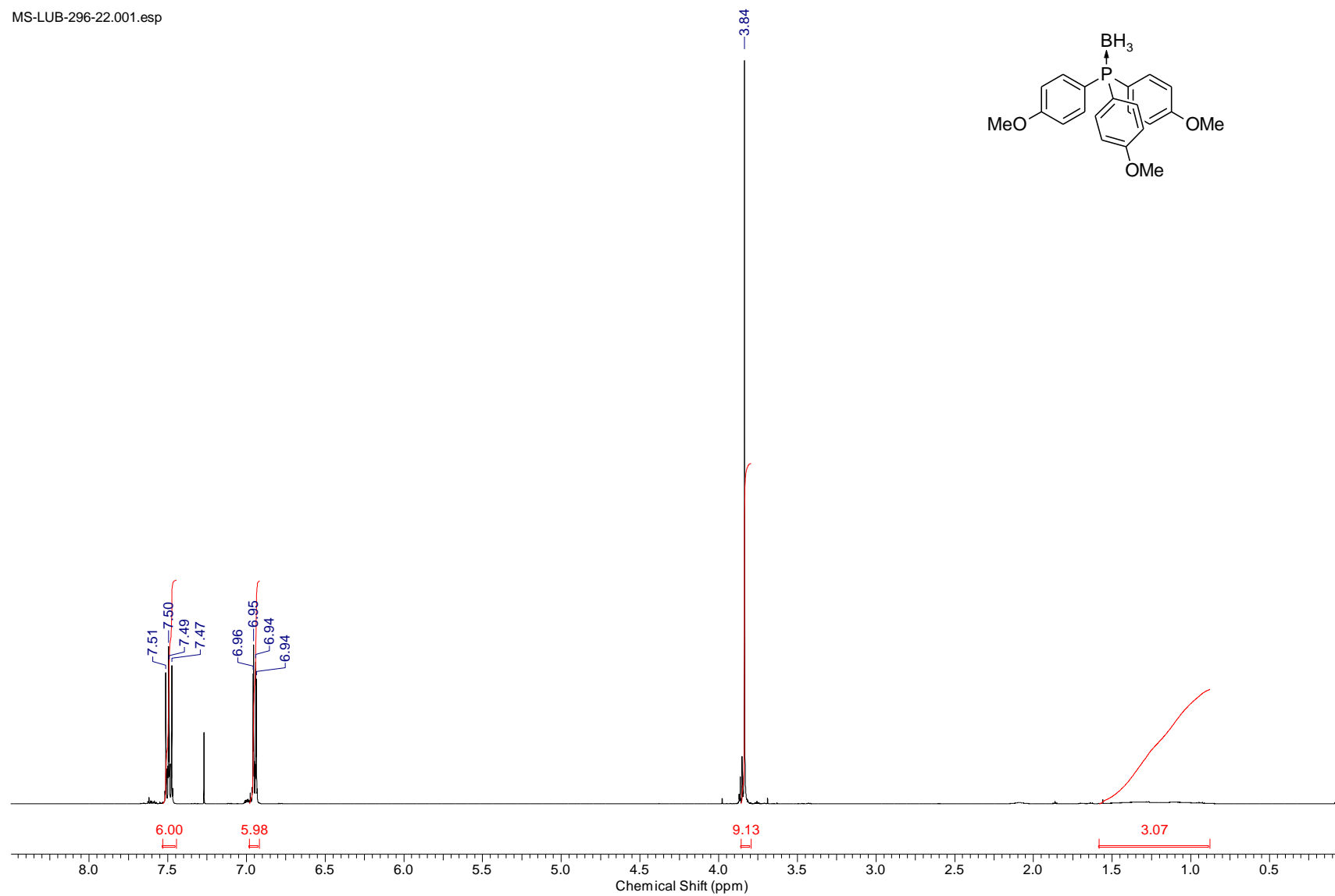
S16. ^1\text{H} NMR spectrum of tri( p -anisyl)phosphine-borane 30 (500 MHz, \text{CDCl}_3 )
