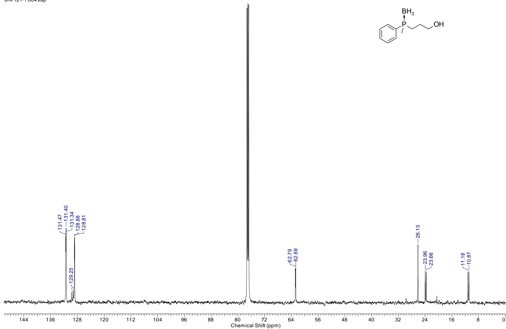
S2. ^{13}\text{C} NMR spectrum of (3-hydroxypropyl)methylphenylphosphine-borane 20 (126 MHz, \text{CDCl}_3 )
