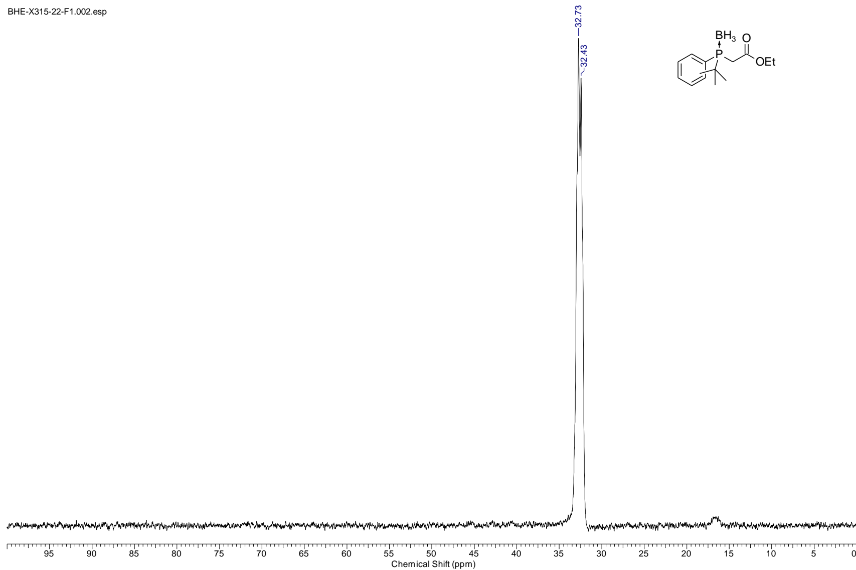
S15. ^{31}\text{P} NMR spectrum of ethyl ( t -butylphenylboranatophosphinyl)acetate 29 (202 MHz, CDCl 3 )
