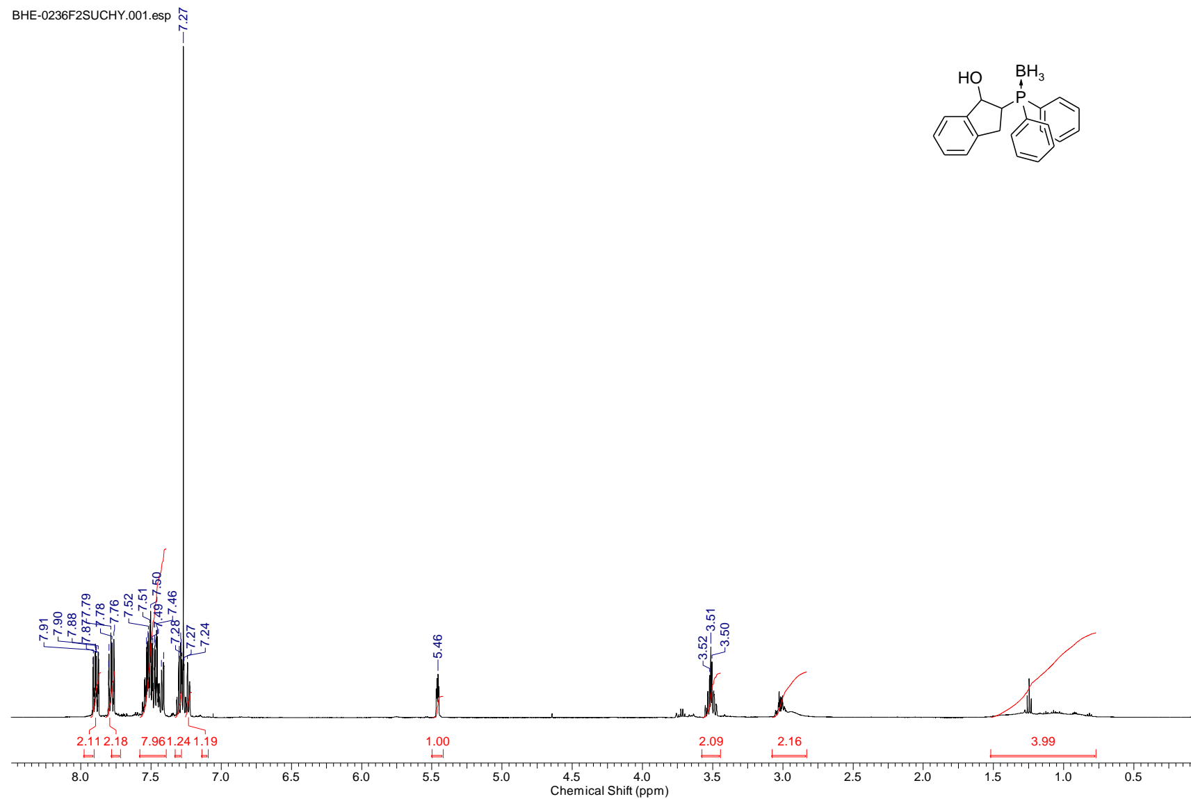
S10. ^1\text{H} NMR spectrum of 2-(diphenylboranatophosphinyl)-1-indanol 28 (500 MHz, \text{CDCl}_3 )
