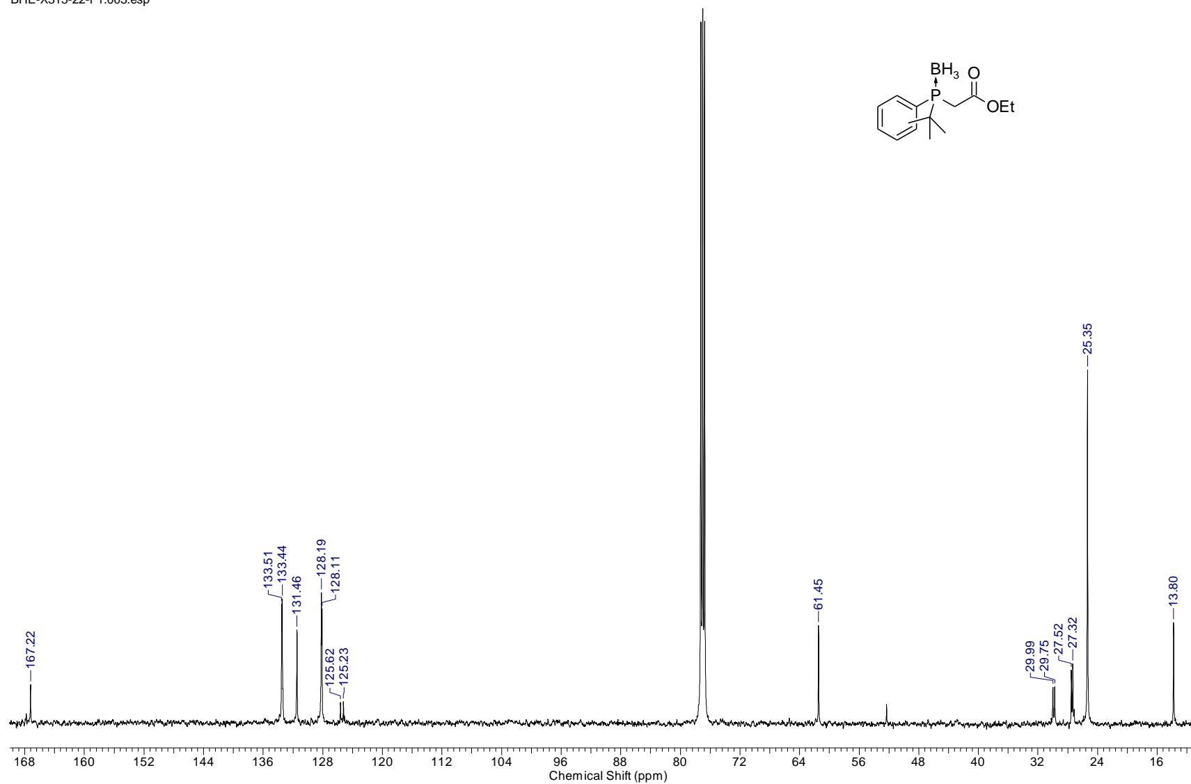
S14. 13 C NMR spectrum of ethyl ( t -butylphenylboranato-phosphinyloxy)acetate 29 (126 MHz, CDCl 3 )
