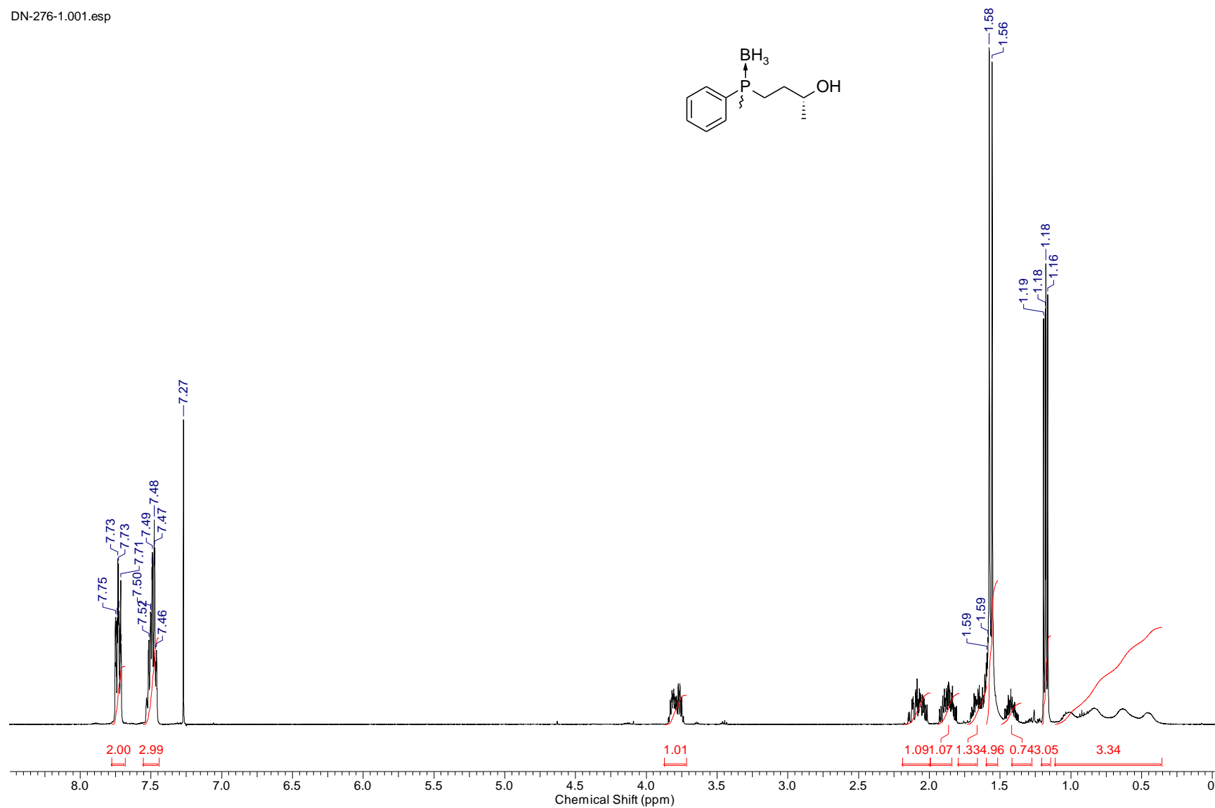
S4. 1 H NMR spectrum of ((3 R )-3-hydroxybutyl)methylphenylphosphine-borane (mixture of diastereomers) 21 (500 MHz, CDCl 3 ).
