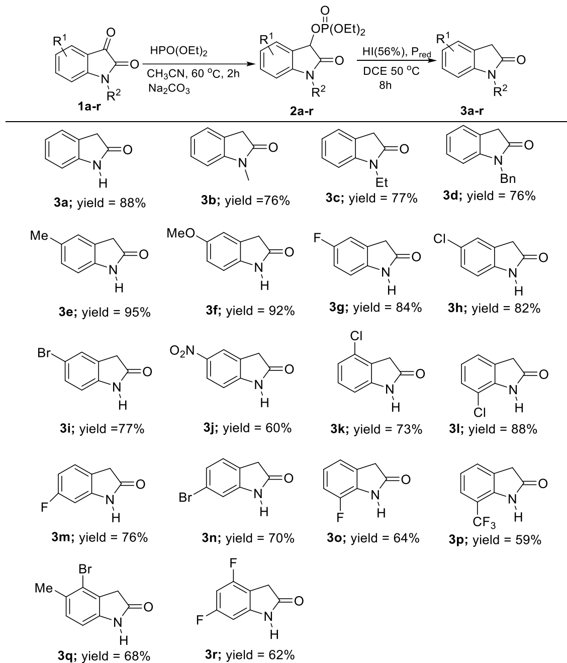
Scheme 2. Substrate scope of the reductive dephosphorylation of phosphates 2 a
