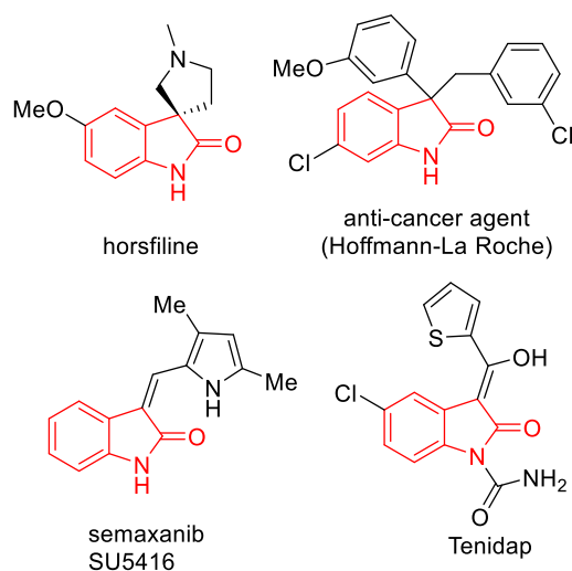
Figure 1 Pharmaceutically relevant oxindoles
