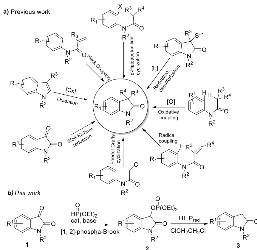
Scheme 1 Methods for the synthesis of oxindoles
