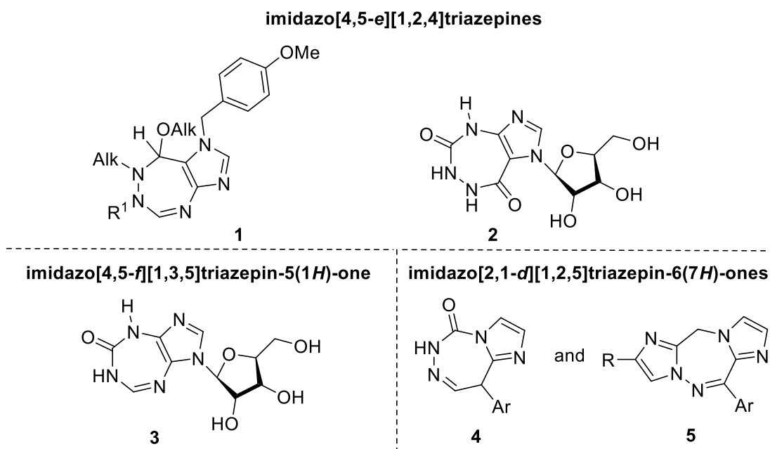
Figure 1. Examples of biologically active imidazotriazepine frameworks
