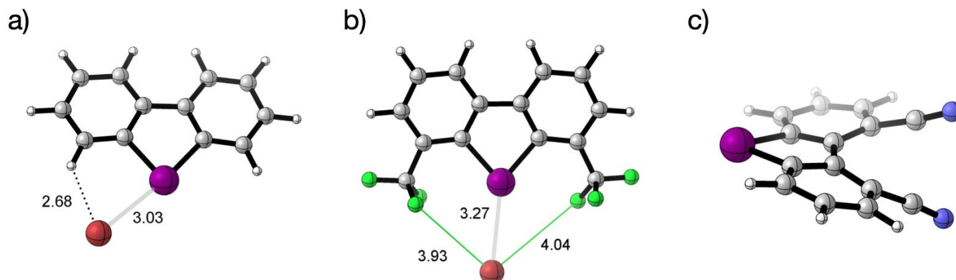
Figure 4. a) Binding of bromide to the unfunctionalized iodolium cation 1 H ; b) Binding of bromide to the sterically blocked 1,8-bis(trifluoromethyl)iodolium cation 8 CF 3 ; c) Distortion of the 4,5-dicyanoiodolium cation 5 CN .
