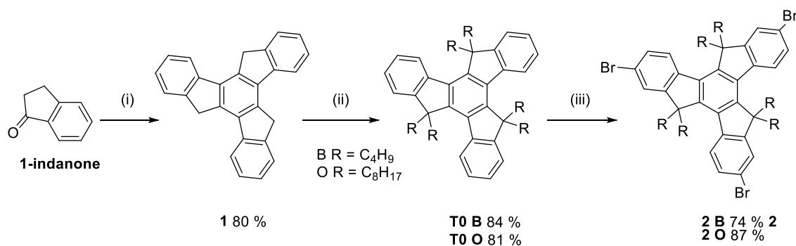
Scheme 1. Synthesis of the truxene core. Reagents and conditions: (i) CH 3 COOH, HCl, 100°C, 16 h; (ii) (1) n -BuLi/THF (0°C), (2) RBr, (3) R.T., 18 h; (iii) Br 2 /CH 2 Cl 2 (R.T.), 12 h.
