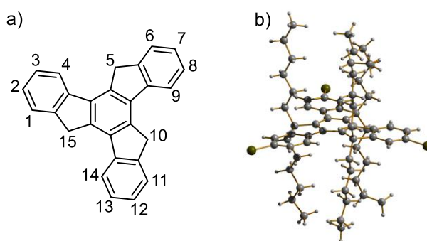
Figure 1. Numbering of the truxene fused system (a) and the orthogonal positions of hexyl substituents in tribromohexahexyltruxene (b).
