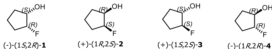
Scheme 3. Chiral 2-fluorocyclopentan-1-ols
