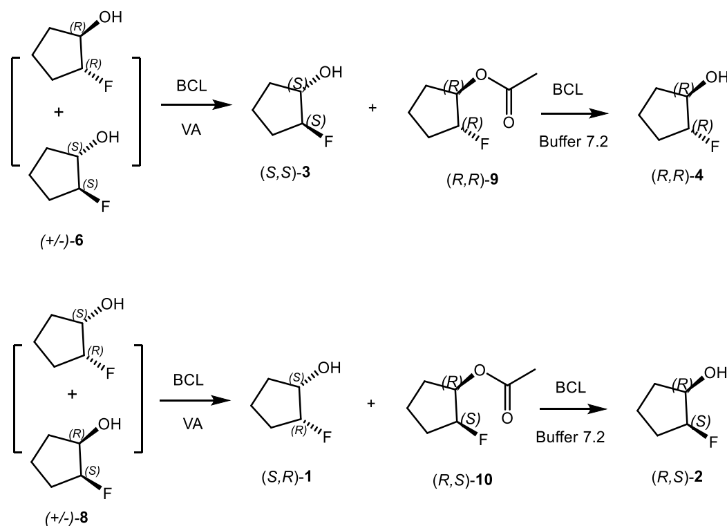
Scheme 6. Enzymatic deracemization of 2- cis - and trans -fluorocyclopentanols 6,8
