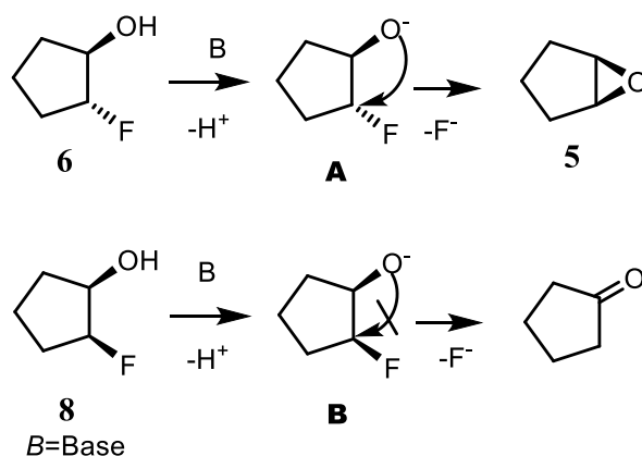
Scheme 5. Base-mediated reaction of cis - and trans -fluorocyclopentan-1-ols
