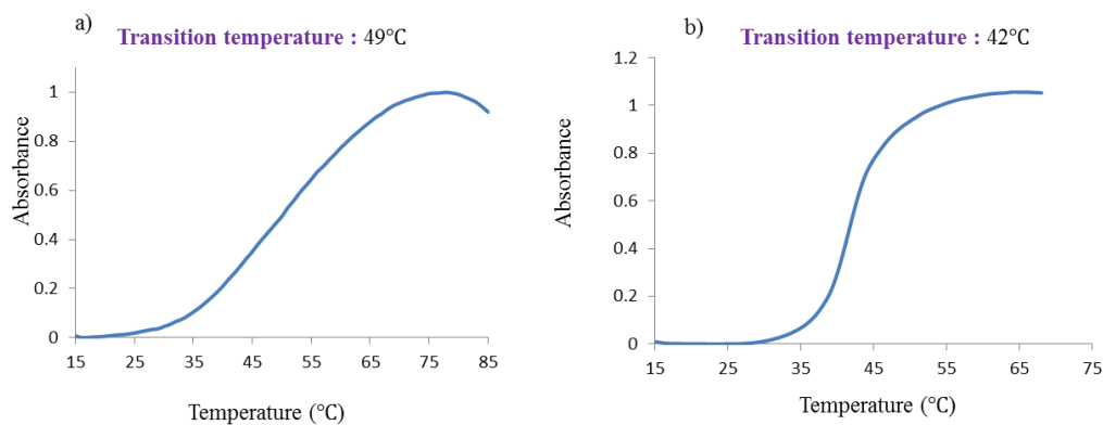
Figure S17: Turbidity measurements of polymer solutions (1 mg mL -1 ) as observed by UV-Vis absorbance at 300 nm: (a) PF75-VPGVG-NH 2 and (b) PF100-VPGVG-NH 2 .
