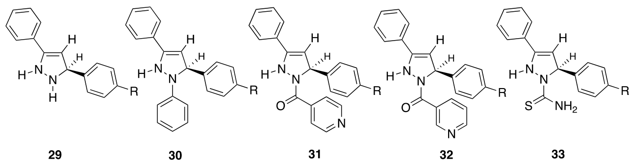
Figure 5. Swarnkar's 3-pyrazolines.
