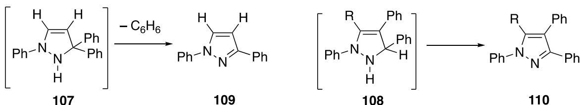
Scheme 29. Synthesis of pyrazoles 110 from sydnone.
