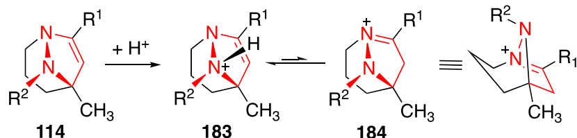
Scheme 48. Possible result of the protonation of 3-pyrazoline 114 .
