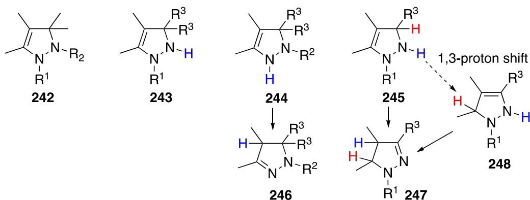
Scheme 58. The 3- to 2-pyrazoline isomerization channels.
