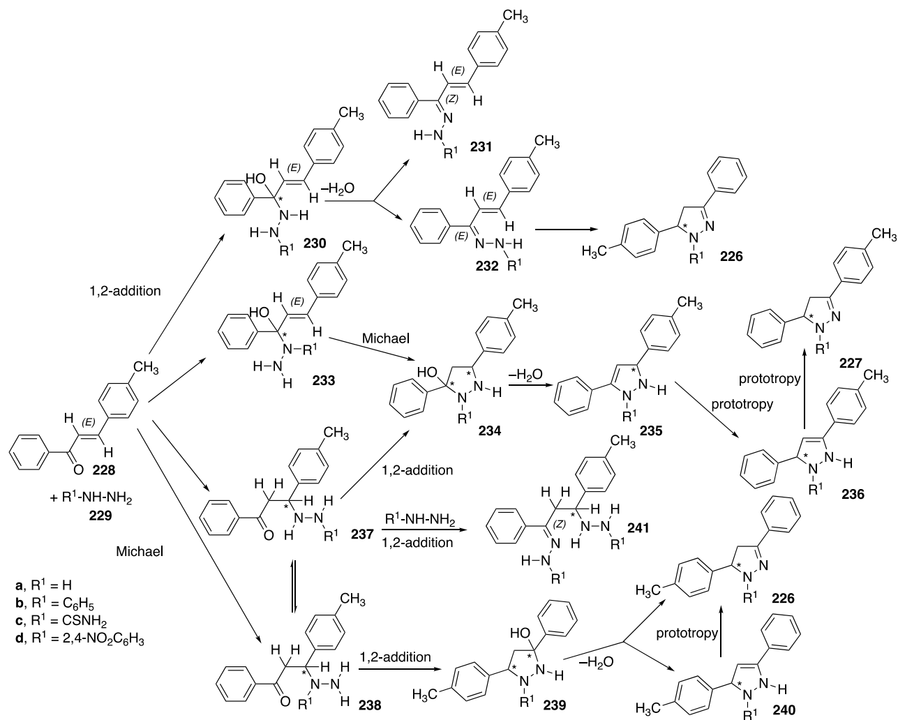
Scheme 57. Different mechanisms for the formation of 2-pyrazolines 226 and 227 .
