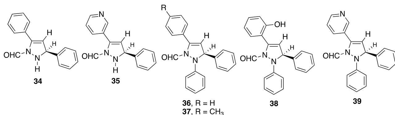
Figure 6. Jeti's 3-pyrazolines.
