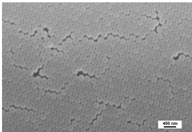
Figure 1. SEM image of the poly(St-co-NaSS) particles, showing their uniform size and crystalline packing.
