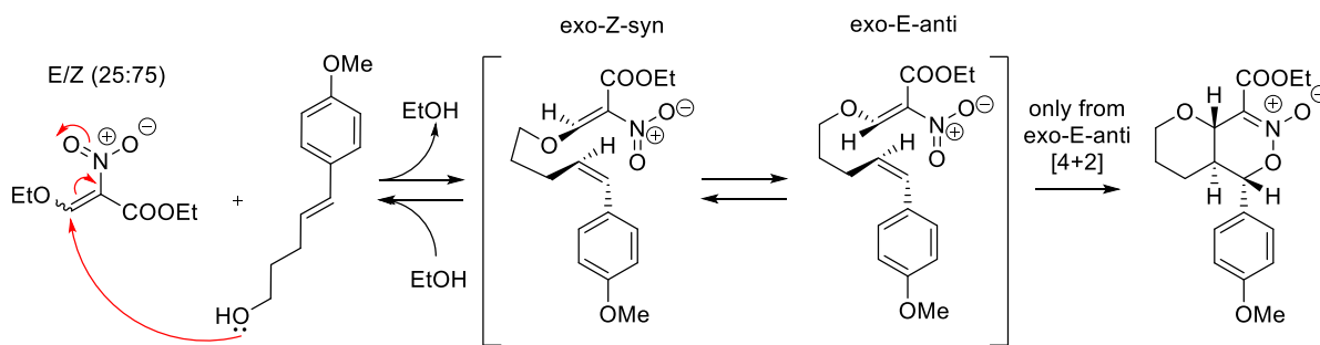
Scheme 14. Proposed reaction pathway for pericyclic reaction J2.
