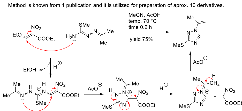
Scheme 12. The pathway and reaction of reviewed nitroalkene with 1,4-binucleophile.
