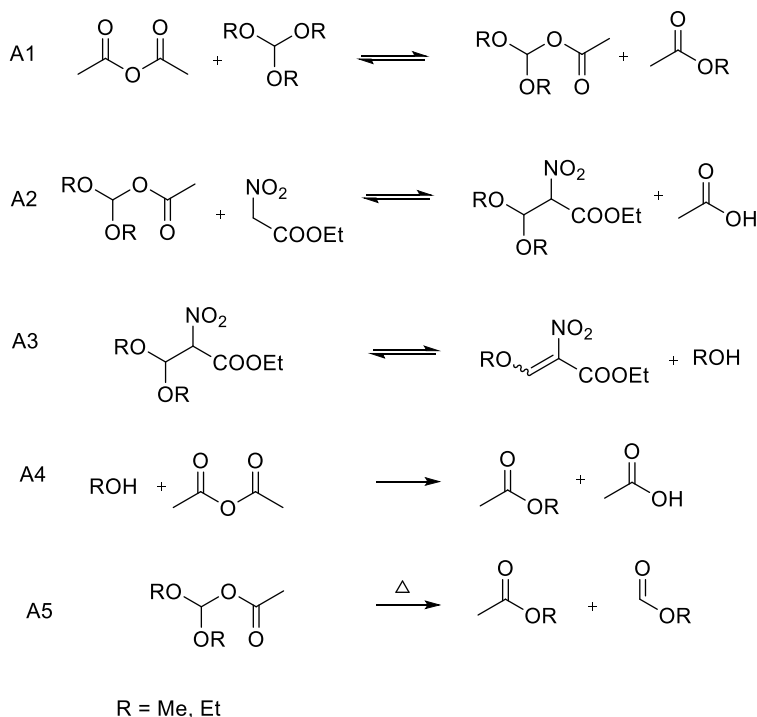
Scheme 2. Proposed mechanism of the preparation of the target nitroenoleters according to method A.
