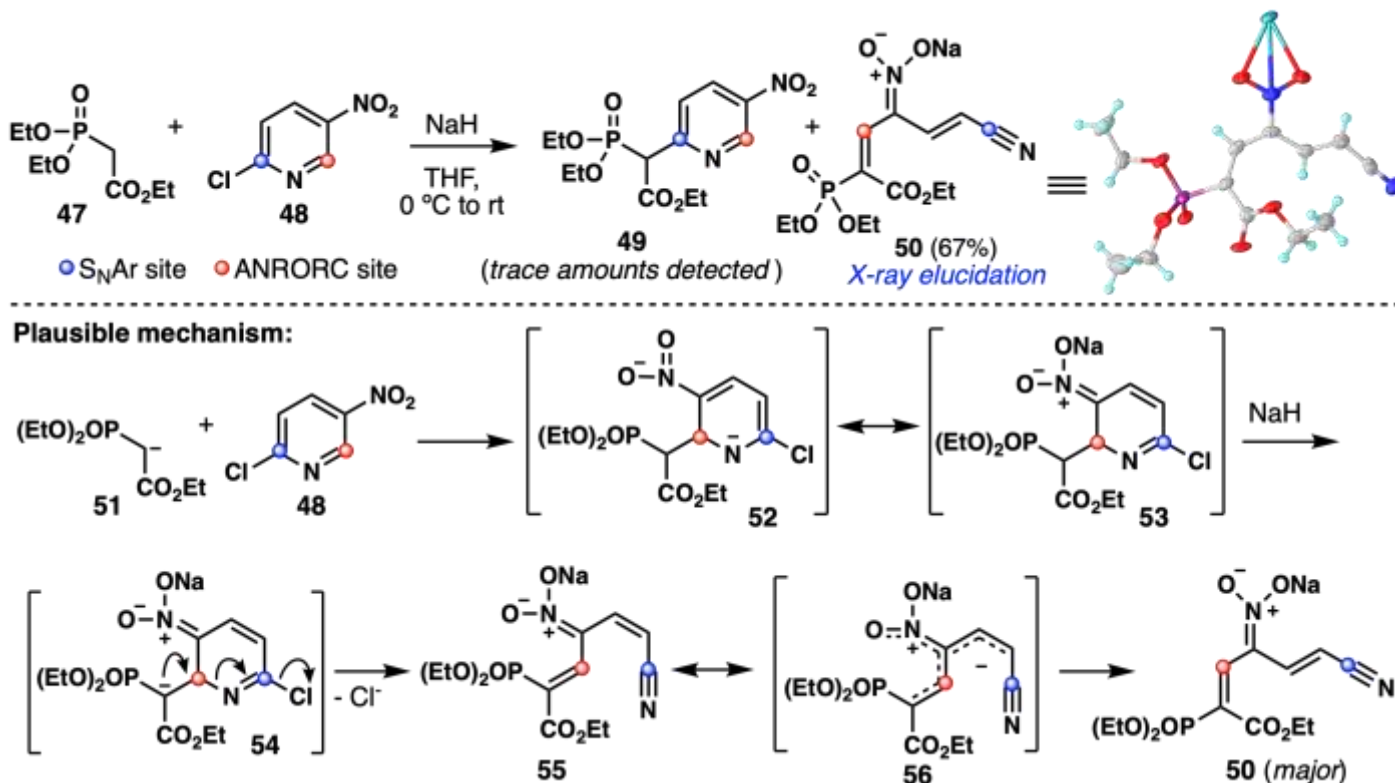
Figure 5. The reaction between anionic triethyl acetophosphonate 47 and 2-chloro-5-nitropyridine 48 via a postulated ANRORC-type mechanism.
