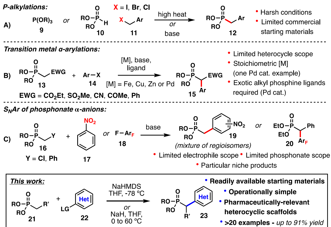
Figure 2. Classical and modern methods for preparing \alpha -arylated phosphonates compared to this work.
