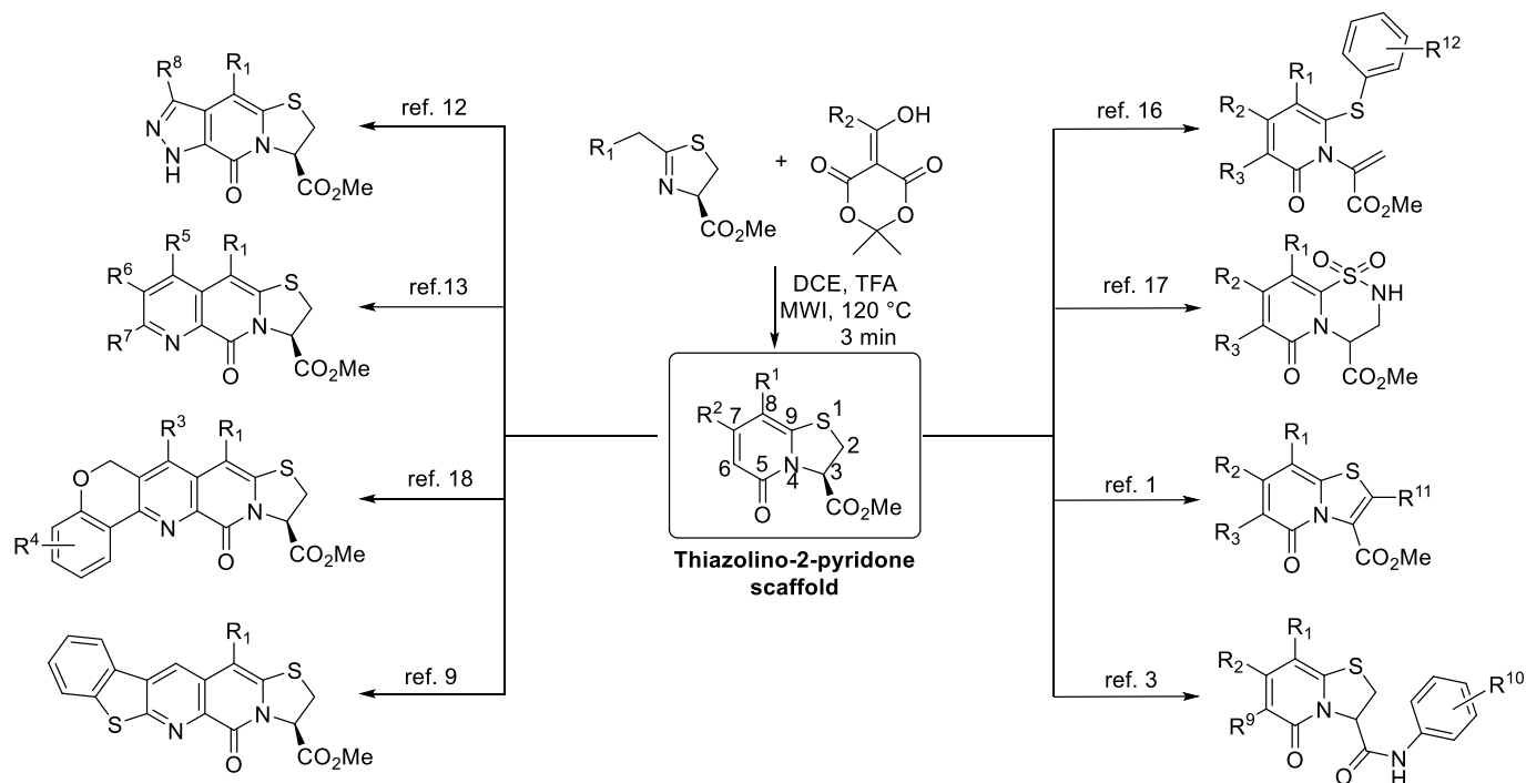
Figure 2. Synthetic applications of ring fused thiazolino-2-pyridones.
