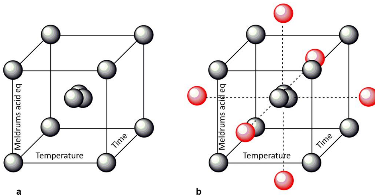
Figure 4. (a) Screening design for 2-pyridone synthesis. A full factorial design using four variables – temperature, reaction time, equivalents of Meldrum’s acid derivative, and concentration of thiazoline (not shown) – resulting in a total of 19 experiments including three central points. (b) Optimisation design for 2-pyridone synthesis. A central composite design using three variables – temperature, reaction time, and equivalents of Meldrum’s acid derivative – resulting in a total of 17 experiments including three central points.
