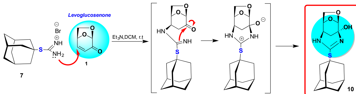
Scheme 4. Plausible reaction mechanism of conjugate addition of thiuronium via Michael addition of thiuronium “masked thiol” 7 to the conjugate system of 1 .
