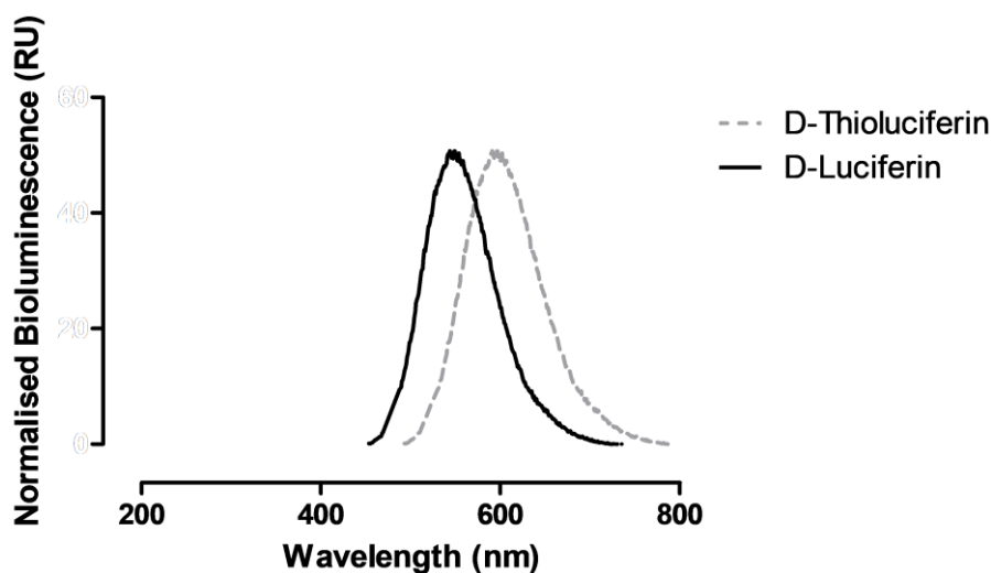
Figure. 1 Normalised bioluminescence emission spectra of 100 \mu\text{M} D-luciferin and 100 \mu\text{M} D-thioluciferin treated with 10 nM luciferase.
