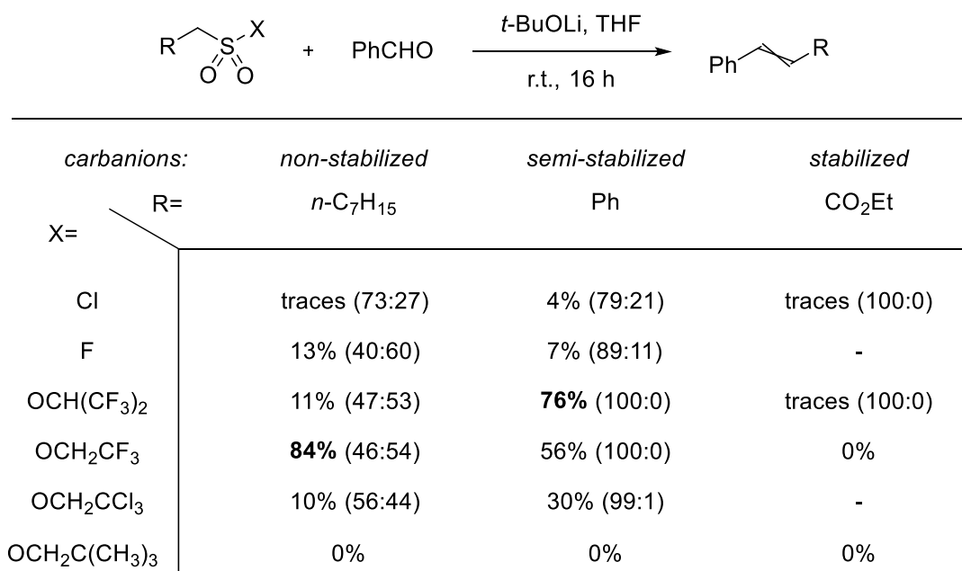
Scheme 9. Alkenes obtained using different types of carbanion precursors ( E/Z ratio was given in parentheses, only selected cases were shown). 17
