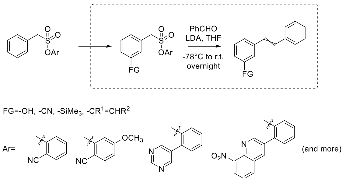
Scheme 16. General synthetic scheme described by Maiti. 23-28
