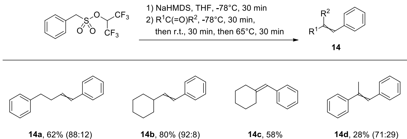
Scheme 12. Synthesis of alkenes by reacting semi-stabilized alkanesulfonate with enolizable carbonyl compounds and selected examples of obtained products ( E/Z ratio was given in parentheses). 17
