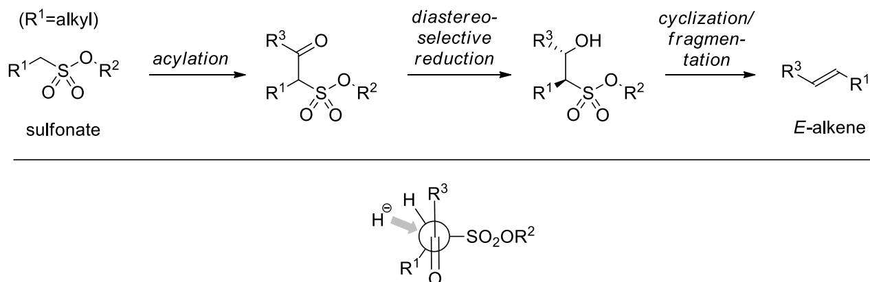
Scheme 14. Conceptual scheme for stereoselective alkene synthesis (top), and Felkin-Ahn model for the carbonyl group reduction (bottom). 19
