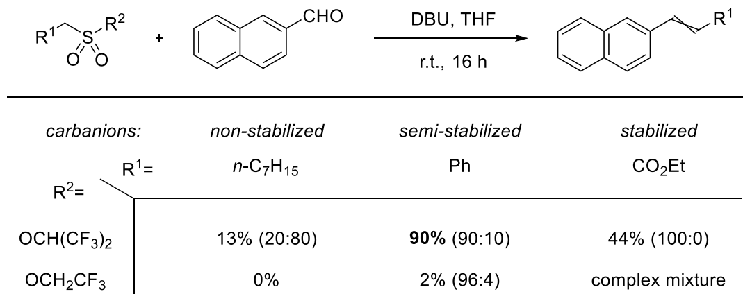
Scheme 10. Alkenes obtained using fluoroalkyl sulfonates and DBU as a base ( E/Z ratio was given in parentheses). 17,18
