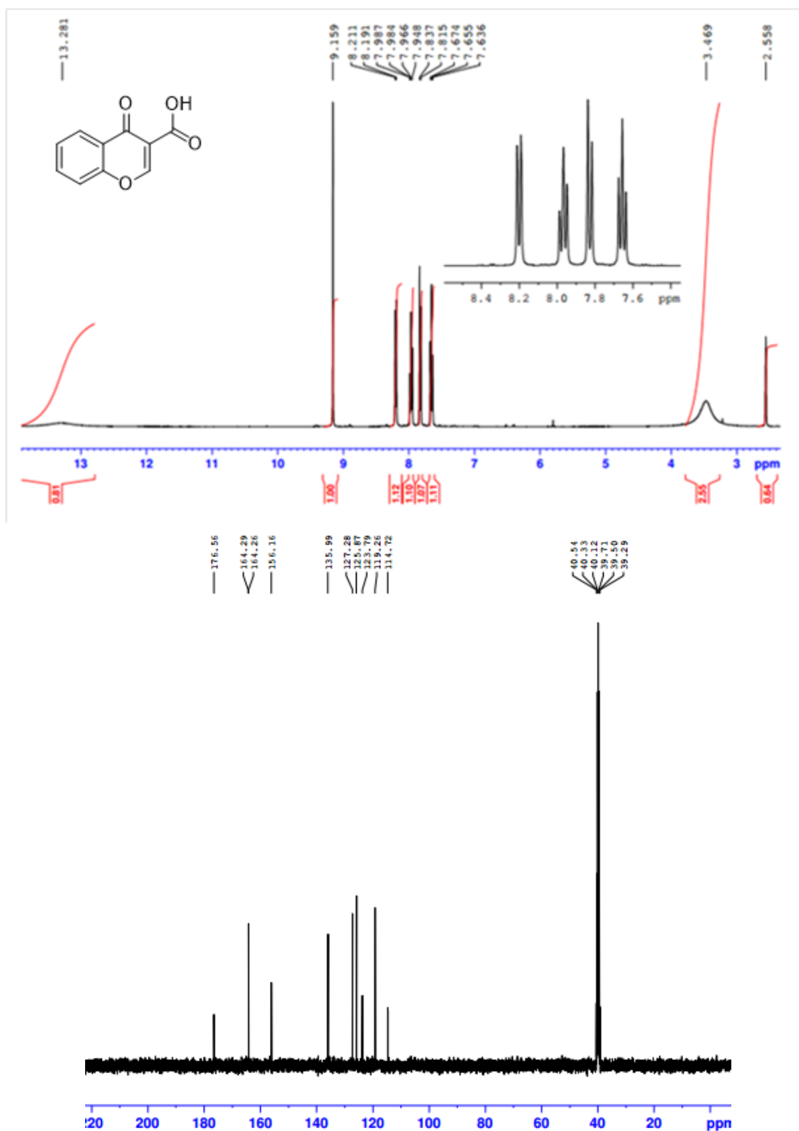
S 7: ^1\text{H} and ^{13}\text{C} spectra of 4-Oxo-4H-chromene-3-carboxylic acid 3a
