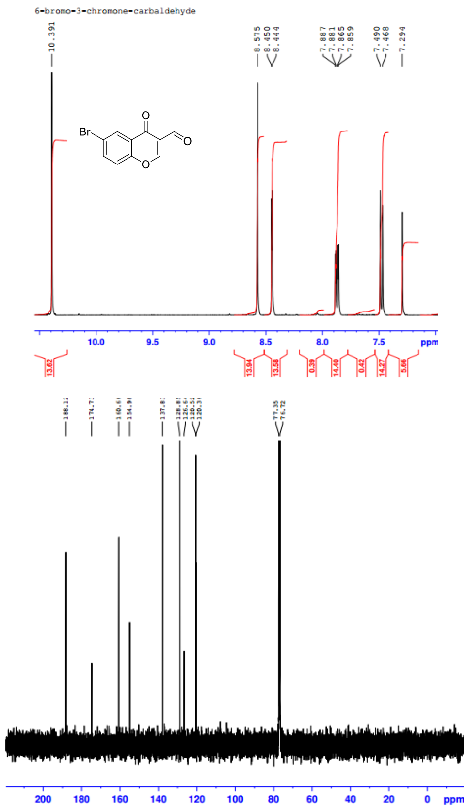
S3: 1 H and 13 C spectra of 6-Bromo-4-oxo-4H-chromene-3-carbaldehyde 2d
