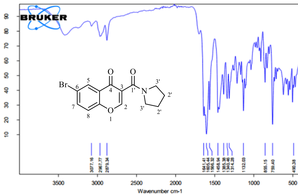
S 13: IR spectrum of 6-Bromo-3-(pyrrolidine-1-carbonyl)-4H-chromen-4-one 6d
