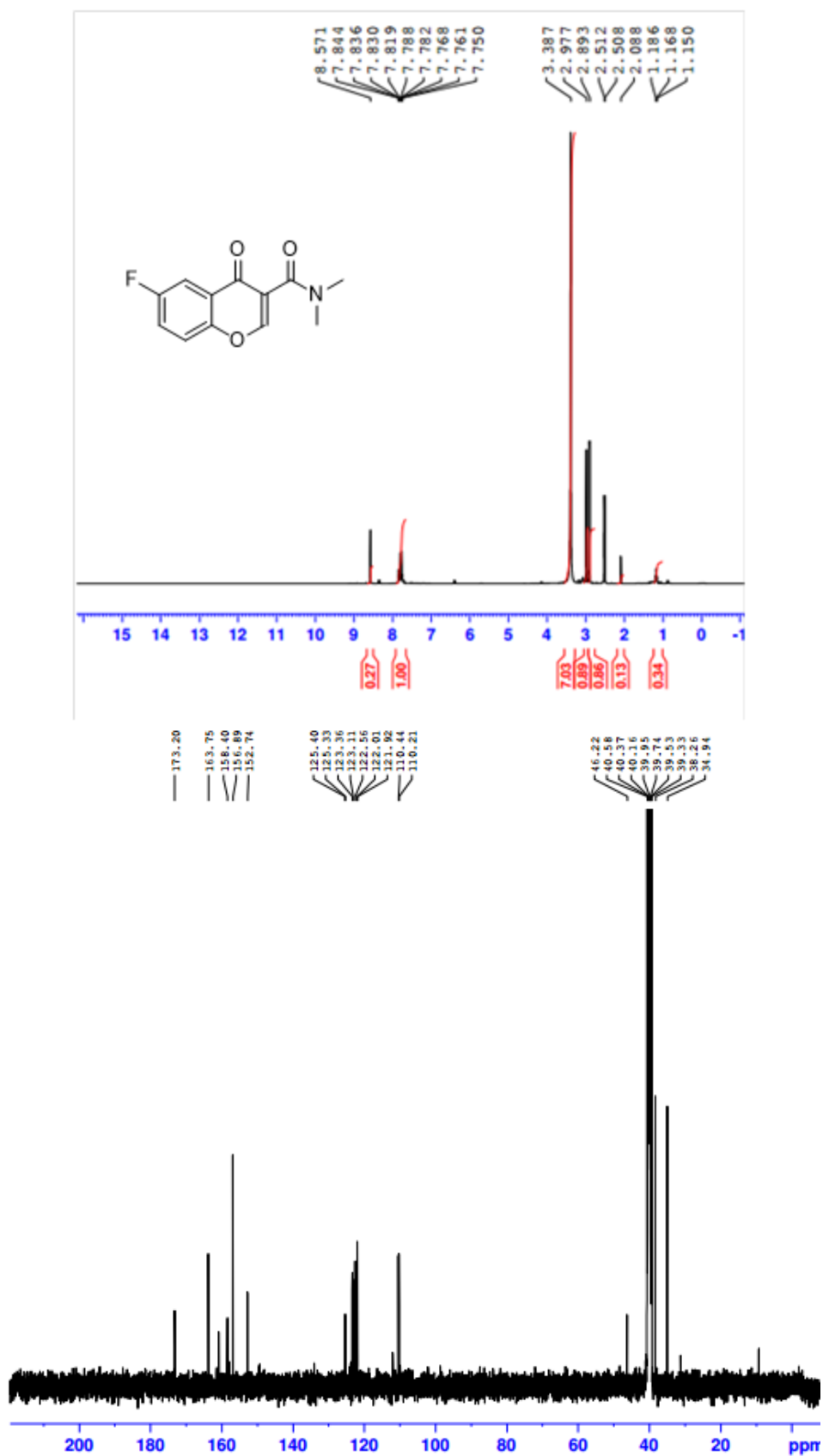
S 11: ^1\text{H} and ^{13}\text{C} spectra of N, N-dimethyl-6-fluoro-chromone-3-carboxamide 5b
