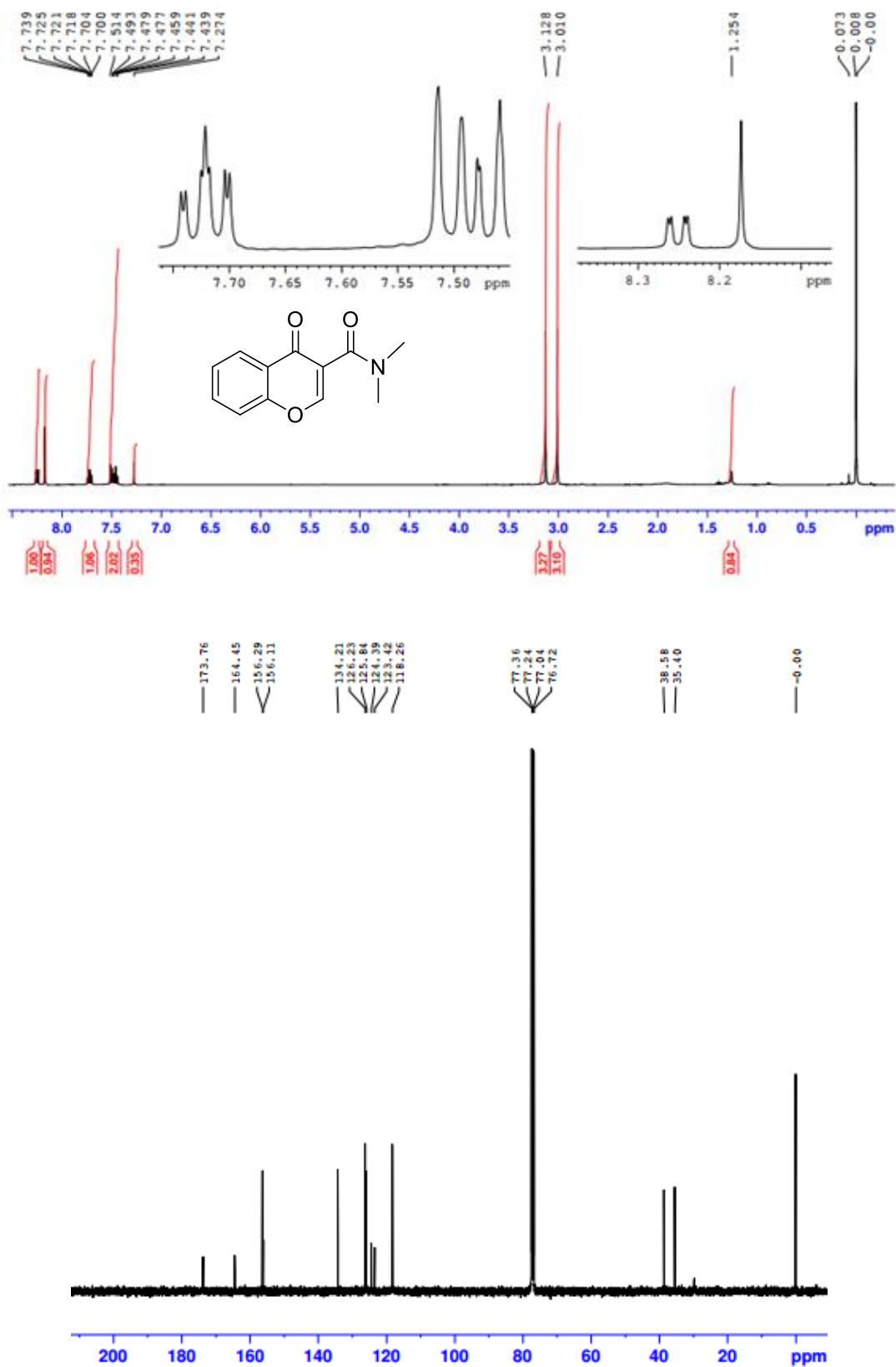
S 9: 1 H and 13 C spectra of N, N-dimethyl-4-oxo-4H-chromene-3-carboxamide 5a
