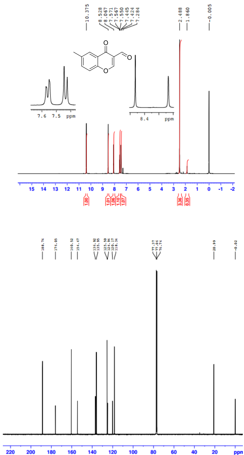
S5: 1 H and 13 C spectra of 6-Methyl-4-oxo-4H-chromene-3-carbaldehyde 2f
