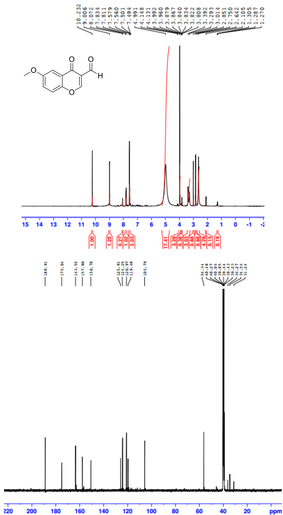
S4: 1 H and 13 C spectra of 6-Methoxy-4-oxo-4H-chromene-3-carbaldehyde 2e
