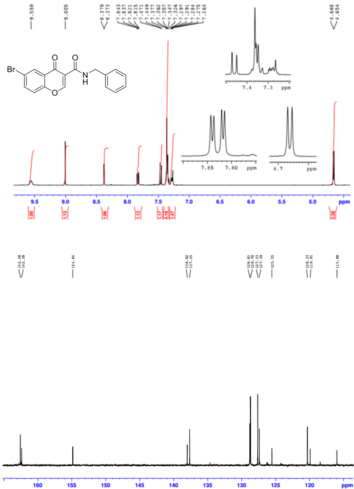
S 14: 1 H and 13 C spectra of N-benzyl-6-bromo-4-oxo-4H-chromene-3-carboxamide 8d
