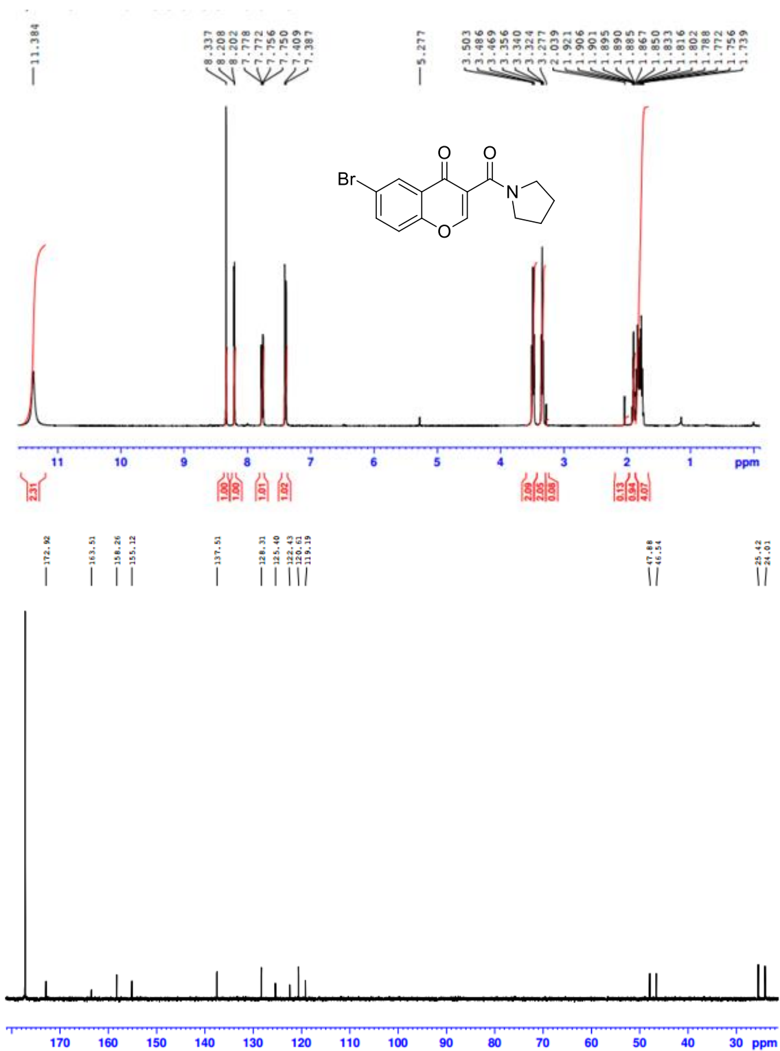
S 12: 1 H and 13 C spectra of 6-Bromo-3-(pyrrolidine-1-carbonyl)-4H-chromen-4-one 6d
