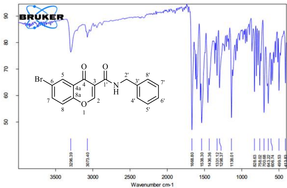
S 15: IR spectrum of N-benzyl-6-bromo-4-oxo-4H-chromene-3-carboxamide 8d
