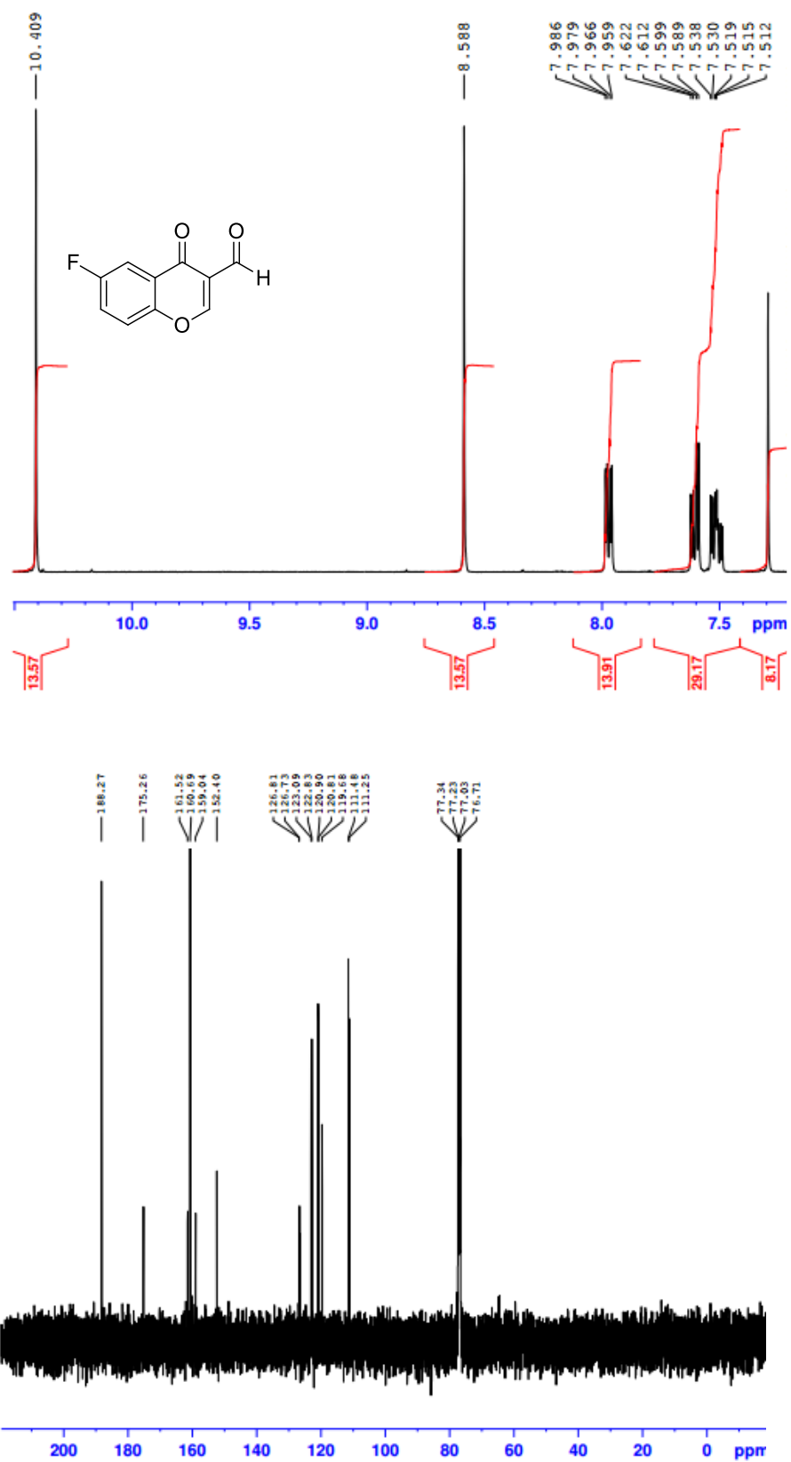
S1: ^1\text{H} and ^{13}\text{C} spectra of 6-Fluoro-4-oxo-4H-chromene-3-carbaldehyde 2b
