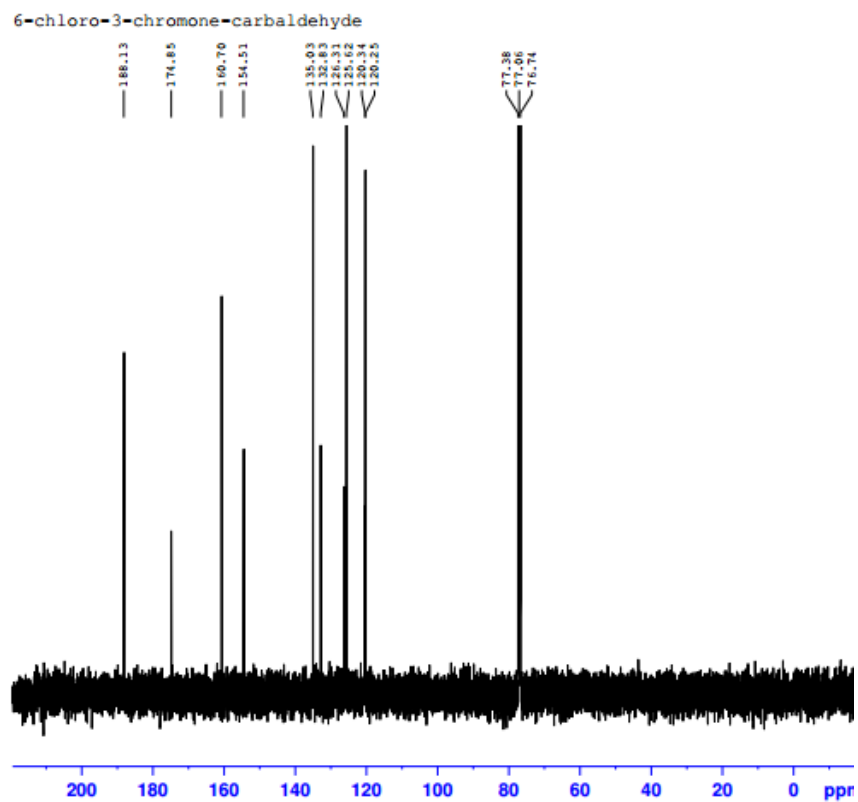
S2: ^1\text{H} and ^{13}\text{C} spectra of 6-Chloro-4-oxo-4H-chromene-3-carbaldehyde 2c
