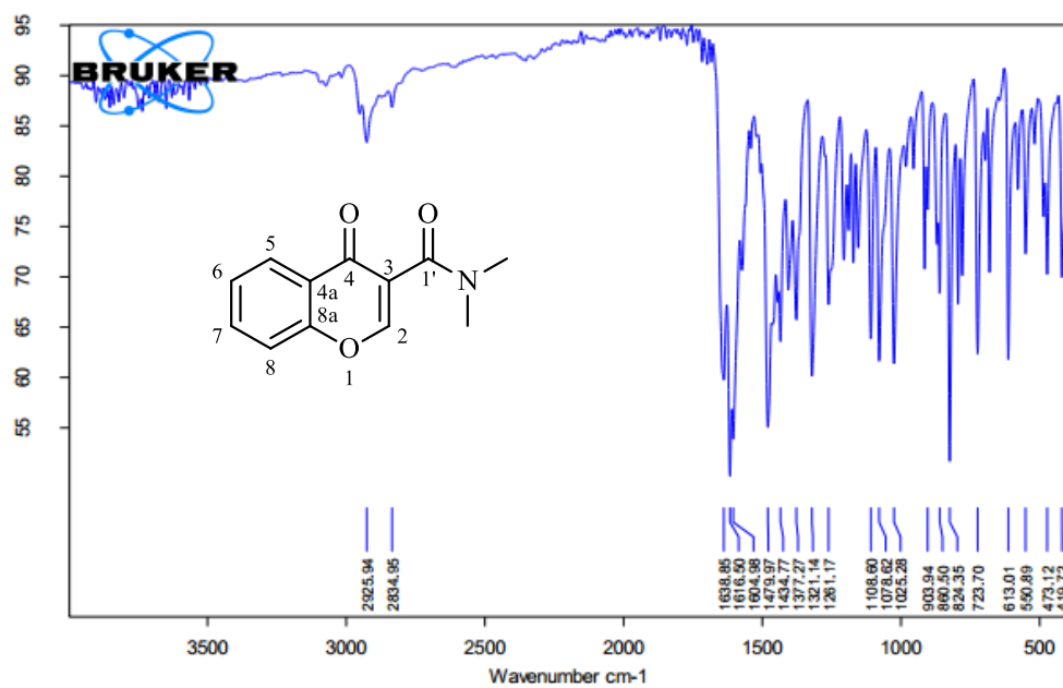
S 10: IR spectrum of N, N-dimethyl-4-oxo-4H-chromene-3-carboxamide 5a
