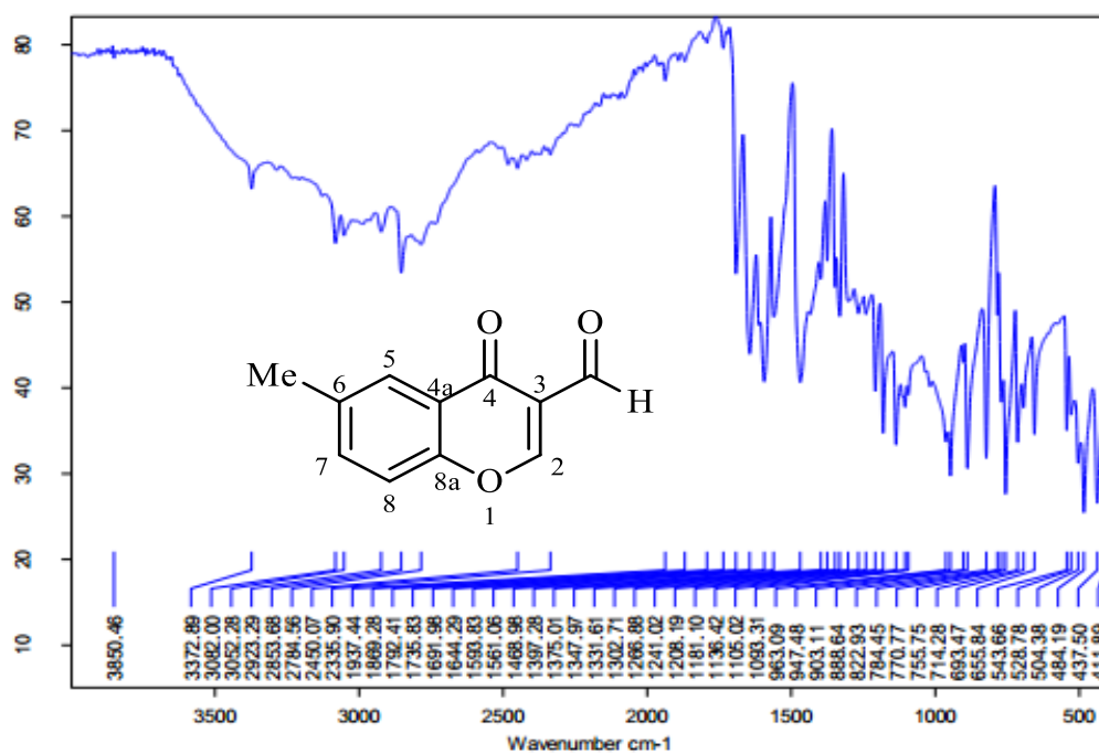
S6: IR spectrum of 6-Methyl-4-oxo-4H-chromene-3-carbaldehyde 2f
