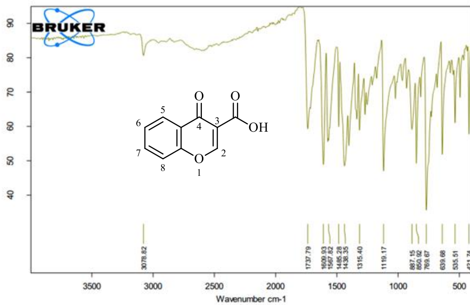
S 8: IR spectrum of 4-Oxo-4H-chromene-3-carboxylic acid 3a
