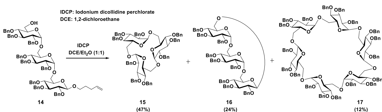
Scheme 4. Synthesis of cycloisomalto-trisaccharide 15 , 16 and -hexaoside 17 . 22
