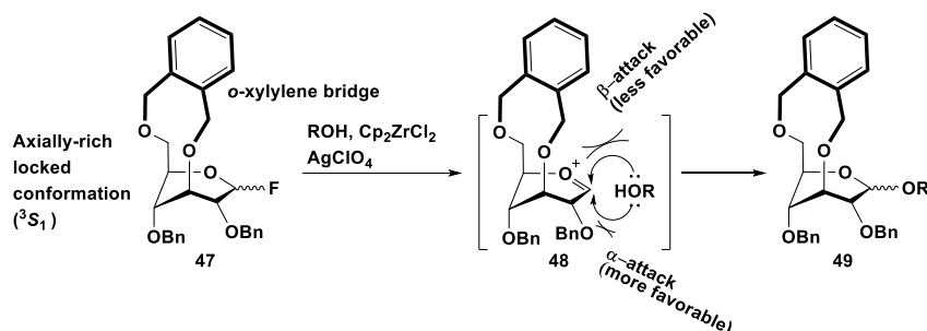
Scheme 10. Glycosylation approach involving conformationally-constrained glycosyl donor, constituted with o -xylylene bridge. 33
