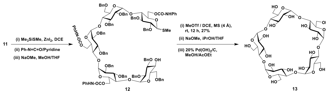
Scheme 3. Stereoselective synthesis of cyclomaltpentose. 21
