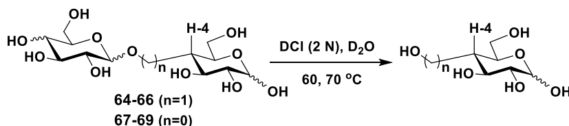
Scheme 15. Acid-catalyzed hydrolysis of disaccharides 64 – 69 . 35
