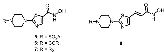
Figure 3. Thiazolyl-based hydroxamic acids HDACi 5-8 24
